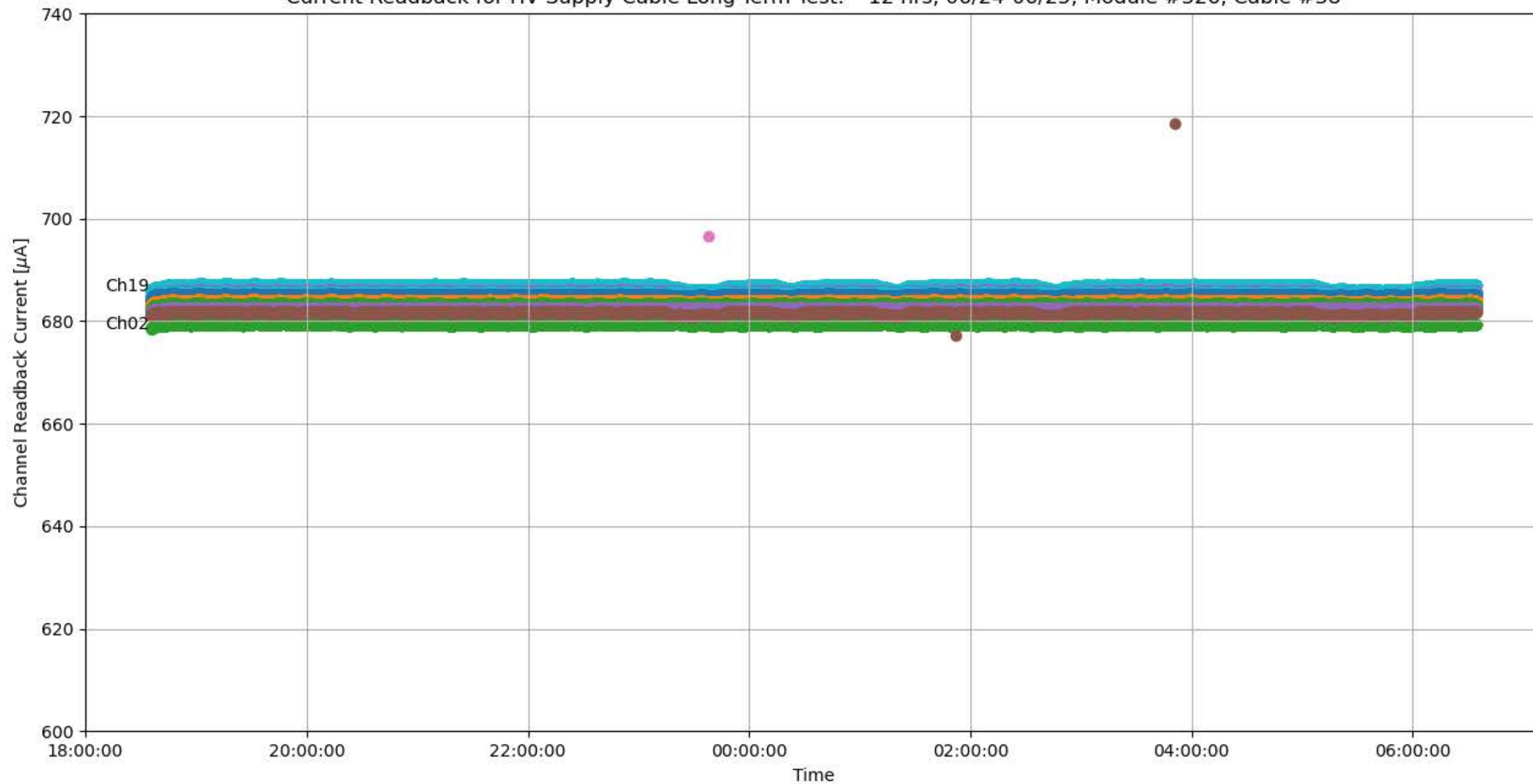
Current Readback for HV Supply Cable Long-Term Test: ~12 hrs, 06/24-06/25, Module #326, Cable #38
