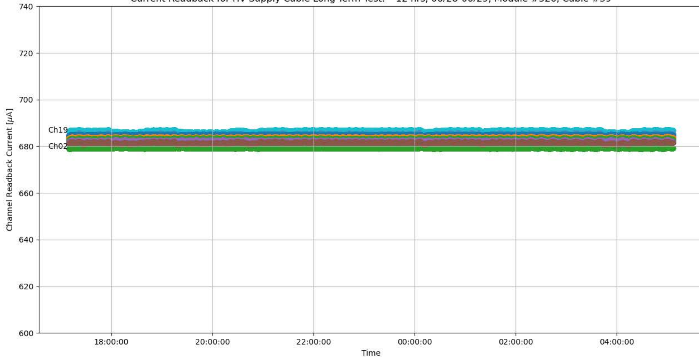
Current Readback for HV Supply Cable Long-Term Test: ~12 hrs, 06/28-06/29, Module #326, Cable #39
