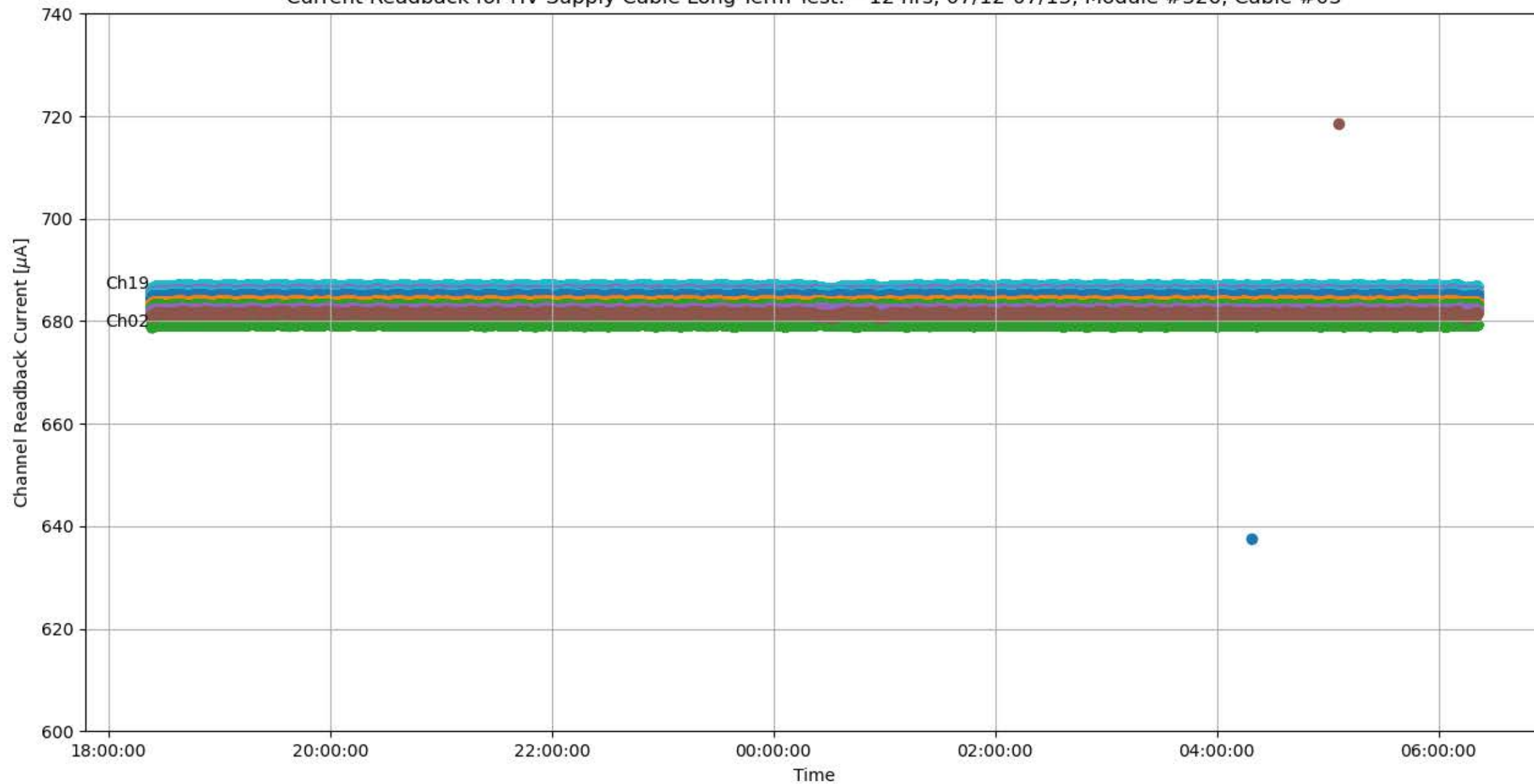
Current Readback for HV Supply Cable Long-Term Test: ~12 hrs, 07/12-07/13, Module #326, Cable #03
