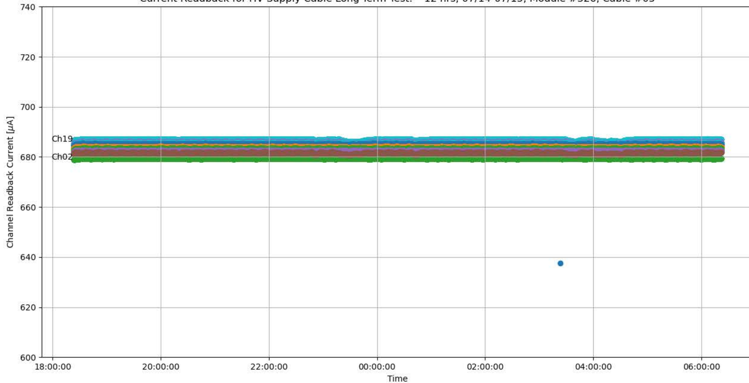
Current Readback for HV Supply Cable Long-Term Test: ~12 hrs, 07/14-07/15, Module #326, Cable #05
