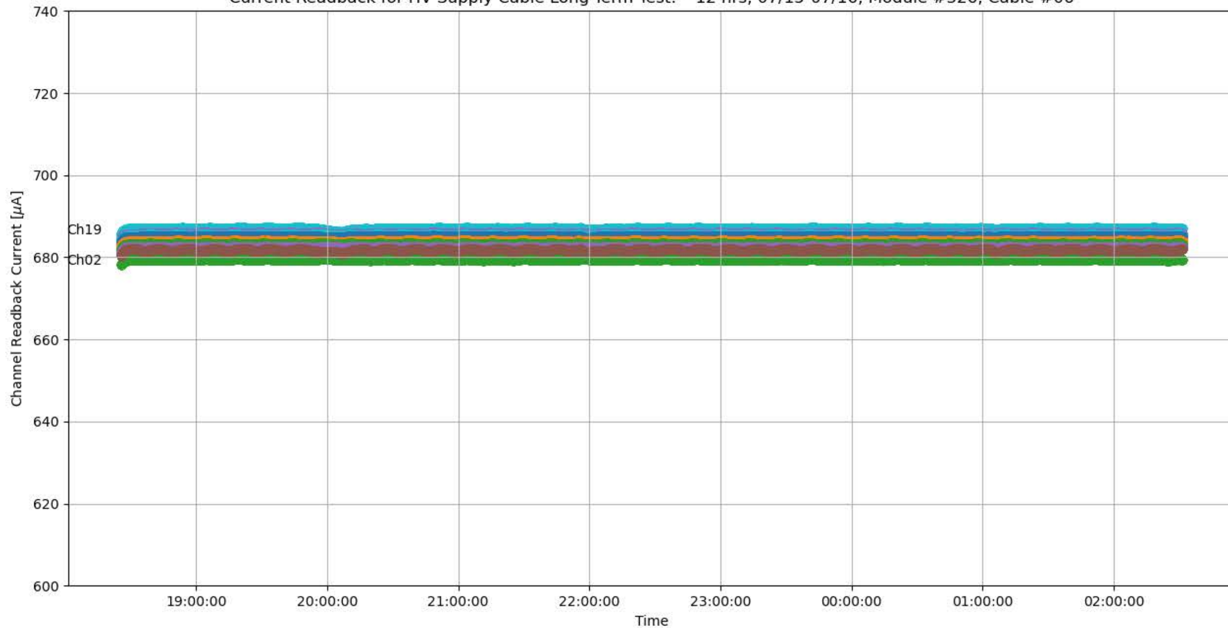
Current Readback for HV Supply Cable Long-Term Test: ~12 hrs, 07/15-07/16, Module #326, Cable #06
