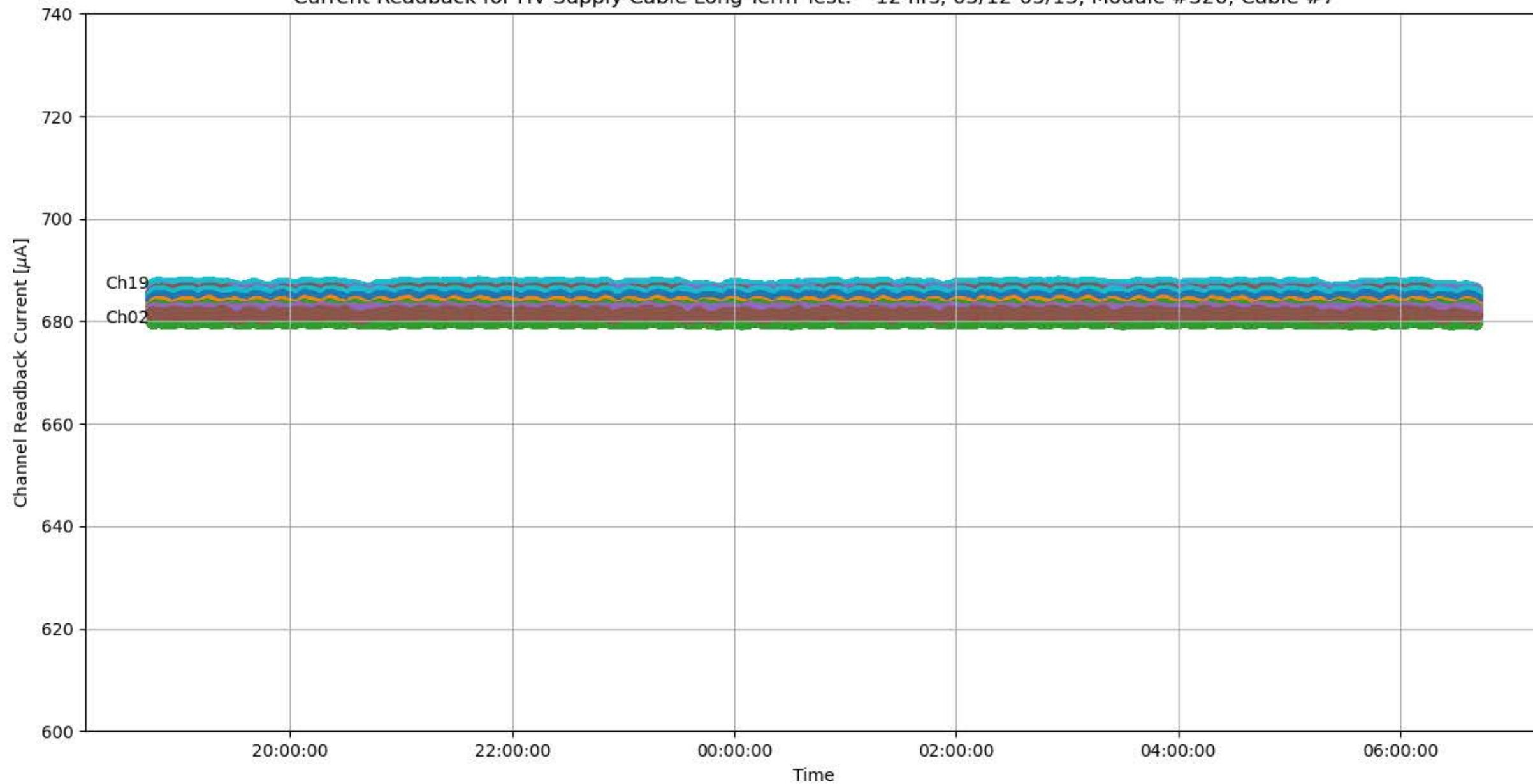
Current Readback for HV Supply Cable Long-Term Test: ~12 hrs, 05/12-05/13, Module #326, Cable #7
