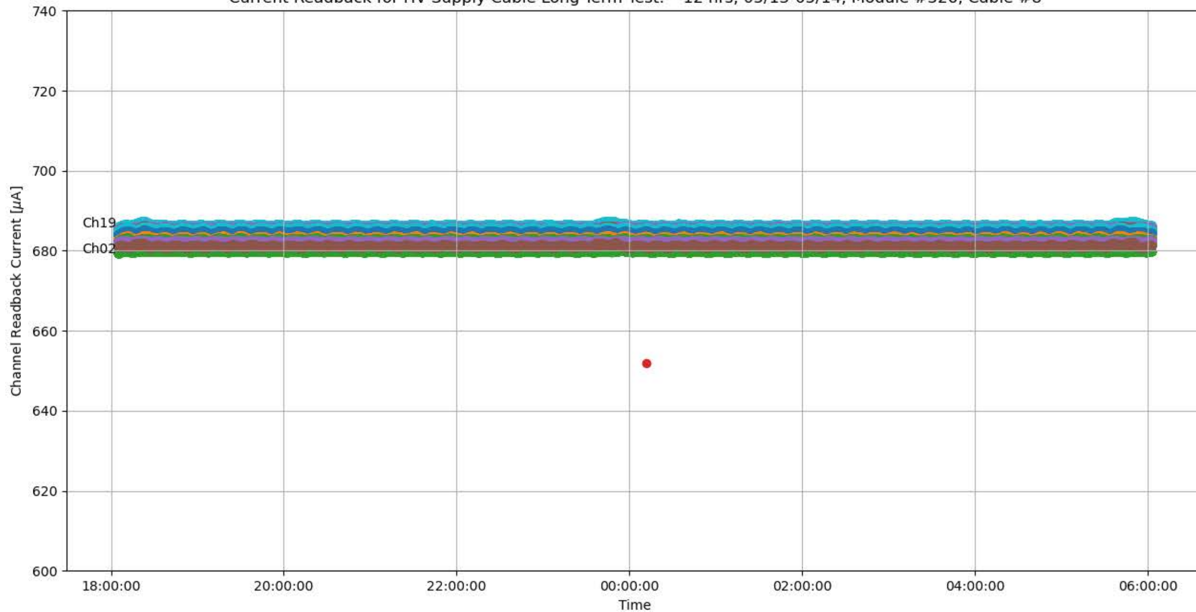
Current Readback for HV Supply Cable Long-Term Test: ~12 hrs, 05/13-05/14, Module #326, Cable #8
