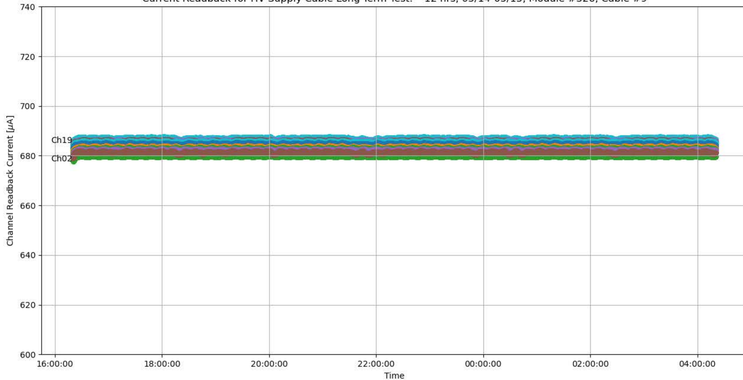
Current Readback for HV Supply Cable Long-Term Test: ~12 hrs, 05/14-05/15, Module #326, Cable #9
