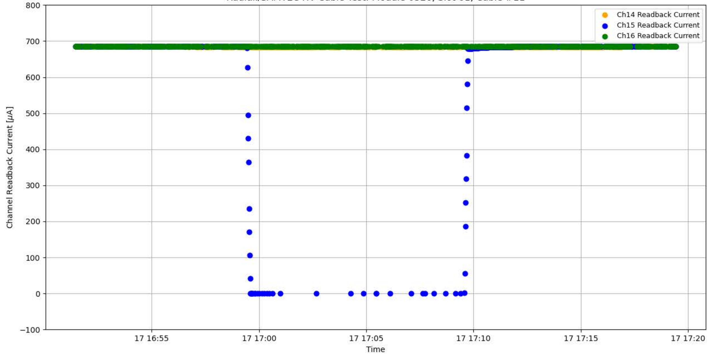
Radial/SAMTEC HV Cable Test: Module 0326, Slot 01, Cable #11
