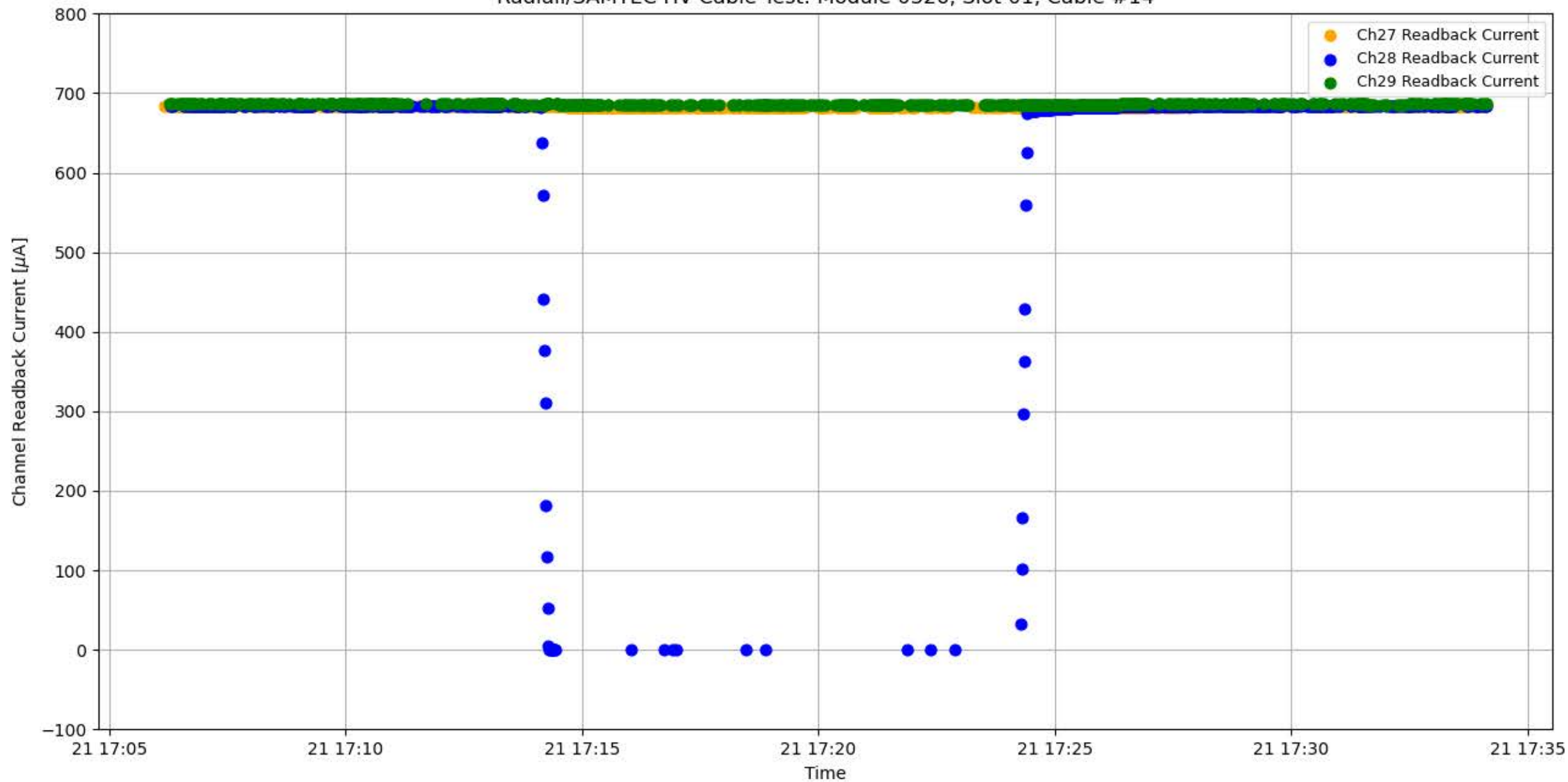
Radial/SAMTEC HV Cable Test: Module 0326, Slot 01, Cable #14
