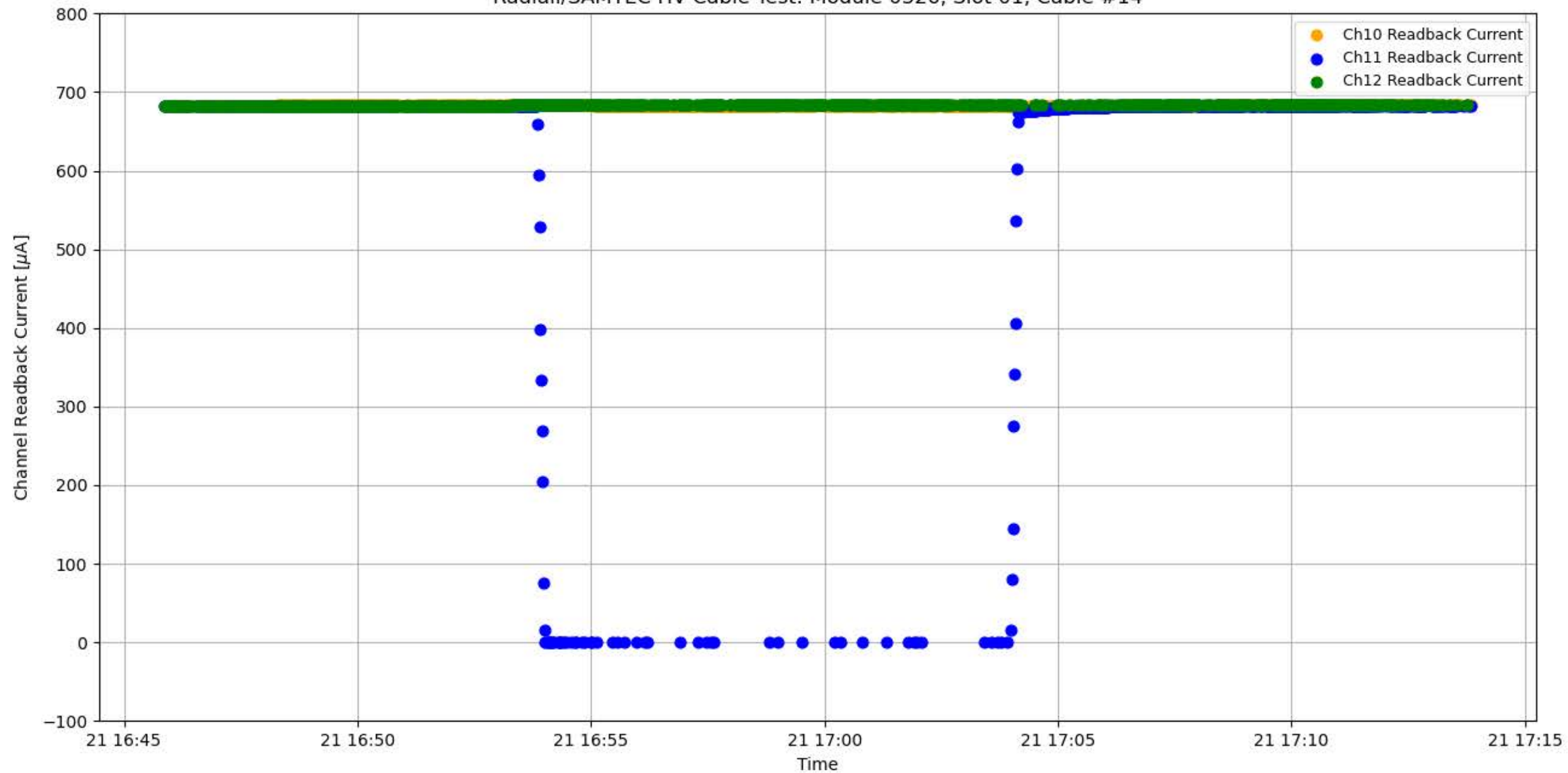
Radial/SAMTEC HV Cable Test: Module 0326, Slot 01, Cable #14
