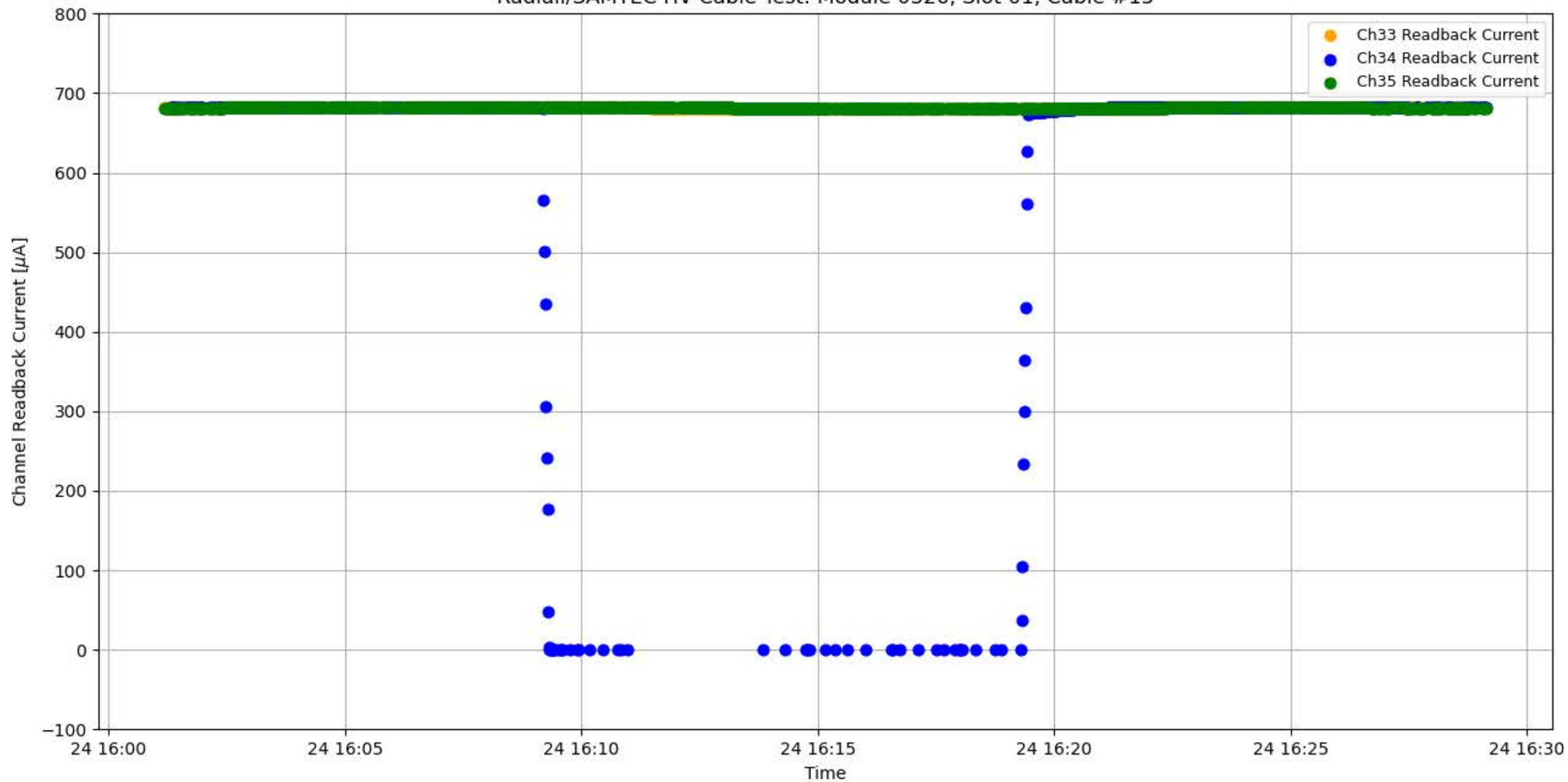
Radial/SAMTEC HV Cable Test: Module 0326, Slot 01, Cable #15
