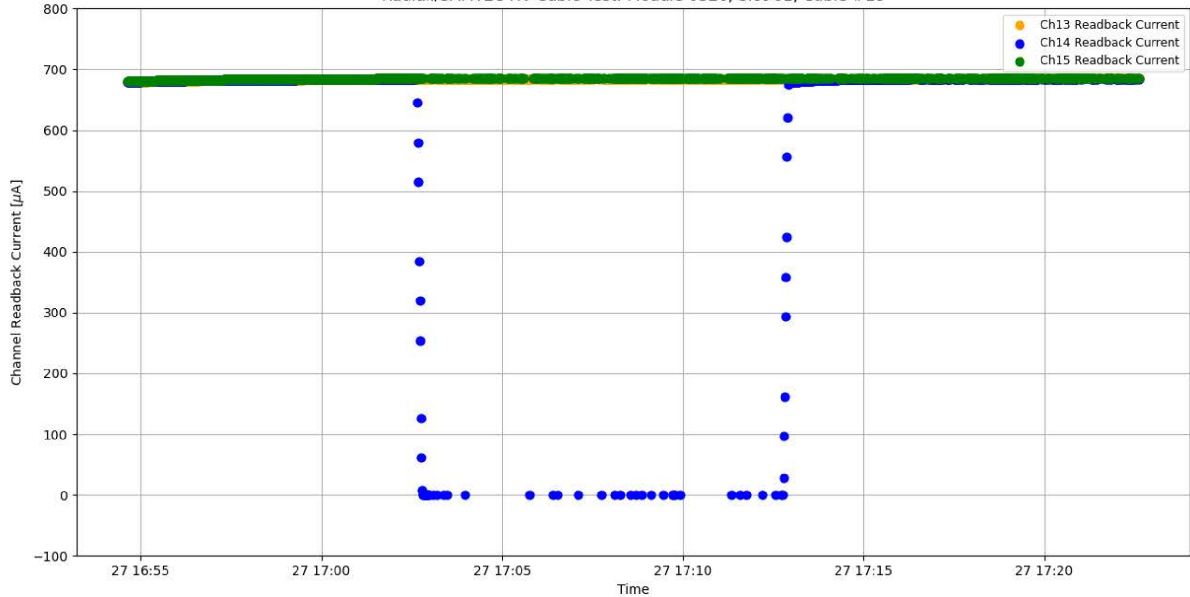
Radial/SAMTEC HV Cable Test: Module 0326, Slot 01, Cable #18
