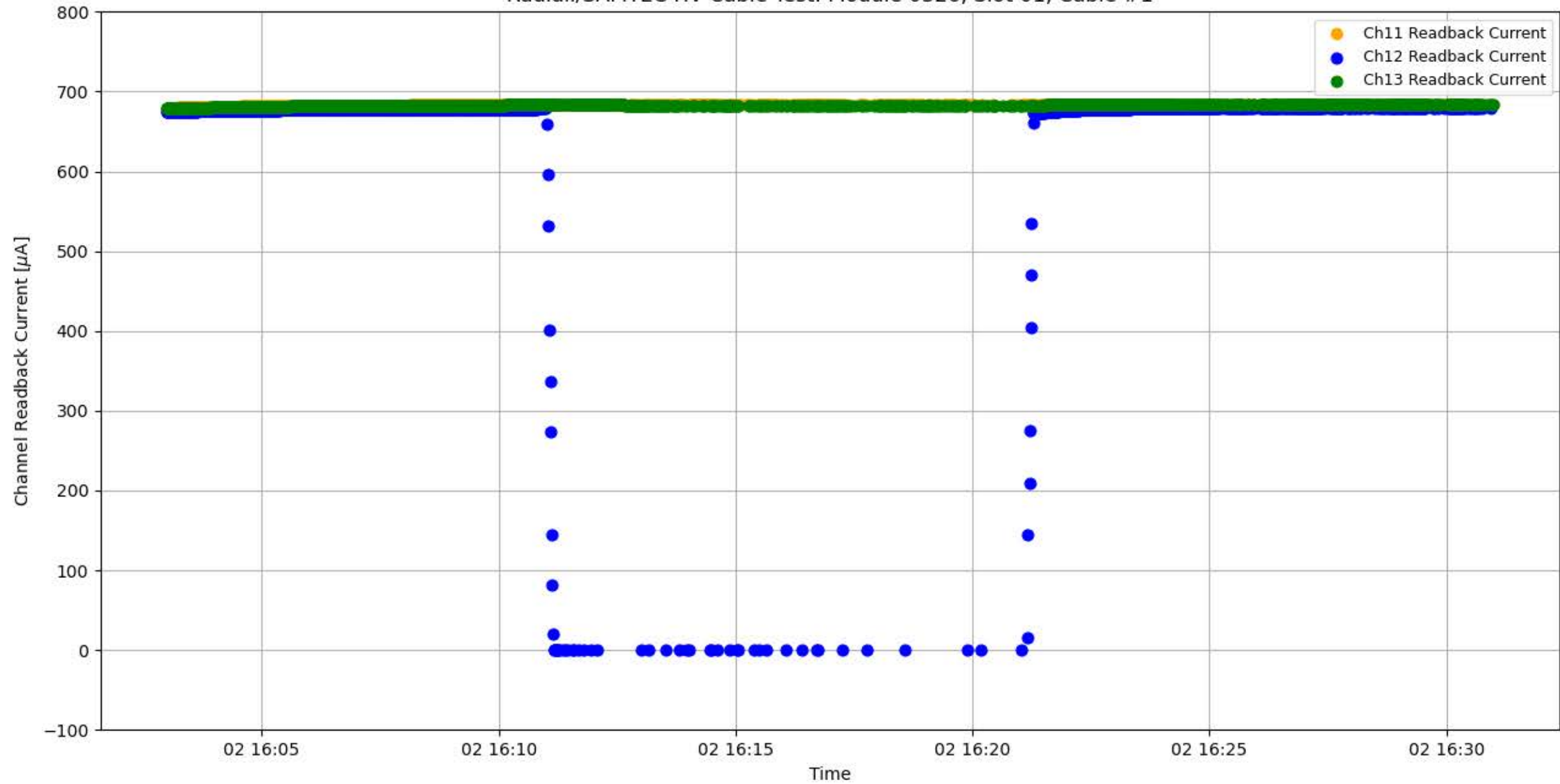
Radiall/SAMTEC HV Cable Test: Module 0326, Slot 01, Cable #1
