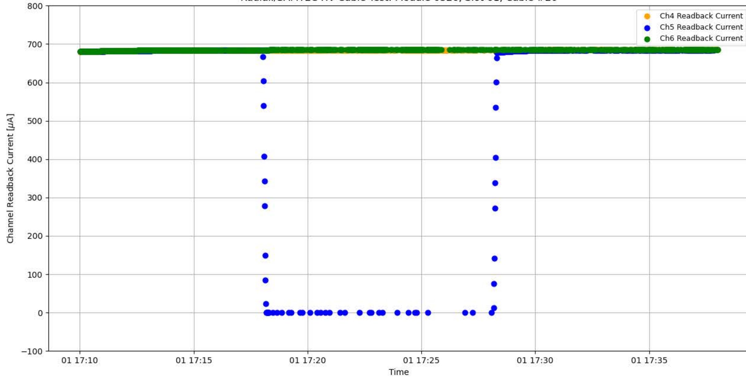
Radial/SAMTEC HV Cable Test: Module 0326, Slot 01, Cable #20
