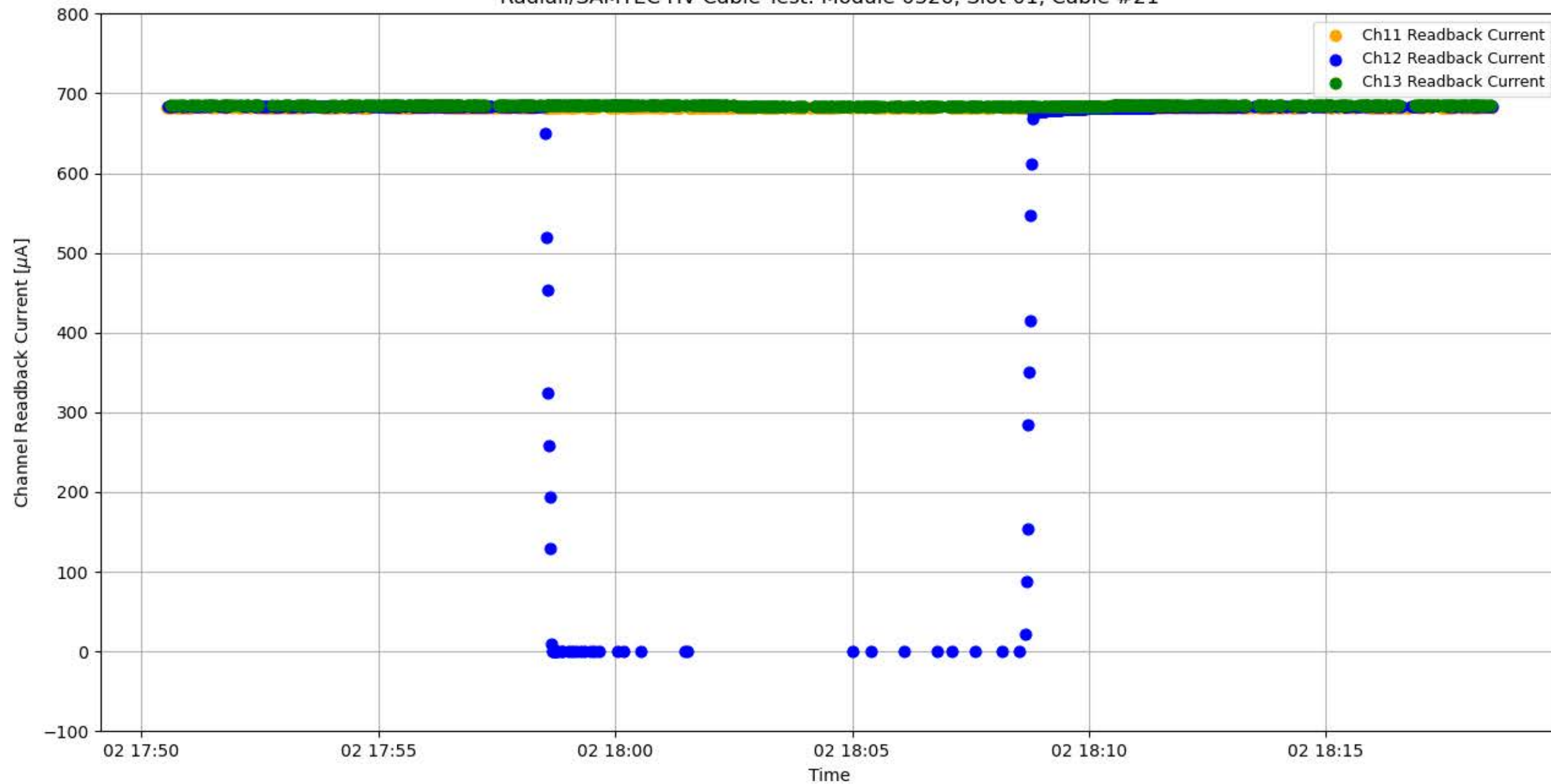
Radial/SAMTEC HV Cable Test: Module 0326, Slot 01, Cable #21
