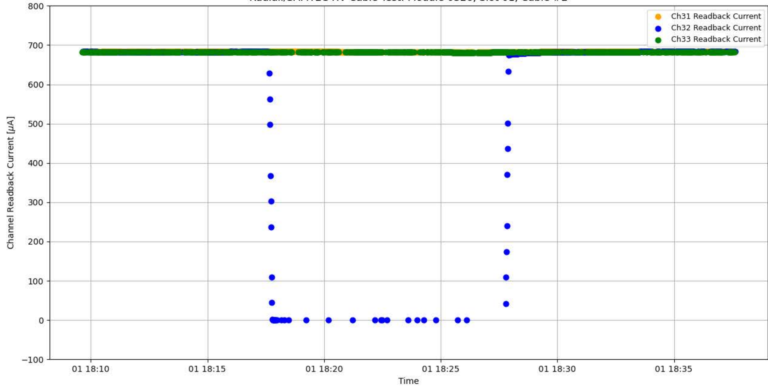
Radiall/SAMTEC HV Cable Test: Module 0326, Slot 01, Cable #2
