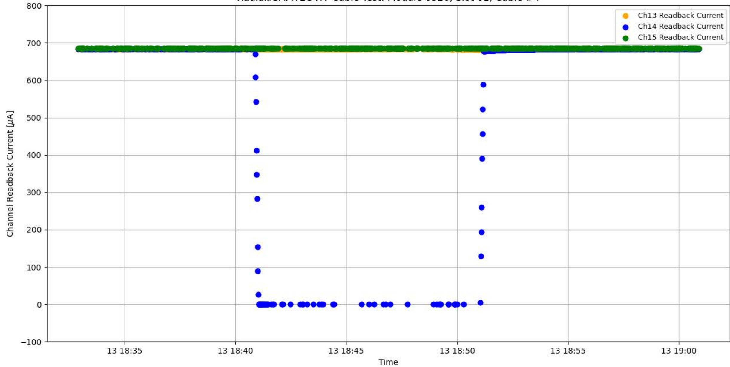
Radiall/SAMTEC HV Cable Test: Module 0326, Slot 01, Cable #4
