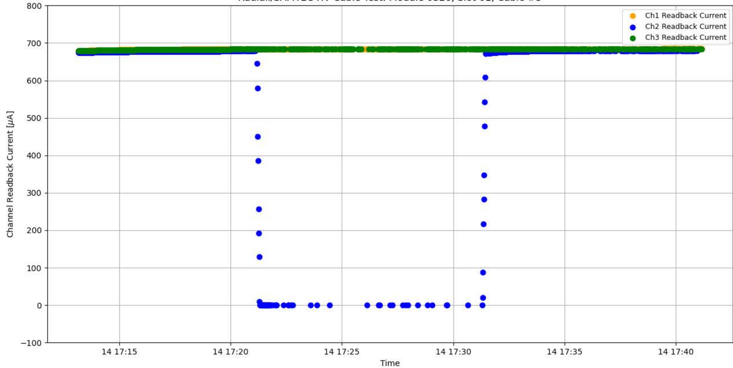
Radiall/SAMTEC HV Cable Test: Module 0326, Slot 01, Cable #5
