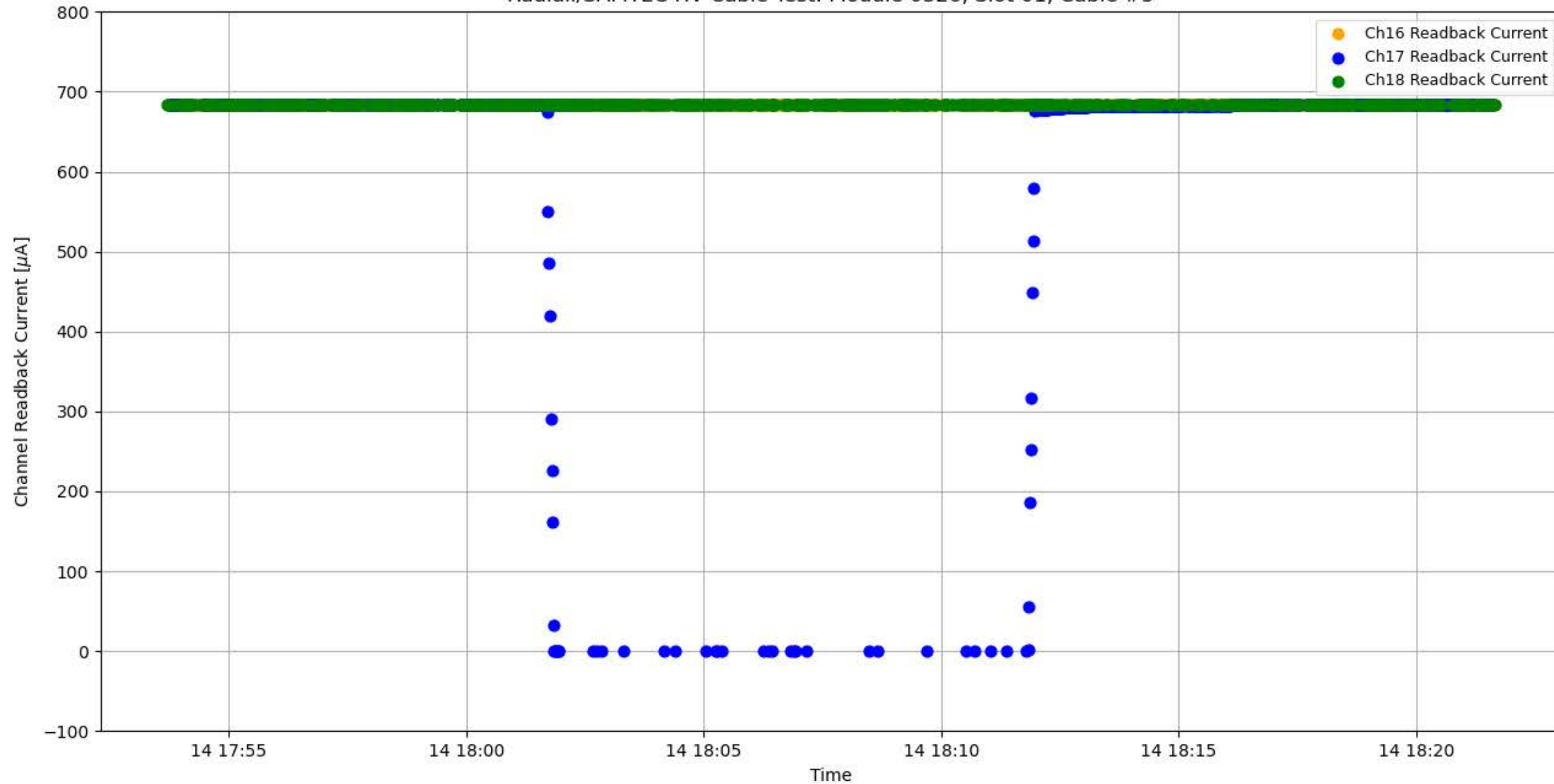
Radiall/SAMTEC HV Cable Test: Module 0326, Slot 01, Cable #5
