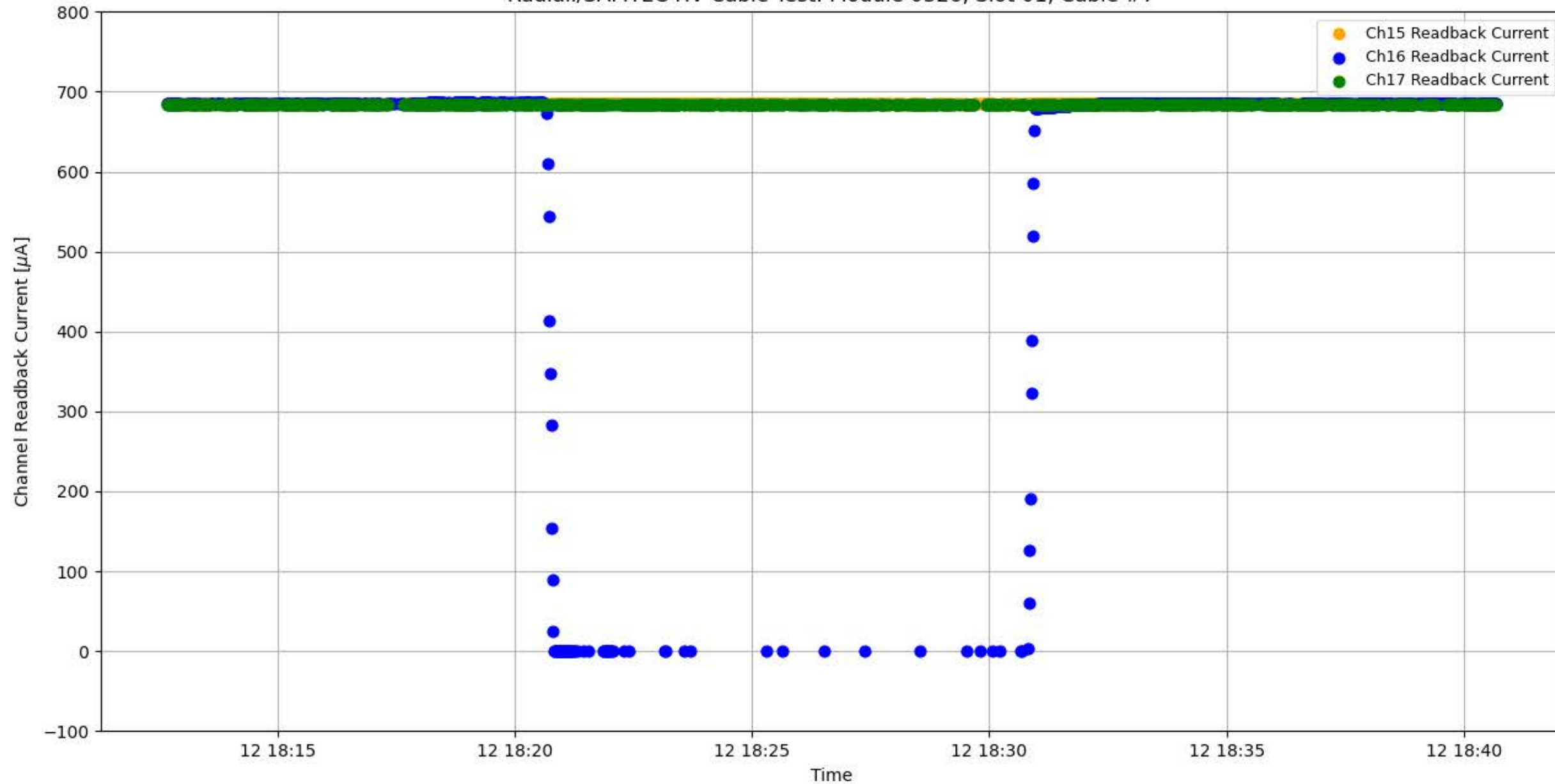
Radiall/SAMTEC HV Cable Test: Module 0326, Slot 01, Cable #7
