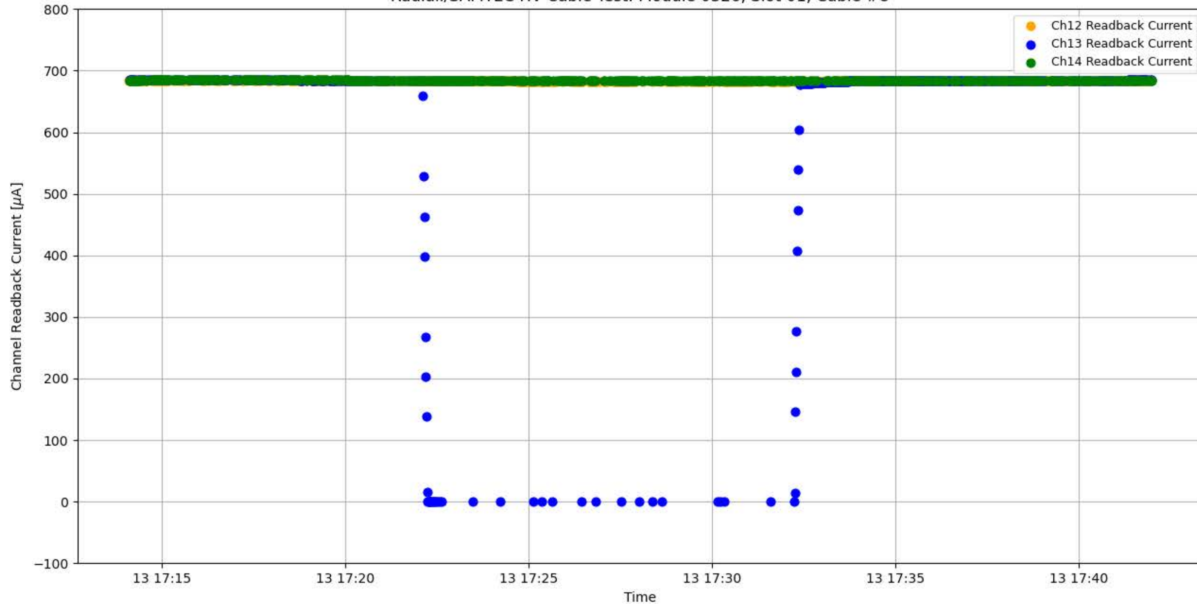
Radiall/SAMTEC HV Cable Test: Module 0326, Slot 01, Cable #8
