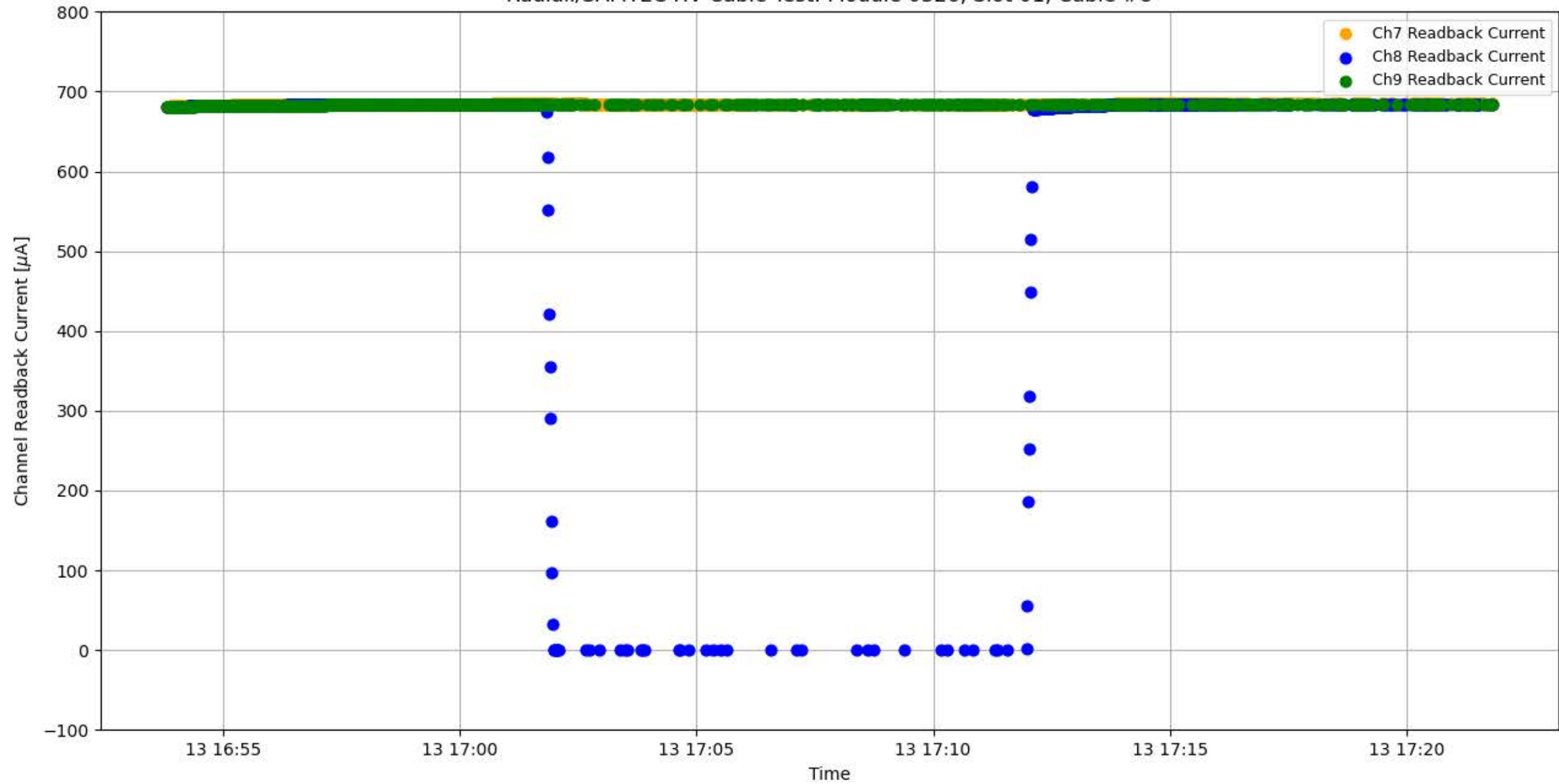
Radiall/SAMTEC HV Cable Test: Module 0326, Slot 01, Cable #8
