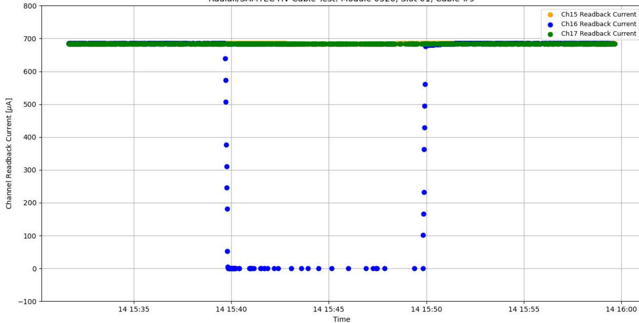
Radiall/SAMTEC HV Cable Test: Module 0326, Slot 01, Cable #9
