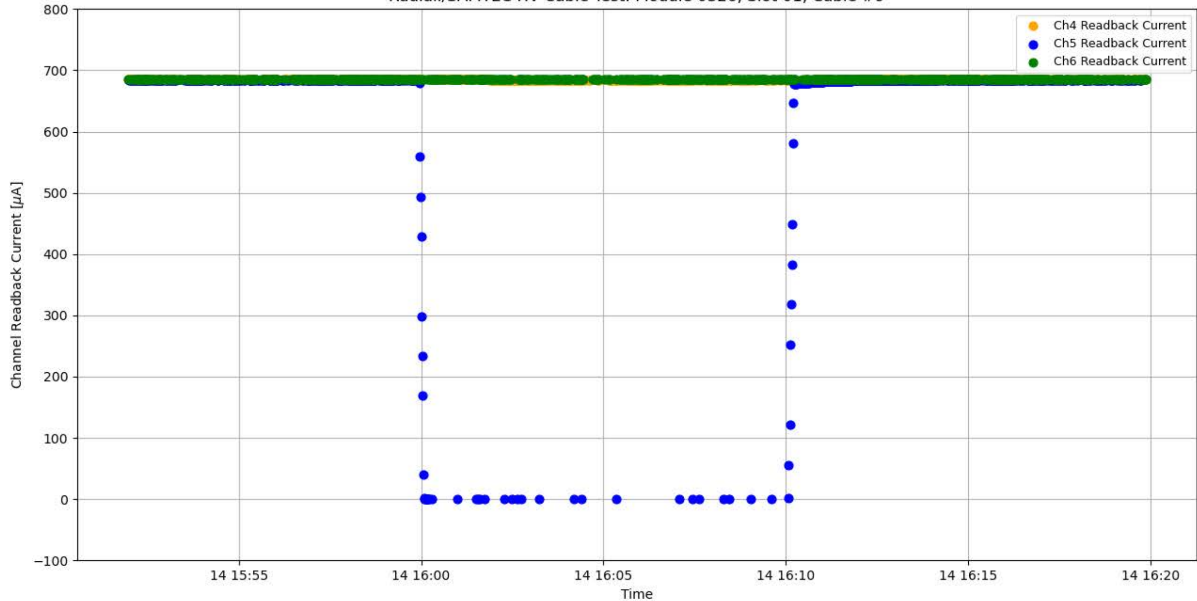
Radiall/SAMTEC HV Cable Test: Module 0326, Slot 01, Cable #9
