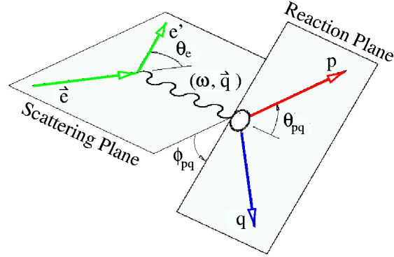
Figure 5: Kinematics of D(e, e'p)n and D(e, e'n)p .
