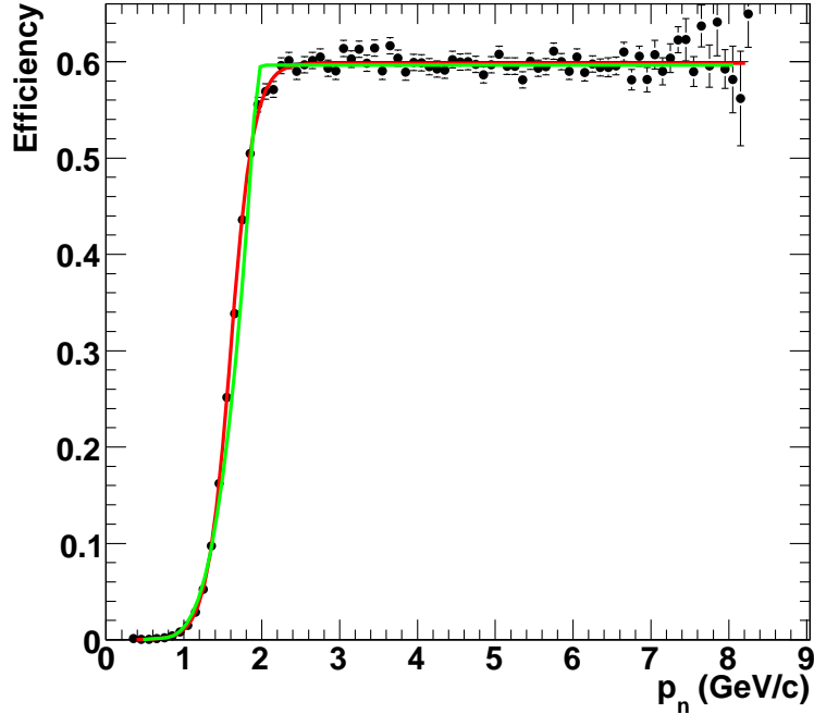
Figure 25: Monte Carlo simulation of the neutron detection efficiency along with two fits to the simulated data. The red curve is a fit to the simulated neutron detection curve using Equation 19; the green curve is a third-order polynomial at low p_n and has a constant value at high p_n . The boundary between the two parts of the green curve is varied to find the best fit.
