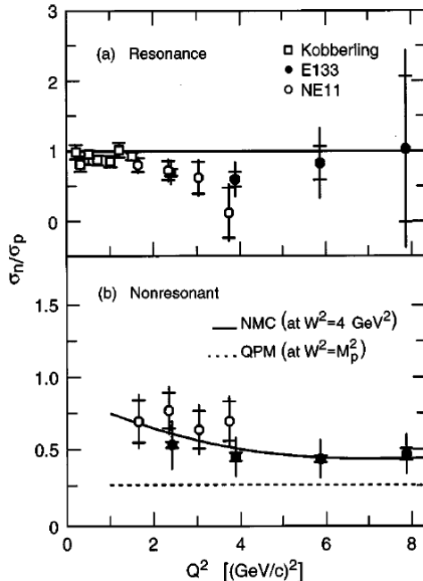
Figure 10: The ratios (a) (\sigma_n/\sigma_p)_\Delta and (b) (\sigma_n/\sigma_p)_{nonres} for inelastic electron scattering from deuterium from Reference [28].
