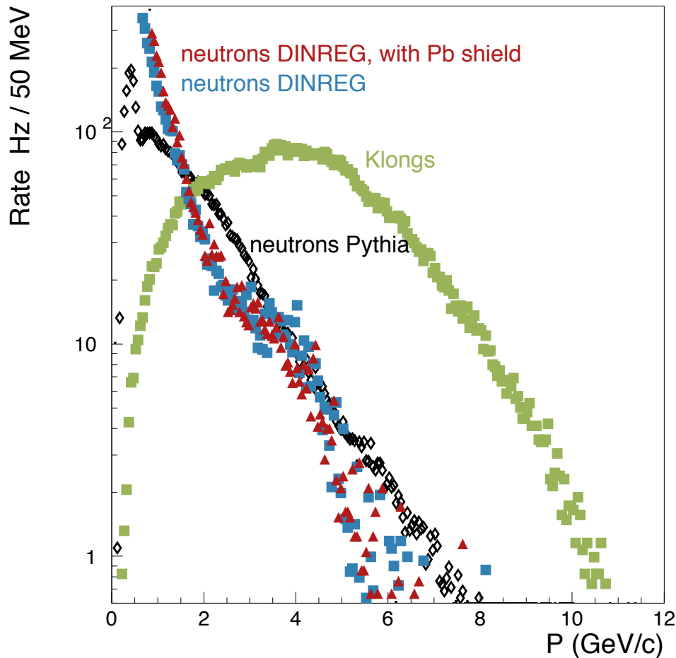
FIG. 2: The rate of neutrons (open symbols) and K_L^0 (full squares) on LH_2 target of Hall D as a function of their momenta simulated with different MC generators with 10^4 K_L^0/\text{sec} .
