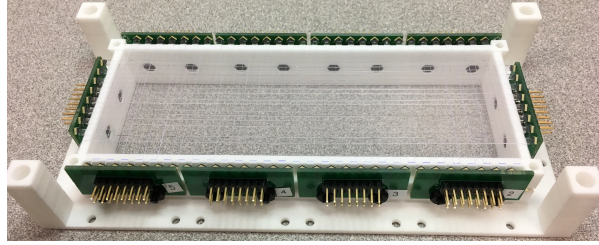
FIG. 17. The scintillating tile focal-plane detector, prior to being enclosed and installed.
