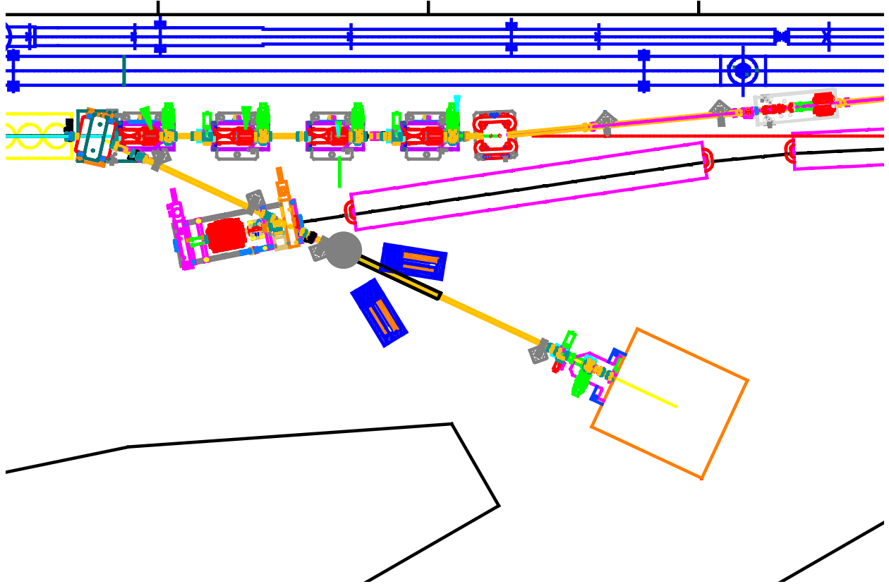
FIG. 3. Overhead view of the relevant beam line segment including spectrometer magnets, target chamber and beam dump. Drawn is a positioning most upstream, to maximize space between wall and spectrometer and distance to beam dump. A shift to a more downstream position is possible if the upstream clearance needs to be increased. (Note: The magnet yoke overhangs the beam pipe and creates an apparent interference in this projection which is not real.)
