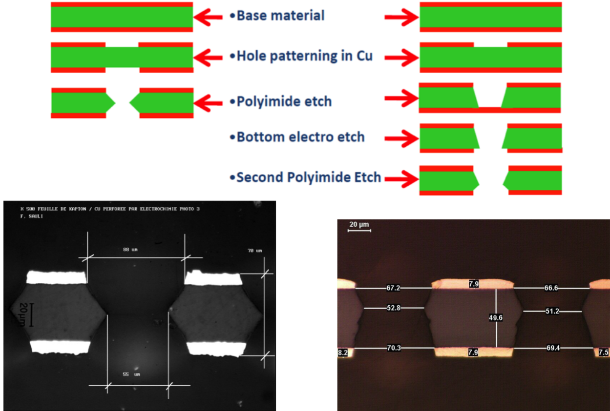
FIG. 5. Left: Double-mask etching technique. Right: Single-mask technique.
