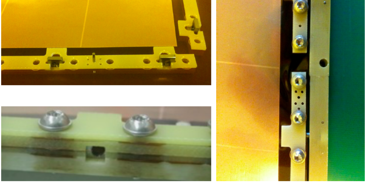
FIG. 6. Photographs of the CMS NS2 frames at CERN. Upper left: single layer of the inner frame showing a groove with an embedded nut to hold the stretching screw. Lower left: Bolted inner frame stack to clamp all layers, showing the hole with the embedded nut for the stretching screw. Right: Inner frame stack with horizontal screws through the outer frame for stretching. The gap between inner and outer frame is a few mm to accommodate the tension.
