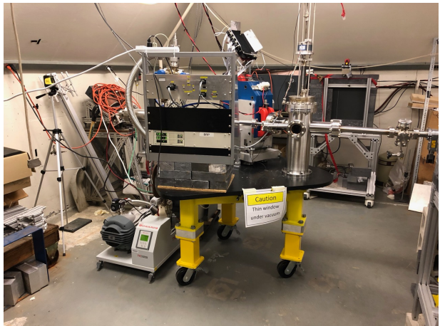
FIG. 19. The radiative Møller experiment being commissioned at the HVRL in February 2018.
