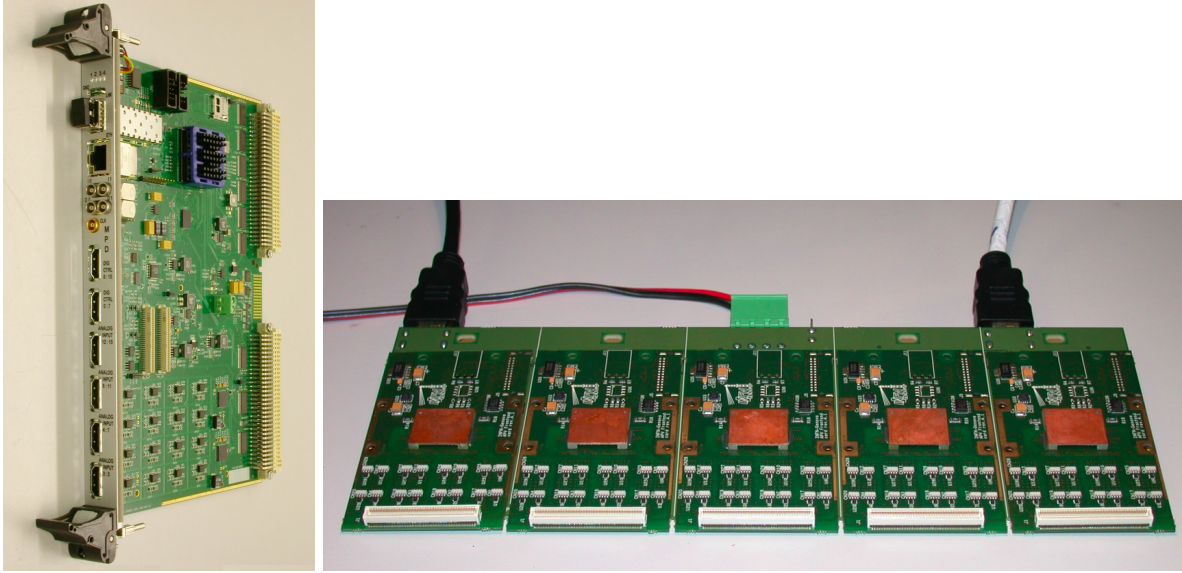
FIG. 9. Left: MPD4 VME module. Right: 5-slot APV backplane equipped with APV front-end v4.1.
