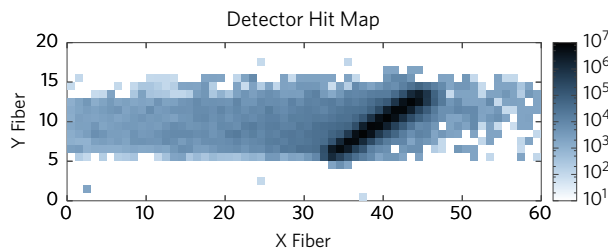
FIG. 18. Hit map on the focal plane detector for a 3 MeV beam at 25^\circ \pm 0.5^\circ . X Fiber corresponds to momentum (lowest left), and Y Fiber scattering angle (lowest top).
