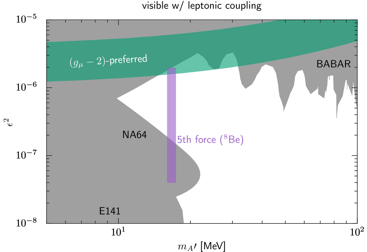
FIG. 1. Parameter space for a fifth force, with ^8\text{Be} and g - 2 anomalies in color. Vertical axis is the leptonic coupling strength. Excluded regions, in gray, are taken from experiments that have no dependence on hadronic couplings.
