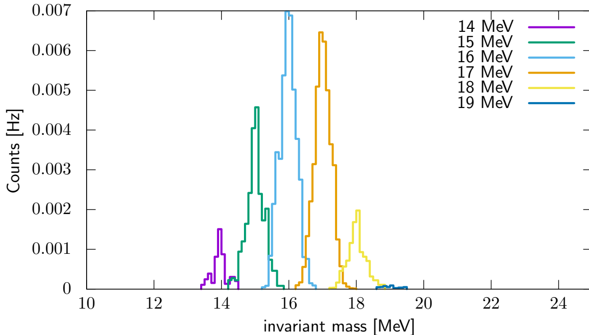
FIG. 10. Simulated signal and rates for A' candidates with a coupling of \epsilon^2 = 10^{-6} . Spectrometer acceptance was optimized for a 17 MeV mass, corresponding to the anomalous resonance in the {}^8\text{Be} spectra.
