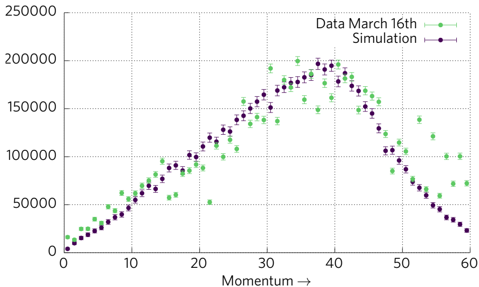
FIG. 20. Measured focal plane momentum distribution for radiative Møller electron scattering from carbon at 45^\circ electron scattering angle and incident energy of 2.5 MeV compared with simulation [13].
