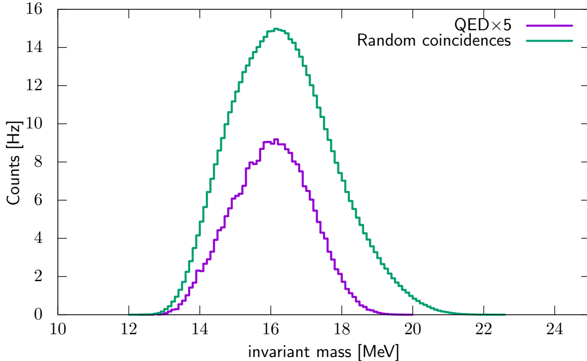
FIG. 11. Simulated background from QED diagrams and random coincidences.
