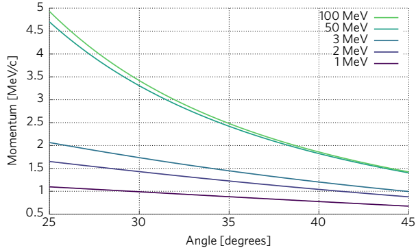
FIG. 15. Scattered Møller electron momentum as a function of angle for Møller scattering, for selected beam energies.
