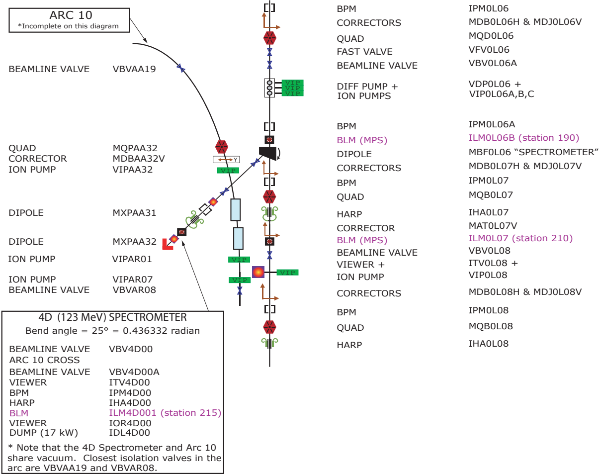
FIG. 2. The CEBAF injector layout in the vicinity of the proposed experiment. Beamline elements are at their approximate positions, but distances and sizes are not to scale. Further injector beamline elements upstream of the upper beam position monitor (IPM0L06) and downstream of the HARP (IHA0L08) are not shown. The injector beam can be diverted by the dipole (MBFOLO6) into the 4D Spectrometer region, in which the target and spectrometers would be placed.
