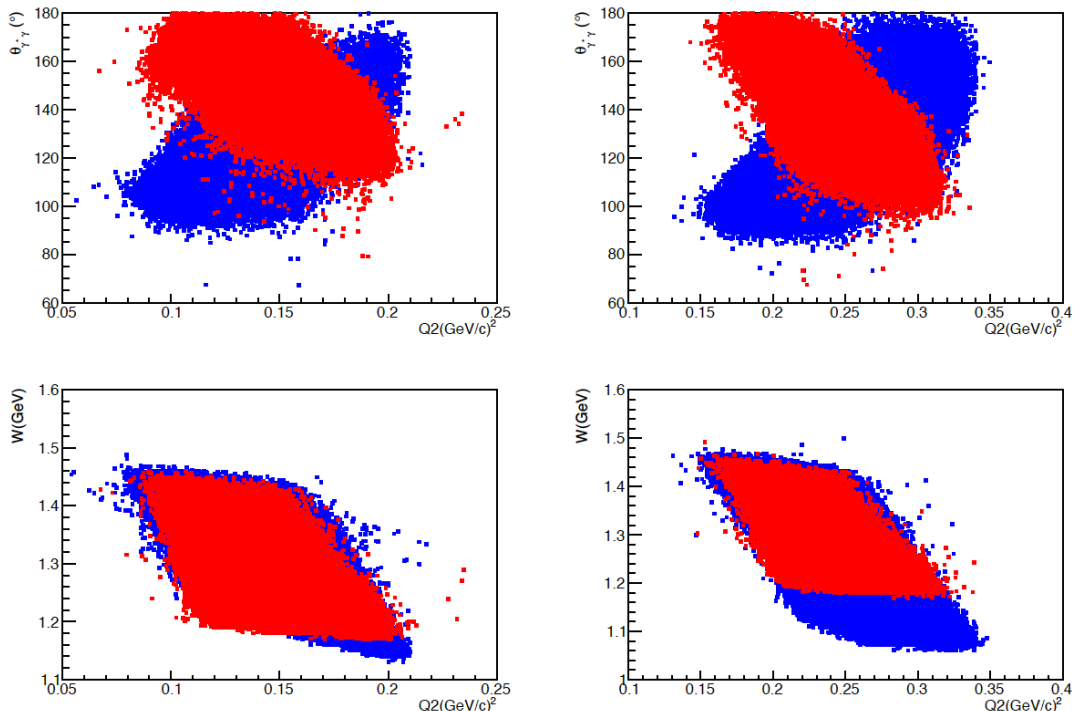
FIG. 12: (Left Q^2 = 0.15 \text{ GeV}^2 and Right Q^2 = 0.25 \text{ GeV}^2 ) Correlation of the phase space variables for a pair of \phi_{\gamma^*\gamma} = 0^\circ , 180^\circ measurements, with the two different colors corresponding to \phi_{\gamma^*\gamma} = 0^\circ and 180^\circ respectively. Left (top and bottom) and right (top and bottom) correspond to a pair of settings from kinematic groups GII and GIII, respectively.
