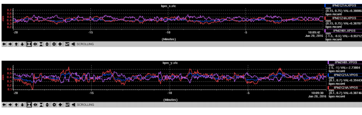
Figure 25: Beam X,Y position stability ( \approx \pm 0.1 mm) during the PRad experiment.
