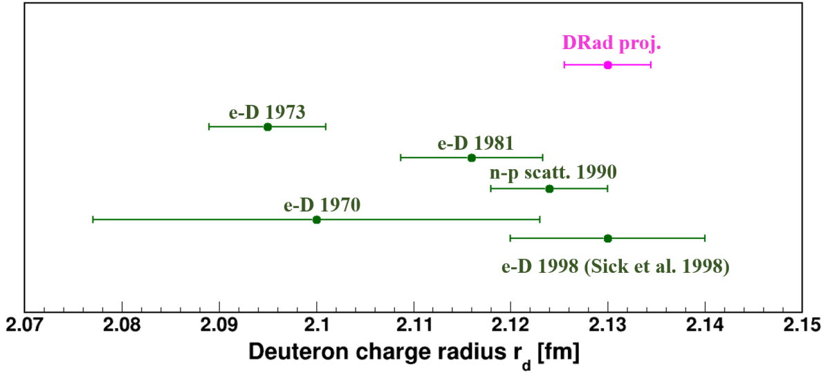
Figure 70: The projected DRad result along with CODATA values and other measurements as described in Fig. 2
