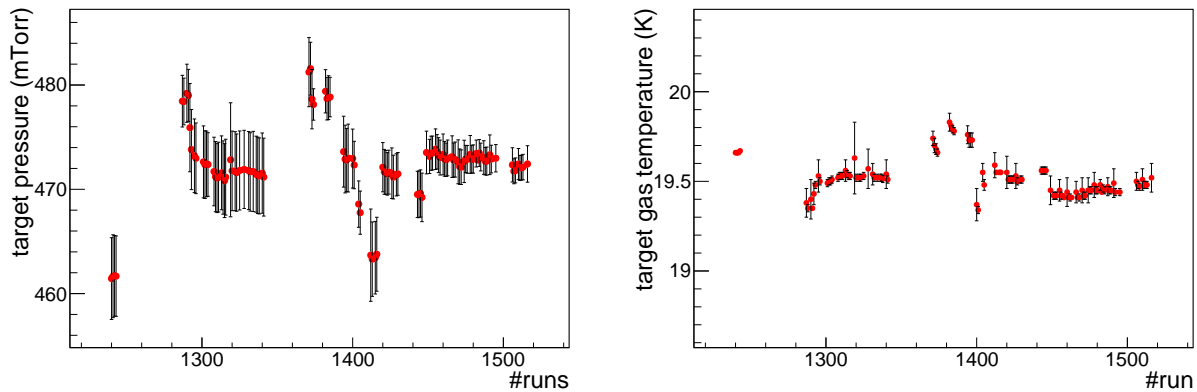
Figure 16: The variation of PRad target pressure and temperature vs. run number. Each run was about 1 hr long.
