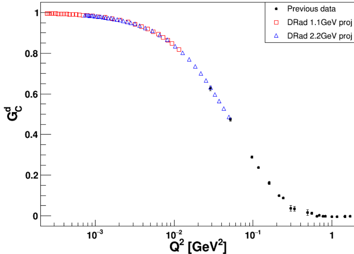
Figure 69: The projected charge form factor of the deuteron over the low Q^2 range covered in the experiment. Also shown are the previous data at low Q^2 .
