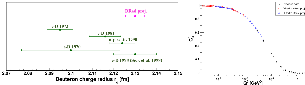
Figure 1: (left) The projected radius result along with other electron scattering measurements. (right) Projected charge form factor along with existing data. Larger versions of these figures are shown in Sec. 9.3
