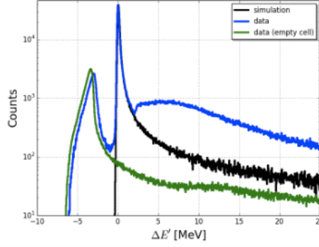
Figure 71: Distribution of elastic ed scattering data (blue) as a function of the \Delta E' = E'(\theta_e) - E' , along with simulation (black) and empty target events (green) for E_e = 315 MeV and \theta_e = 23.6^\circ . The events beyond \Delta E' = 2.2 MeV are from deuteron breakup while the events at \Delta E' < 0 are from the target cell wall. The figure is reproduced from Ref. [85].
