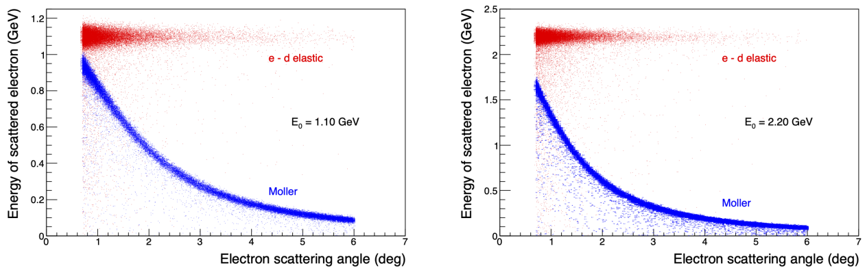
Figure 10: The simulated energy vs. scattering angle distribution of e - d elastic and one of the Møller scattered electrons at E_0 = 1.1 GeV (left) and at E_0 = 2.2 GeV (right). The ed and Møller event generators includes radiative effects, developed for the PRad experiment and the ed process.
