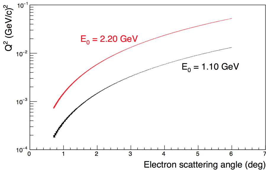
Figure 39: Four-momentum transfer squared ( Q^2 ) in e - d scattering vs. the electron scattering angle for both E_0 = 1.1 and 2.2 \text{ GeV} energies.
