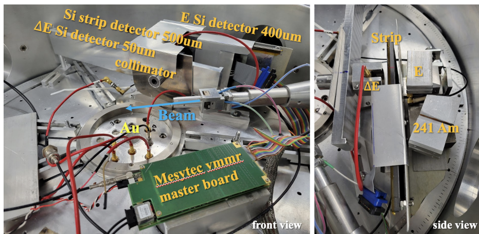
Figure 30: (left)The TUNL vacuum chamber showing front view of the test setup mounted on rails with the beam entering the chamber from the left. (right) The side view of the setup showing a close up view of the 3 detectors and collimators.
