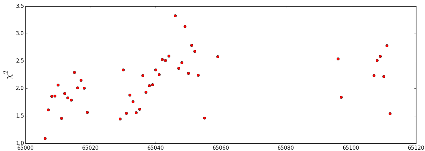
Single Arm Carbon: 149 runs between 64716 - 64988
