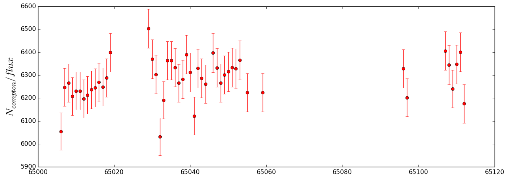
Single Arm Carbon: 149 runs between 64716 - 64988
