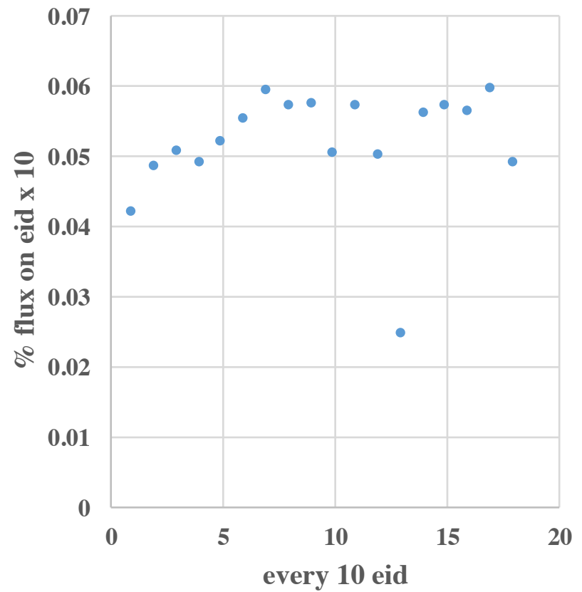
flux vs eid x 10
