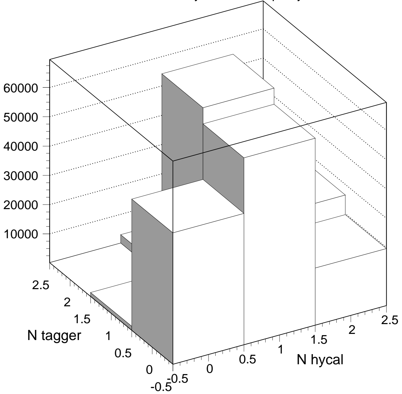
TAGM-LR VS HyCal hist multiplicity
