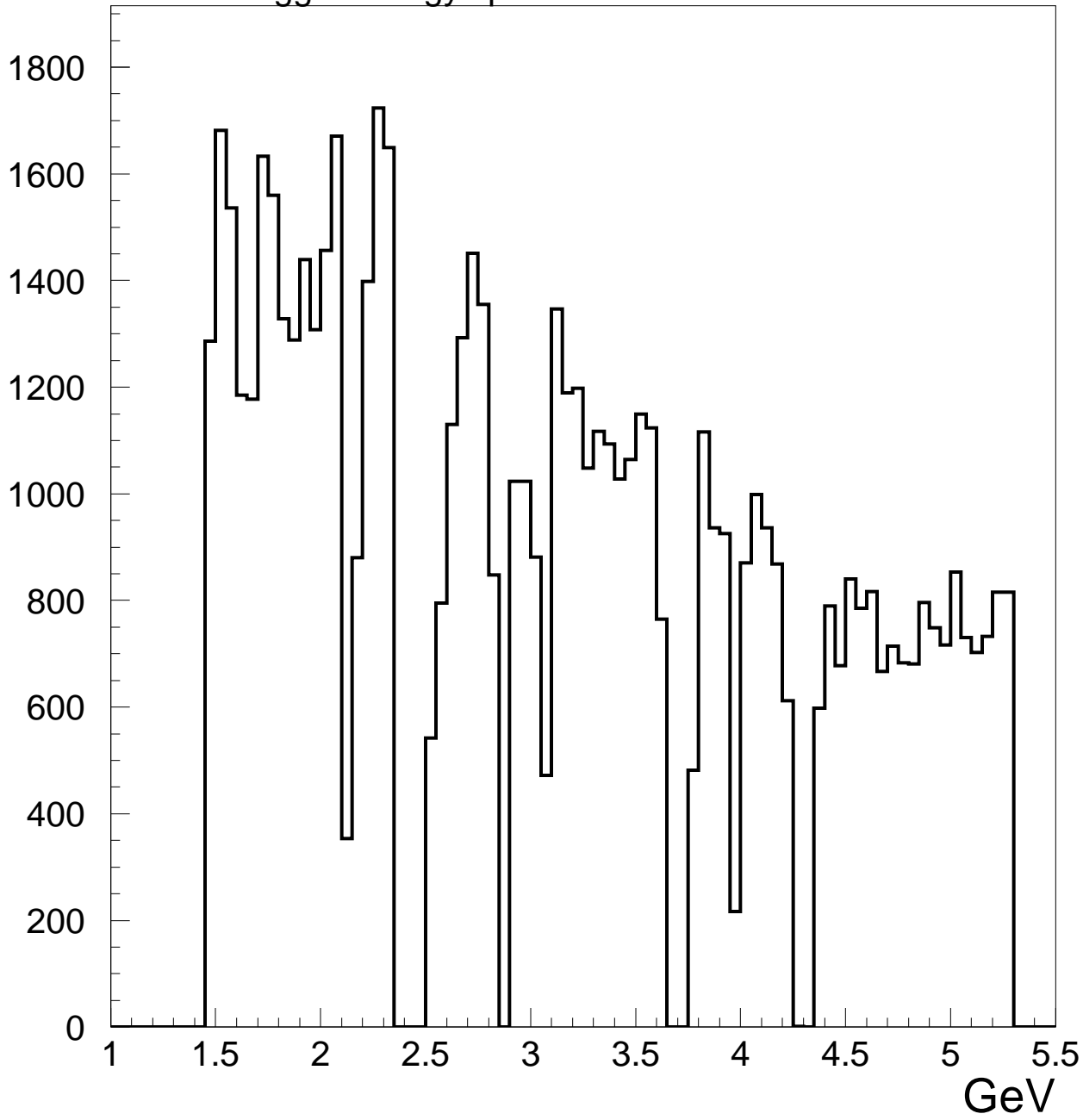
Tagger energy spectrum for Run=65116
