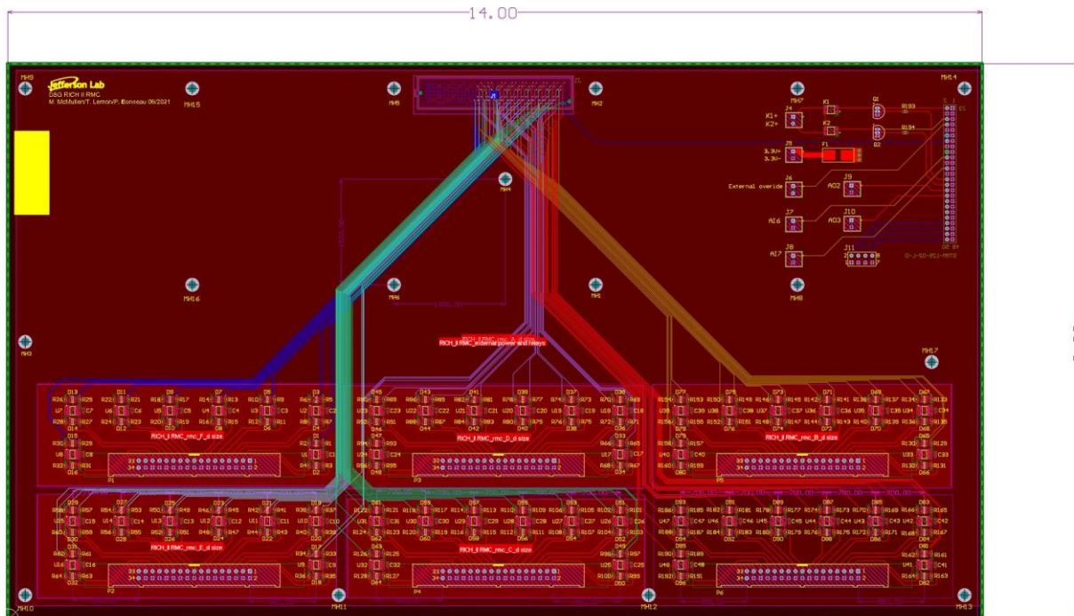
RMC design in Altium
