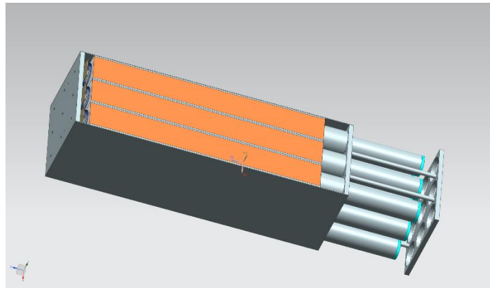
Screenshot of NX12 model of supermodule
