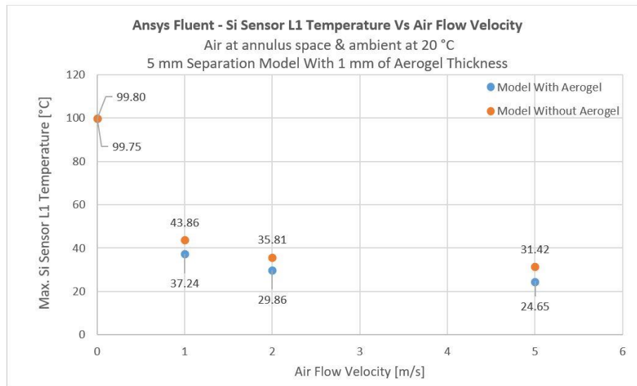
Plot of results at various air flow velocities with and without aerogel.
