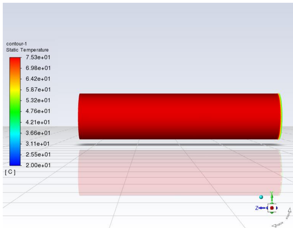
Right side view of silicon sensor layer with air flow velocity of 1 \times 10^{-7} m/s (effectively no air flow)
