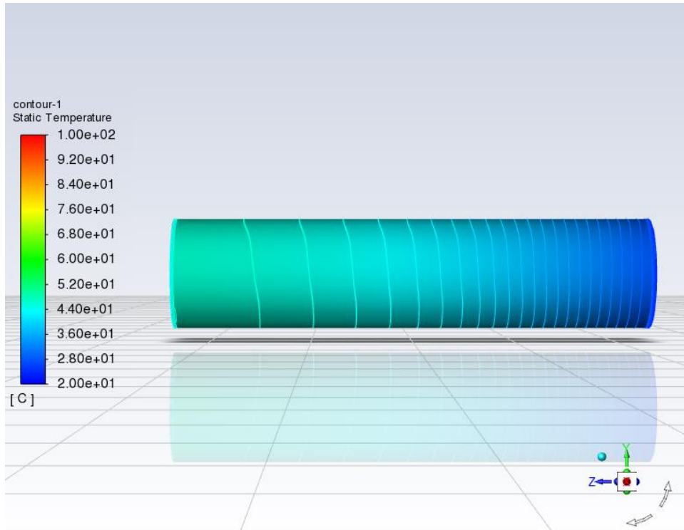
Right side view of silicon sensor layer with air flow velocity of 1 m/s
