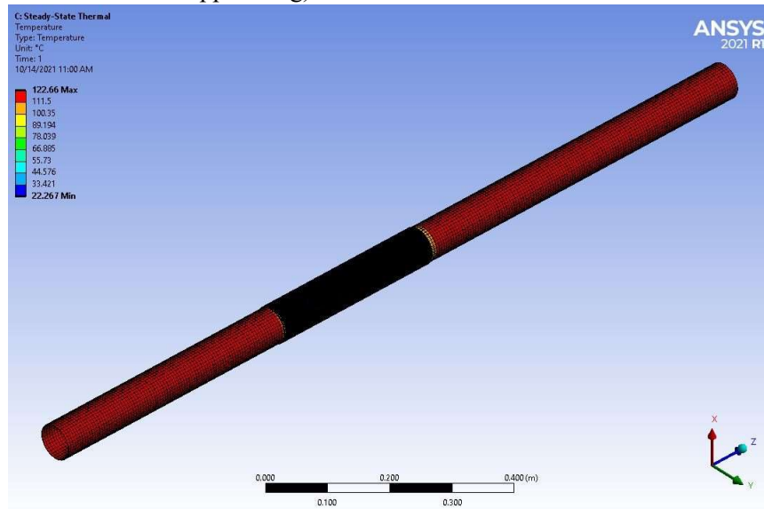
Simplified EIC Beampipe and Silicon Tracking Geometry
