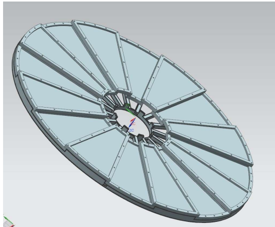
Work-in-progress of MPGD support structure (trapezoid overlap to be increased for no dead-area)
