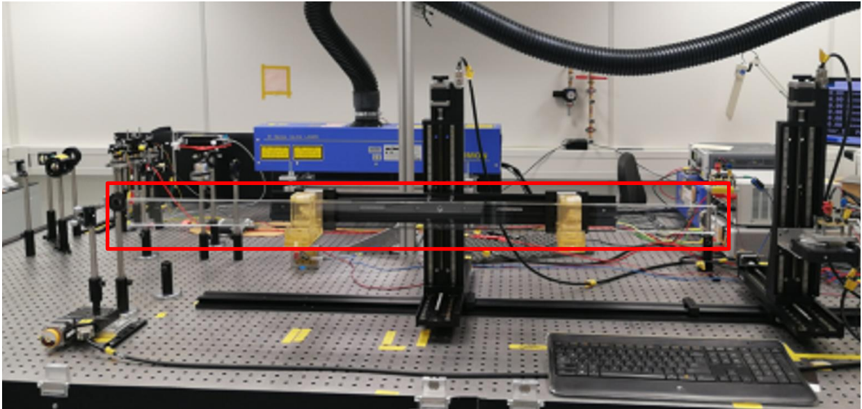
Photo of one bar, in red box, installed into previous test station at GSI, mounted on linear stages.
