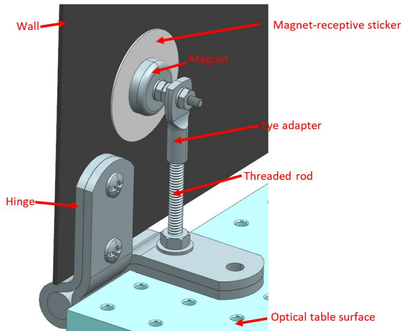
Model of proposed side wall hinge with magnetic holder.
