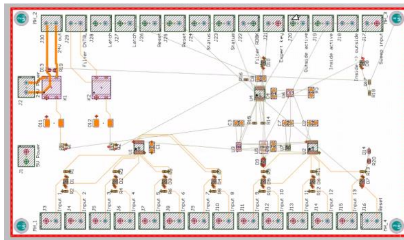
Screenshot of Altium editor of PCB layout; trace routing in progress
