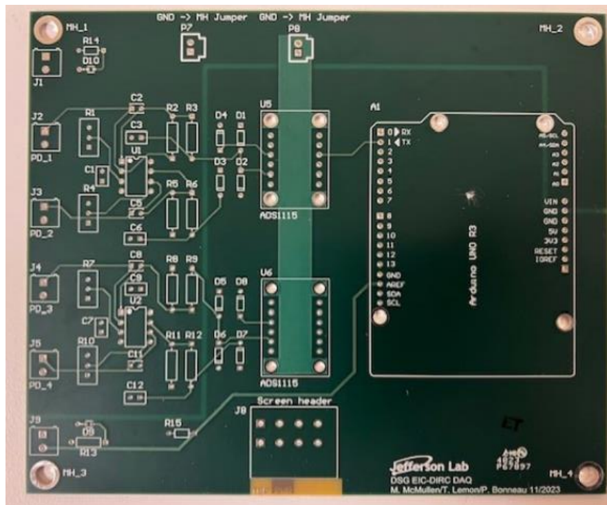
Bare PCB received from manufacturer
