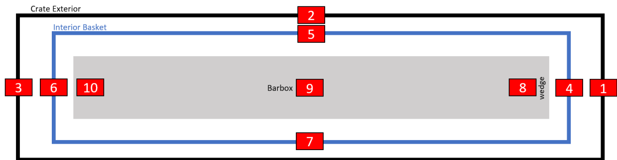
Sketch diagram of accelerometer locations in crates for EIC Shipping.
