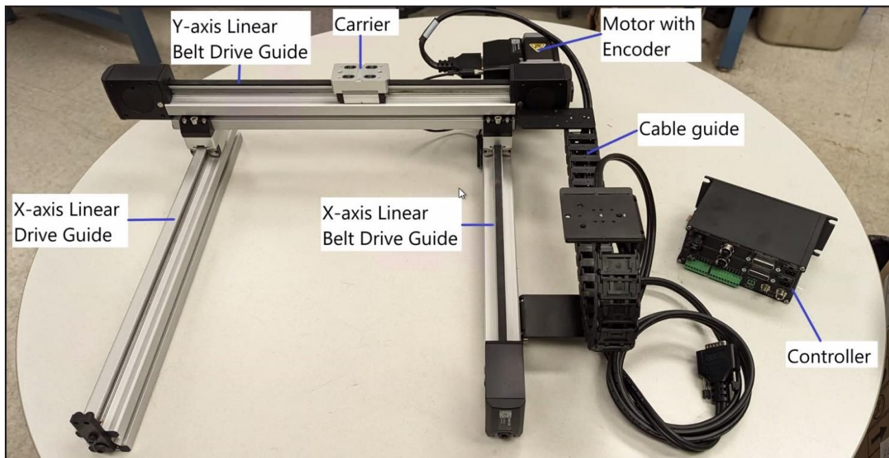
Assembled gantry for LAPPD
