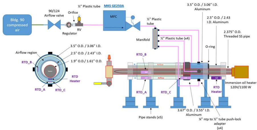
EIC Beampipe thermal test stand diagram
