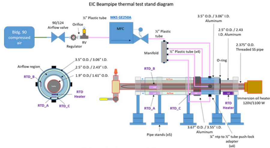
EIC Beamline Test Stand Airflow Test
