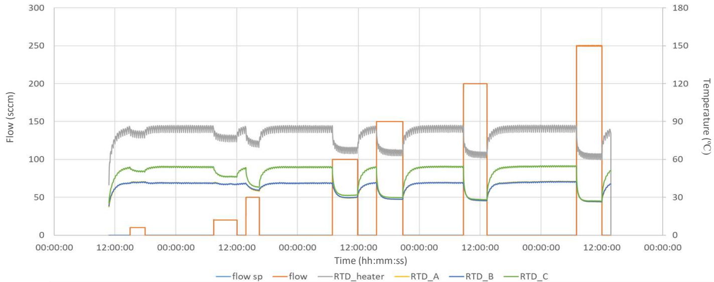
EIC Beamline Test Stand Airflow Test
