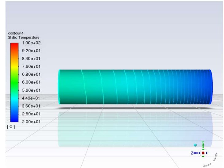
Right side view of silicon sensor with air flow velocity at 1 m/s
