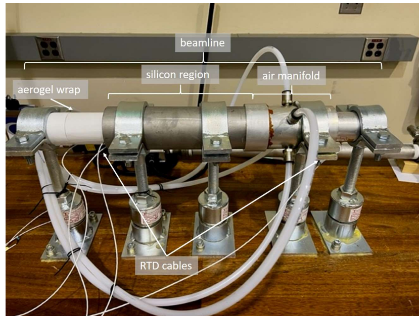
Reassembly of the simulated beam line with aerogel wrap added to the inner pipe
