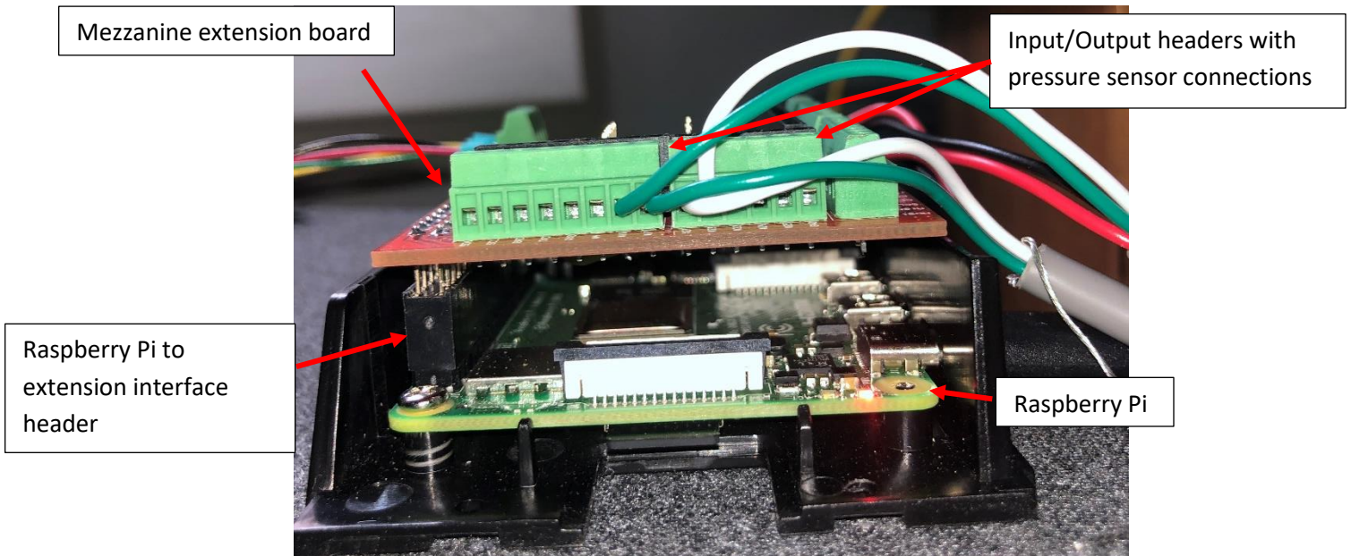
Figure 1. GEM gas readout system Raspberry Pi with mezzanine expansion board, which provides connection to the pressure and flow sensors
