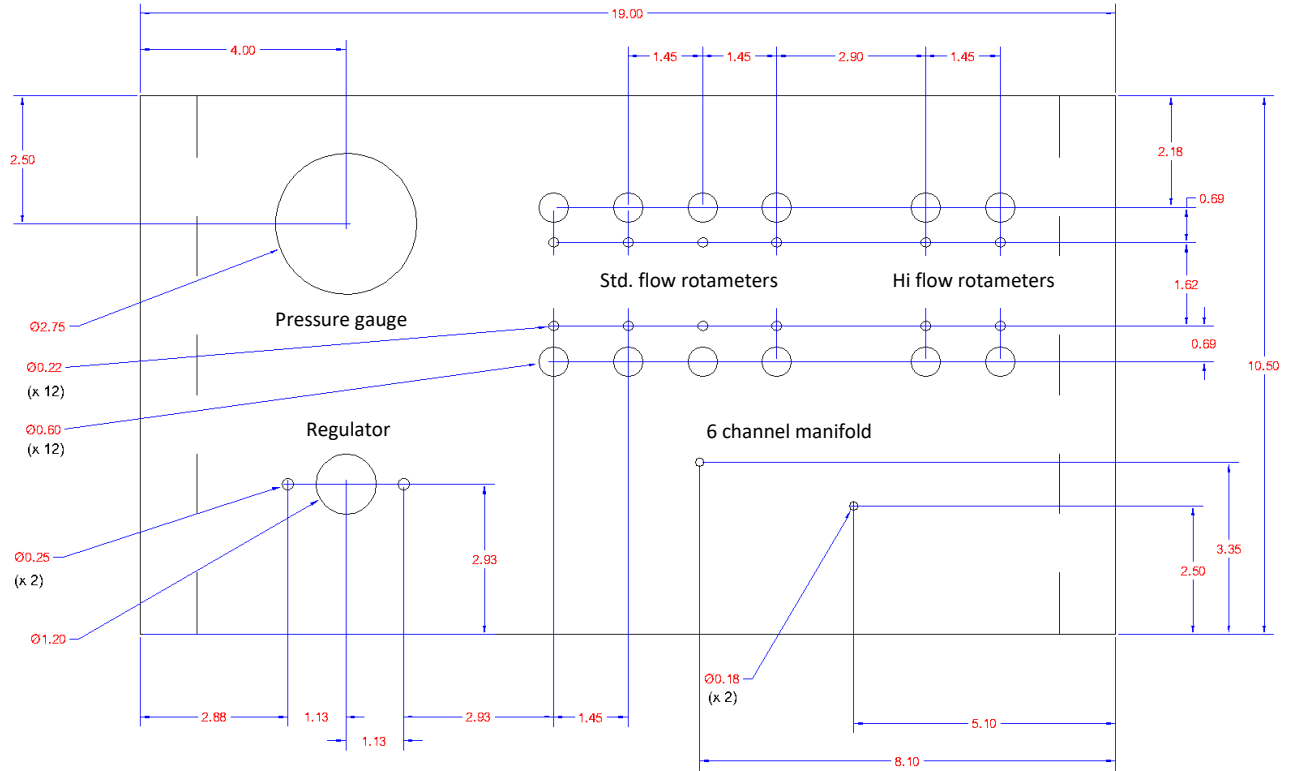
Front panel of supplemental gas distribution chassis; dimensions in inches
