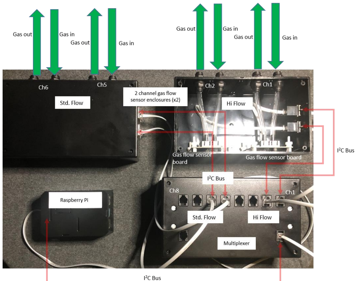
DSG-designed exhaust flow sensor and multiplexer system
