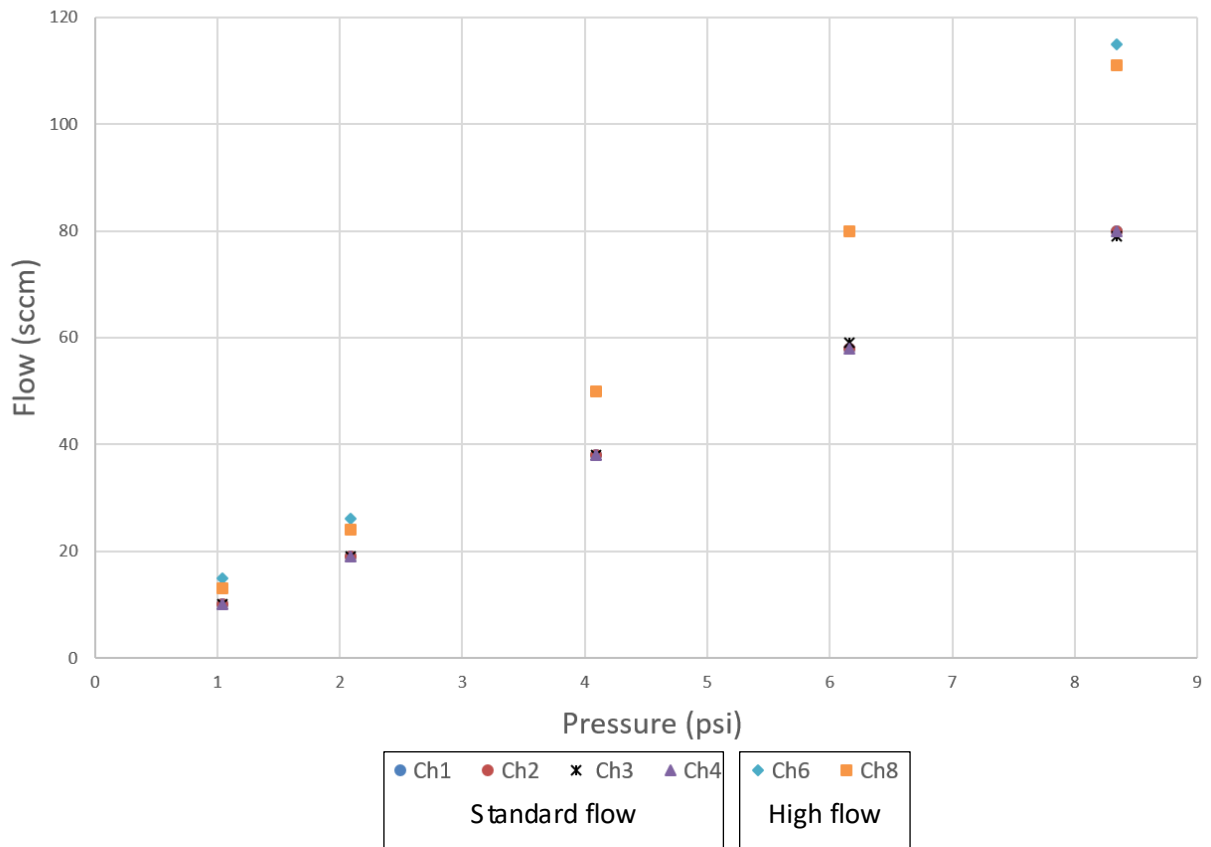
BigBite gas distribution system: Pressure variation vs. flow
