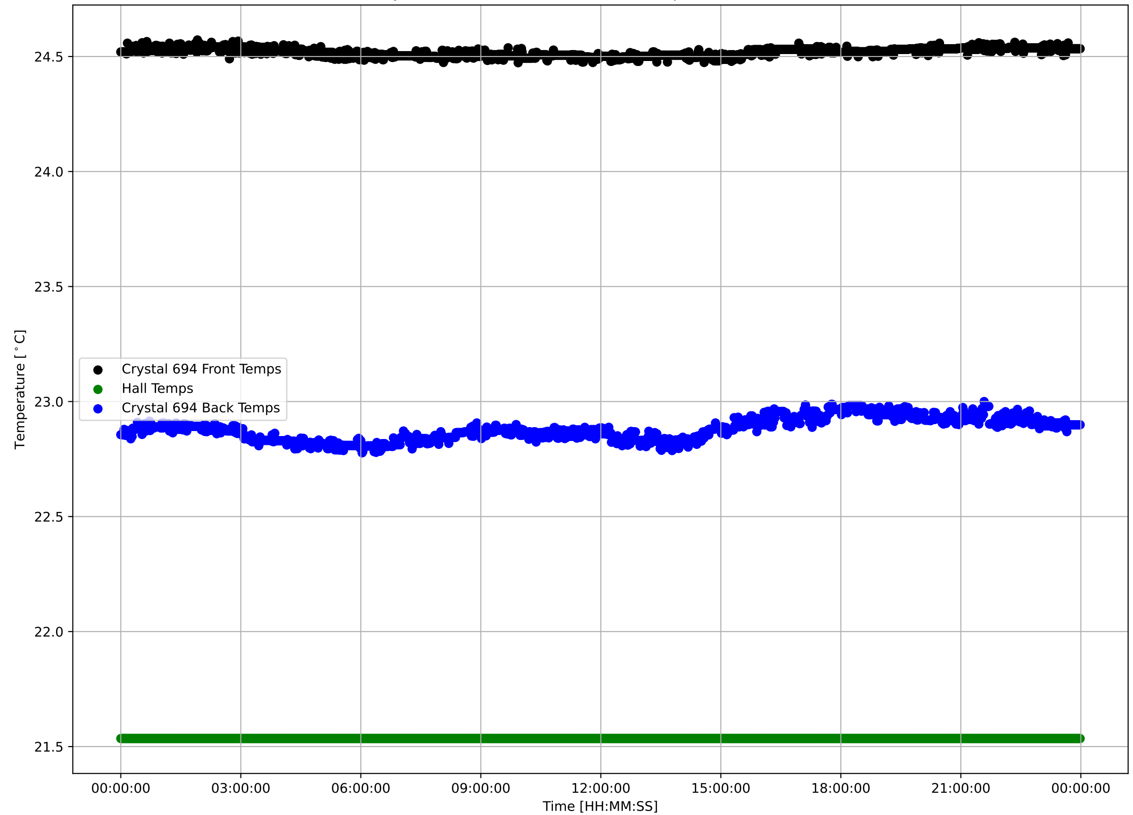
Crystal 694 Front, Back, and Hall Temps v Time - 240404
