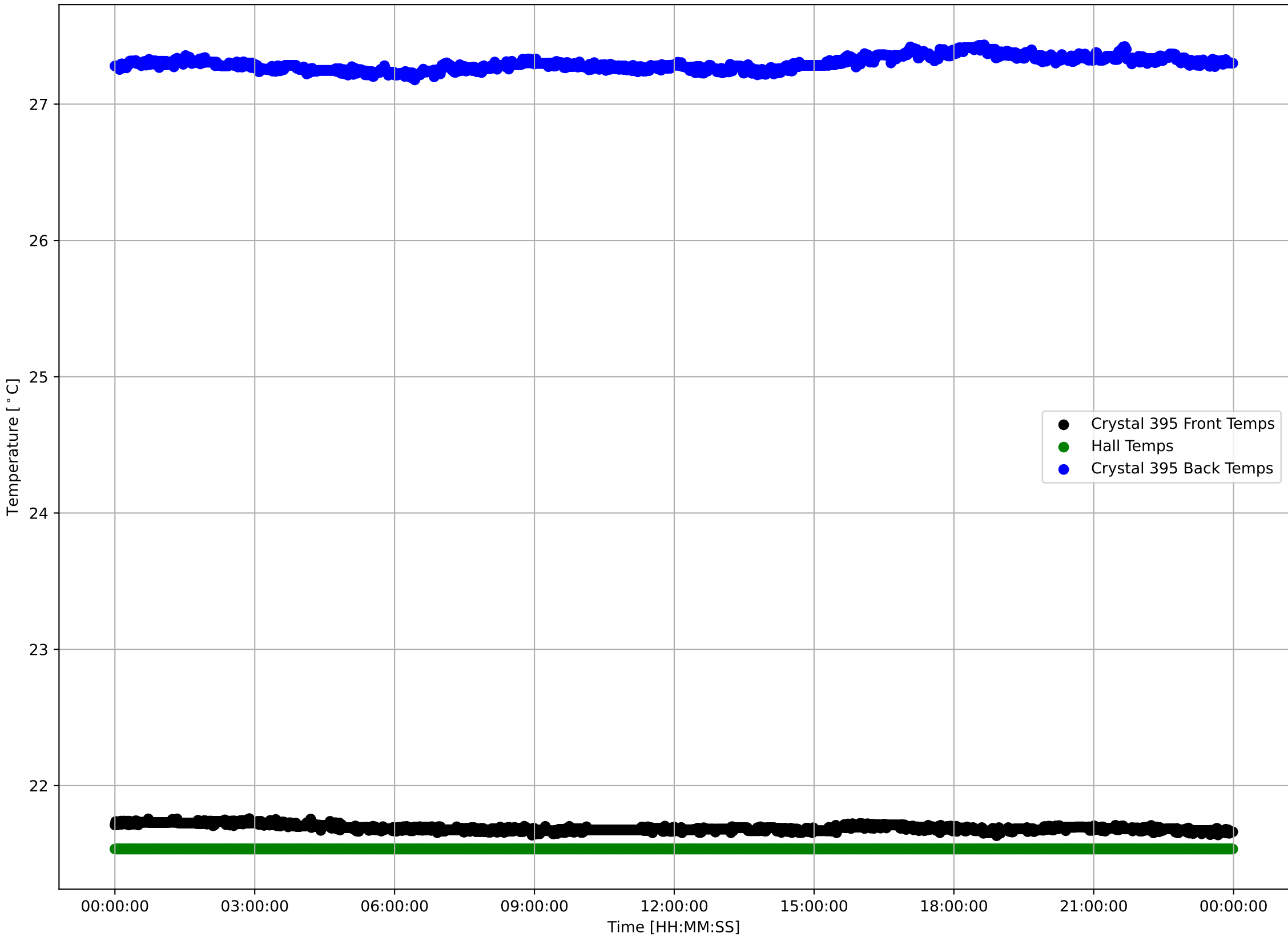
Crystal 395 Front, Back, and Hall Temps v Time - 240404
