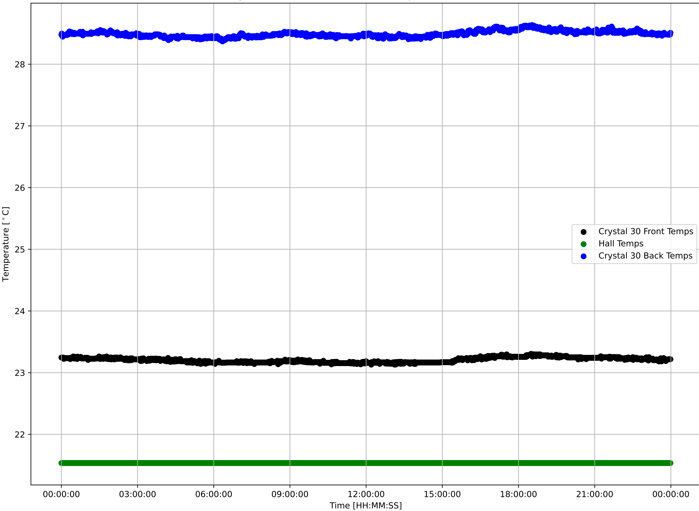
Crystal 30 Front, Back, and Hall Temps v Time - 240404
