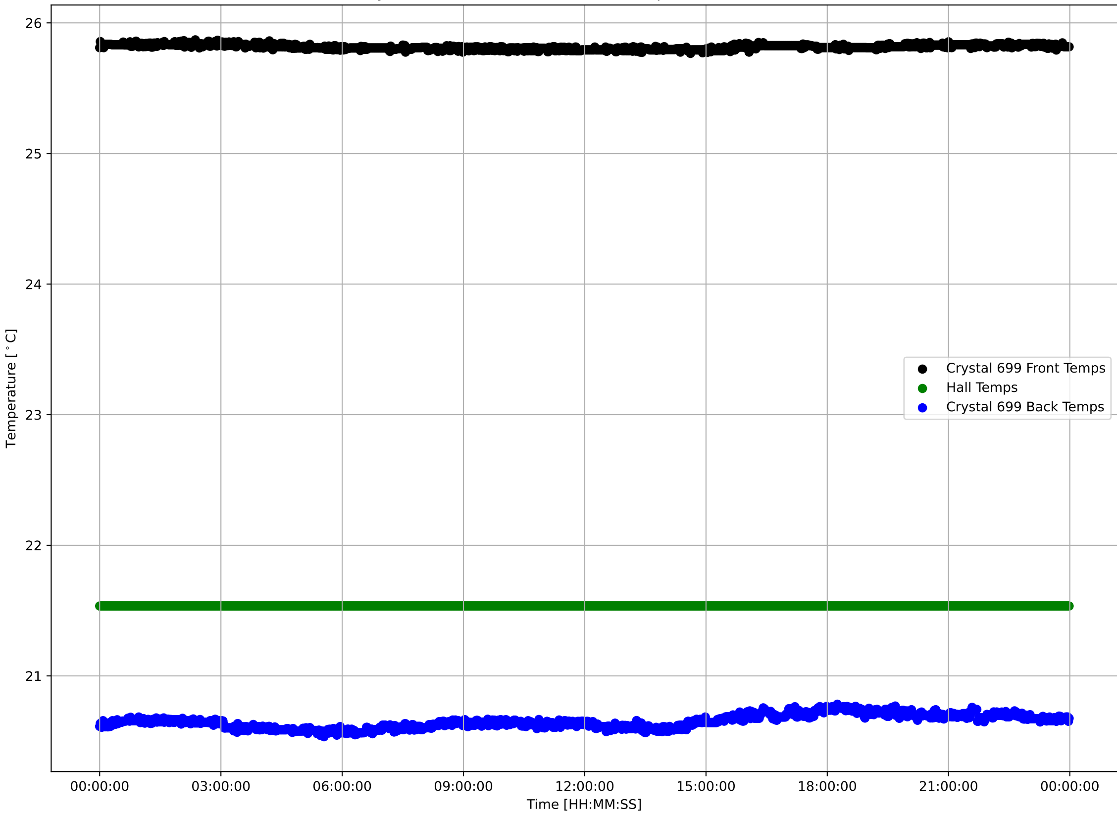
Crystal 699 Front, Back, and Hall Temps v Time - 240404
