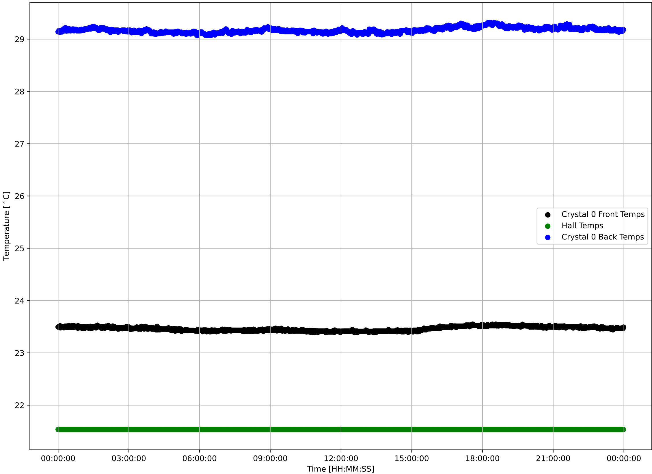
Crystal 0 Front, Back, and Hall Temps v Time - 240404
