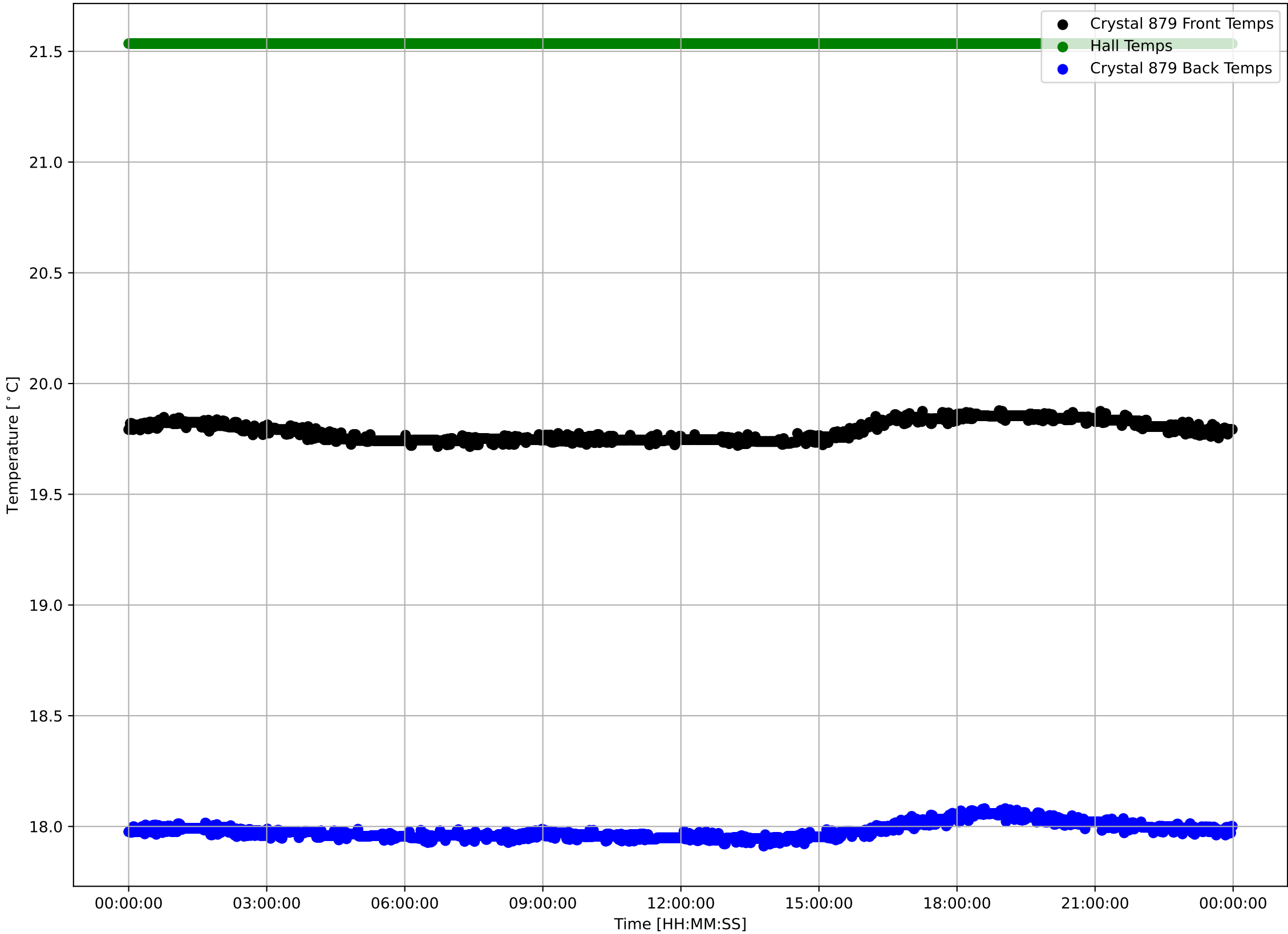
Crystal 879 Front, Back, and Hall Temps v Time - 240404
