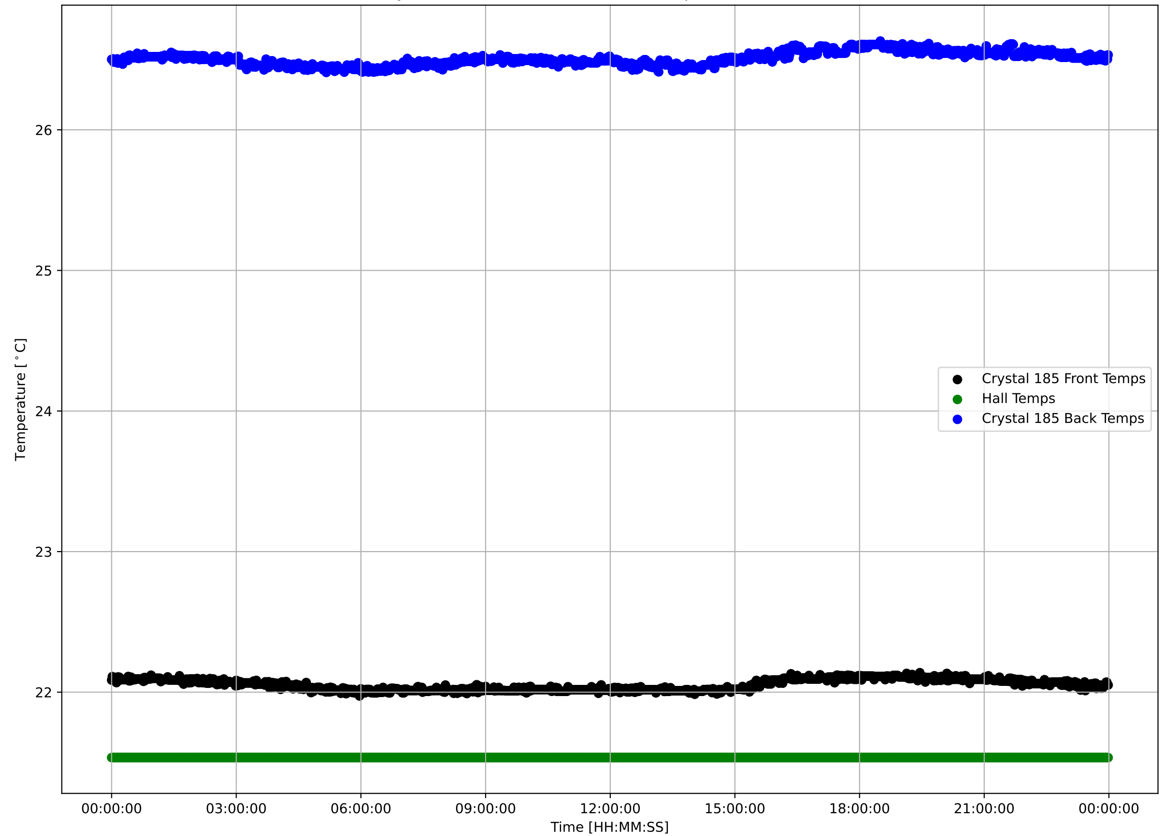
Crystal 185 Front, Back, and Hall Temps v Time - 240404
