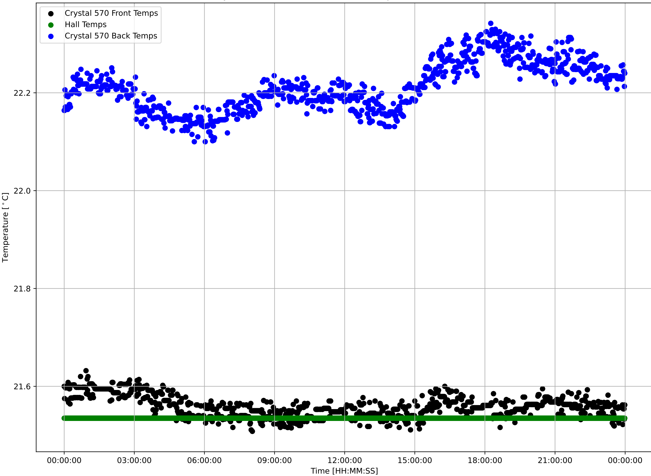
Crystal 570 Front, Back, and Hall Temps v Time - 240404
