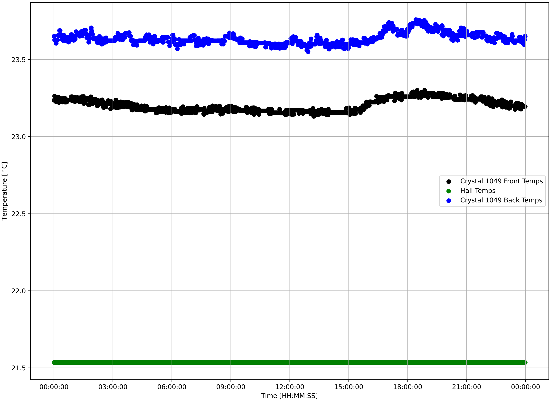
Crystal 1049 Front, Back, and Hall Temps v Time - 240404
