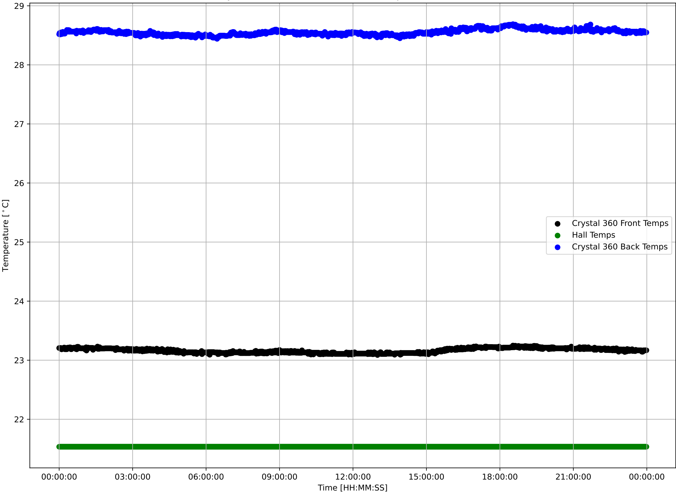
Crystal 360 Front, Back, and Hall Temps v Time - 240404
