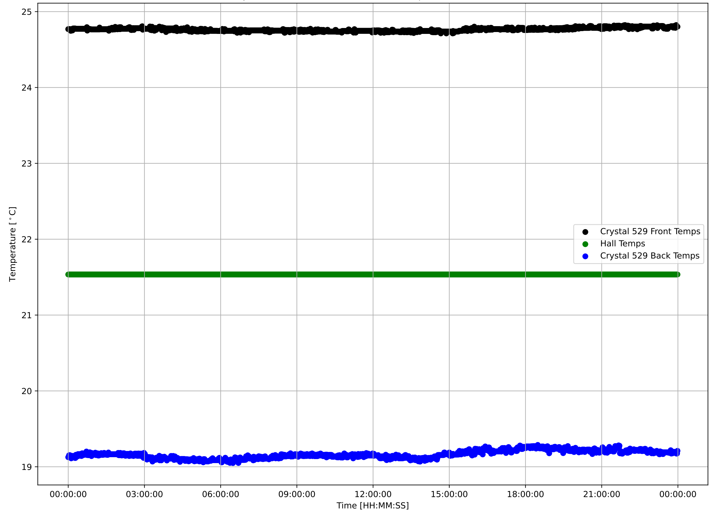
Crystal 529 Front, Back, and Hall Temps v Time - 240404
