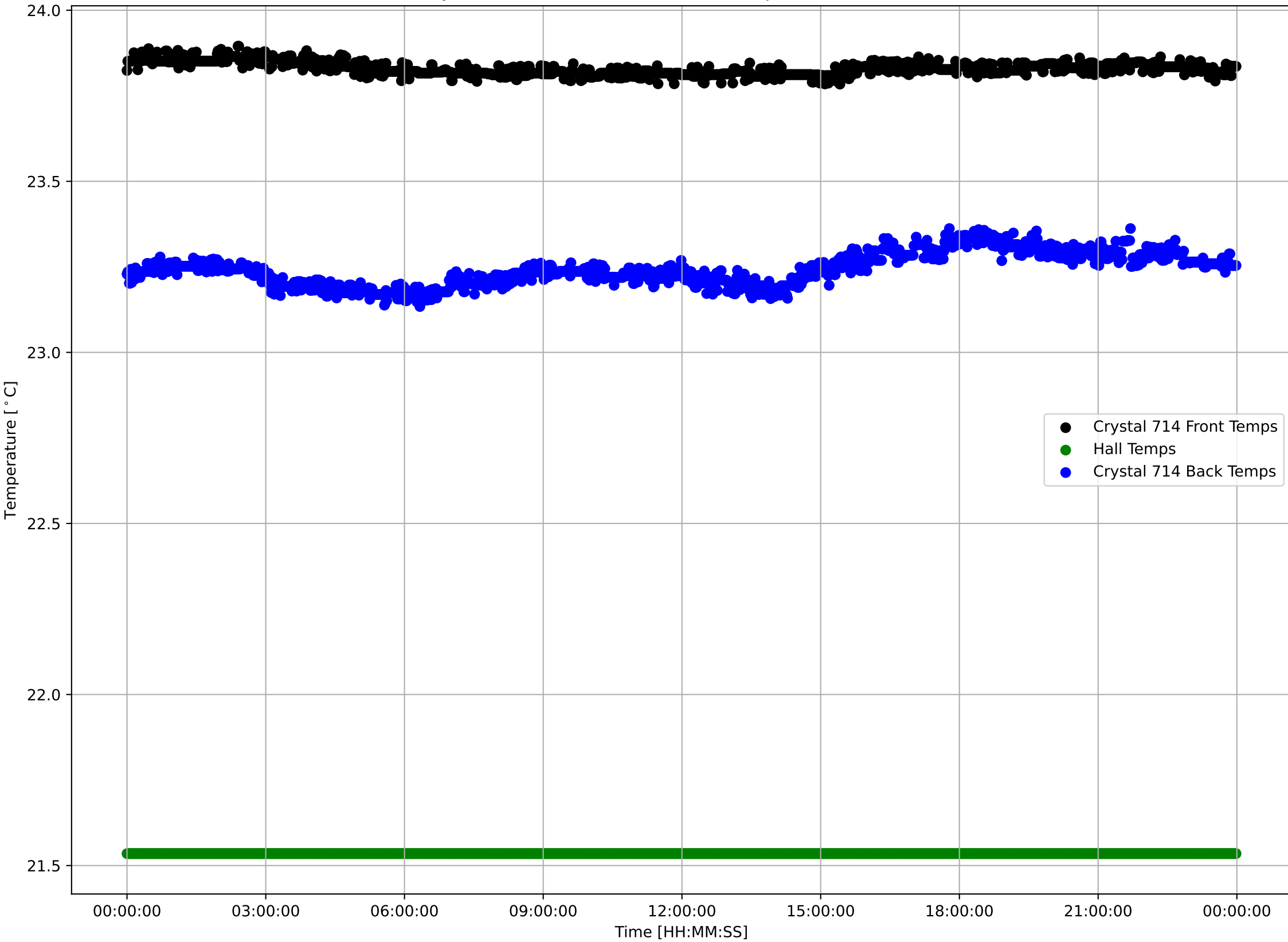
Crystal 714 Front, Back, and Hall Temps v Time - 240404
