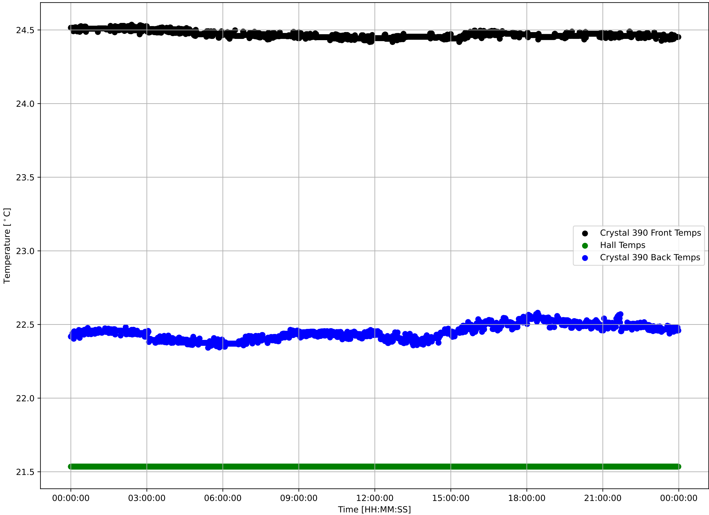
Crystal 390 Front, Back, and Hall Temps v Time - 240404
