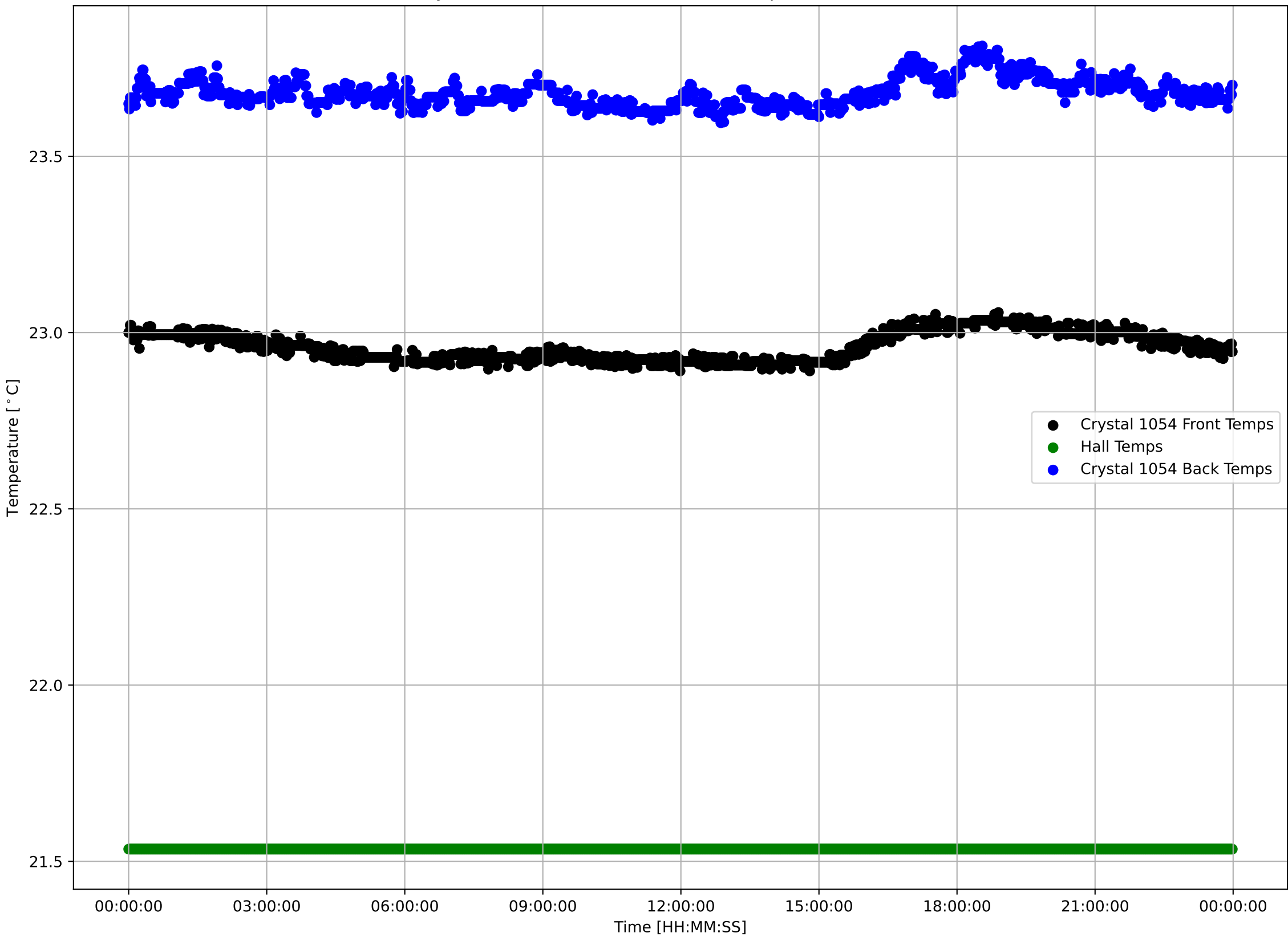
Crystal 1054 Front, Back, and Hall Temps v Time - 240404
