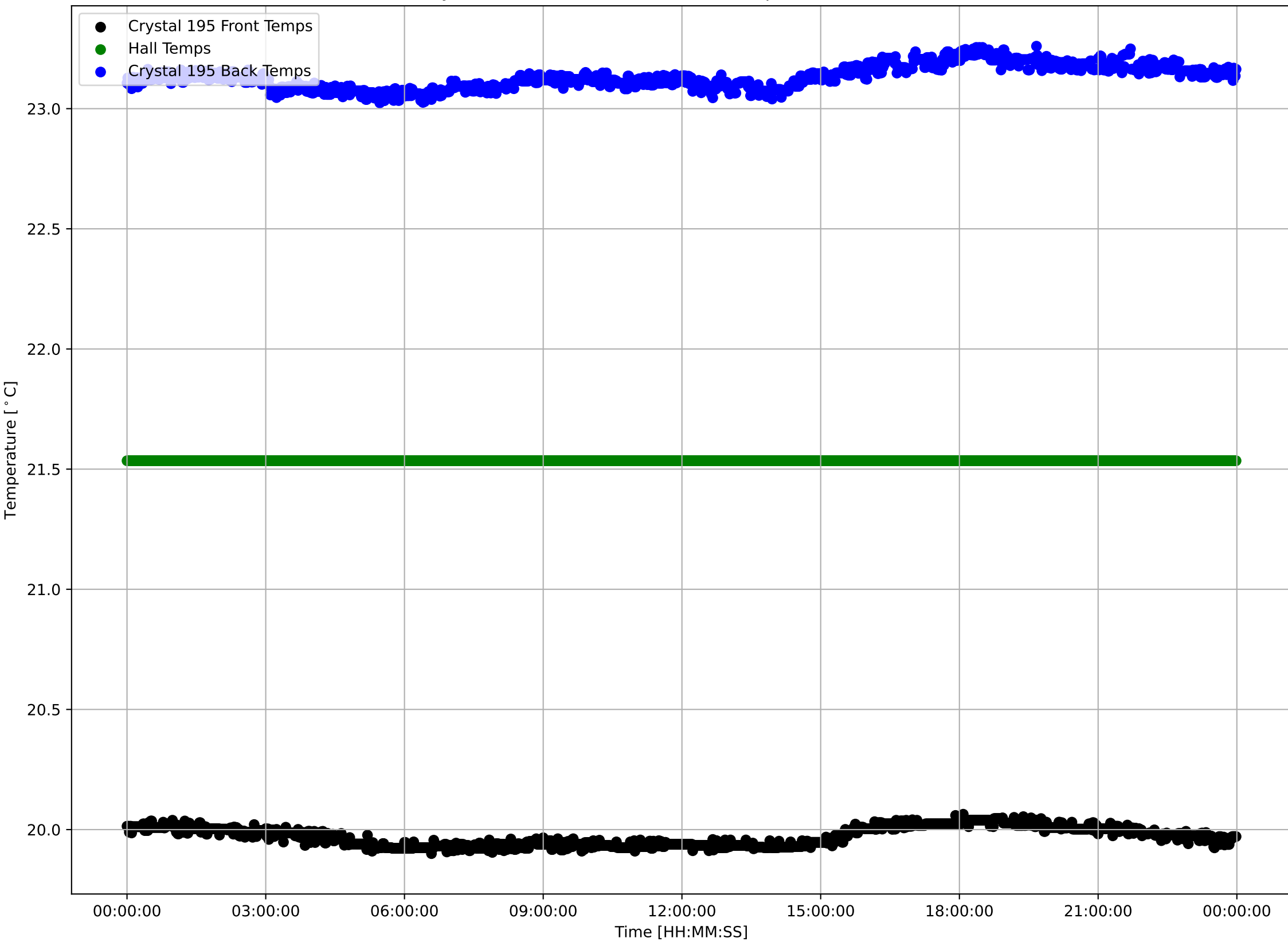
Crystal 195 Front, Back, and Hall Temps v Time - 240404
