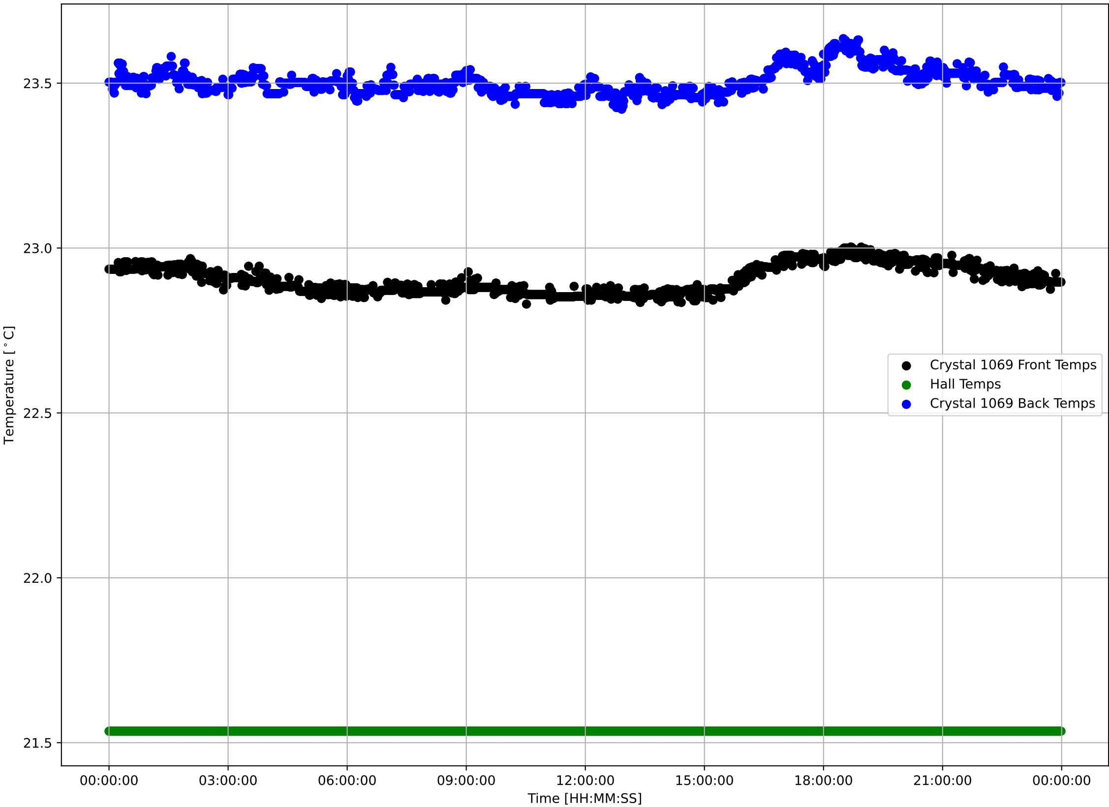
Crystal 1069 Front, Back, and Hall Temps v Time - 240404
