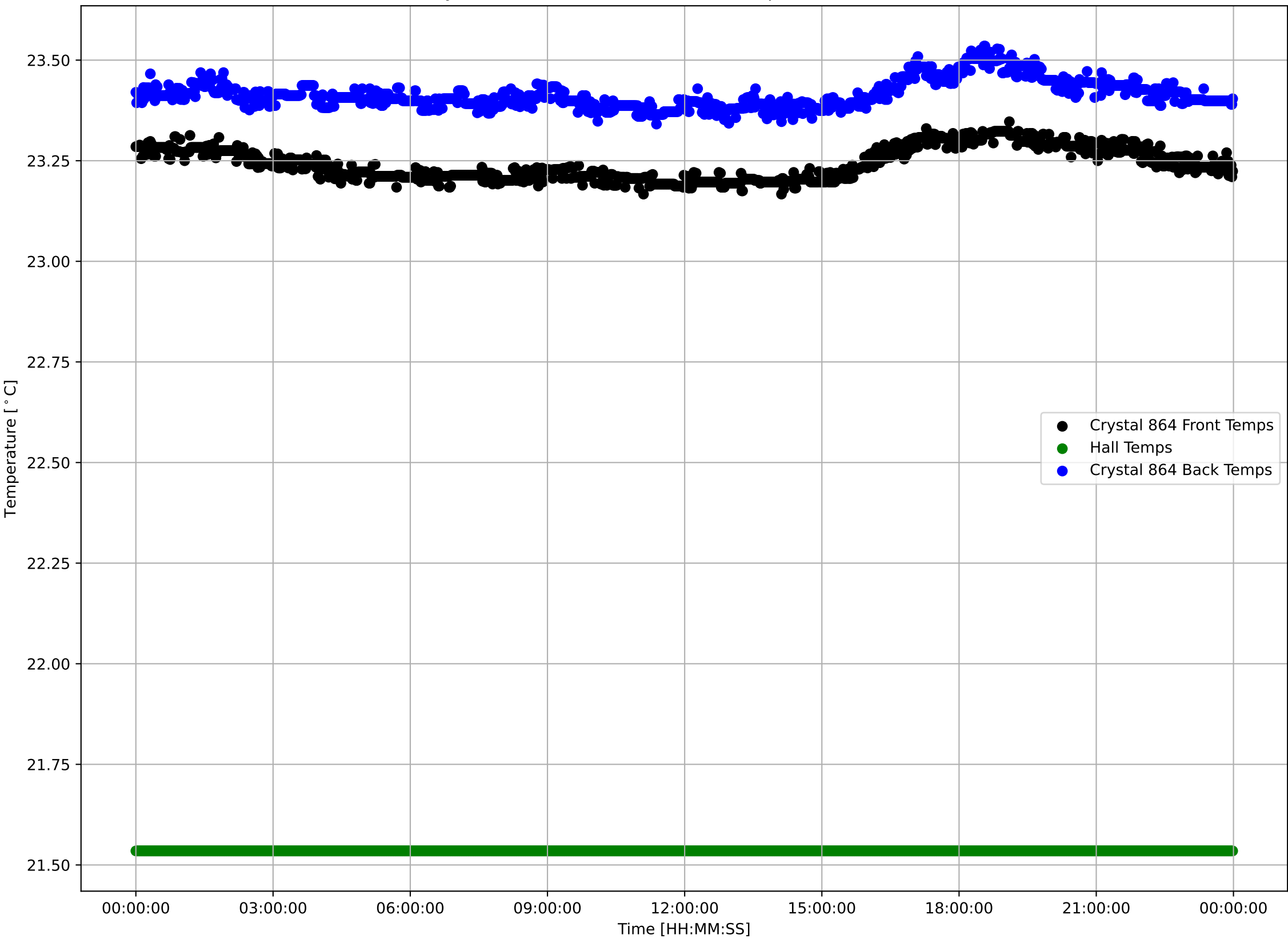
Crystal 864 Front, Back, and Hall Temps v Time - 240404
