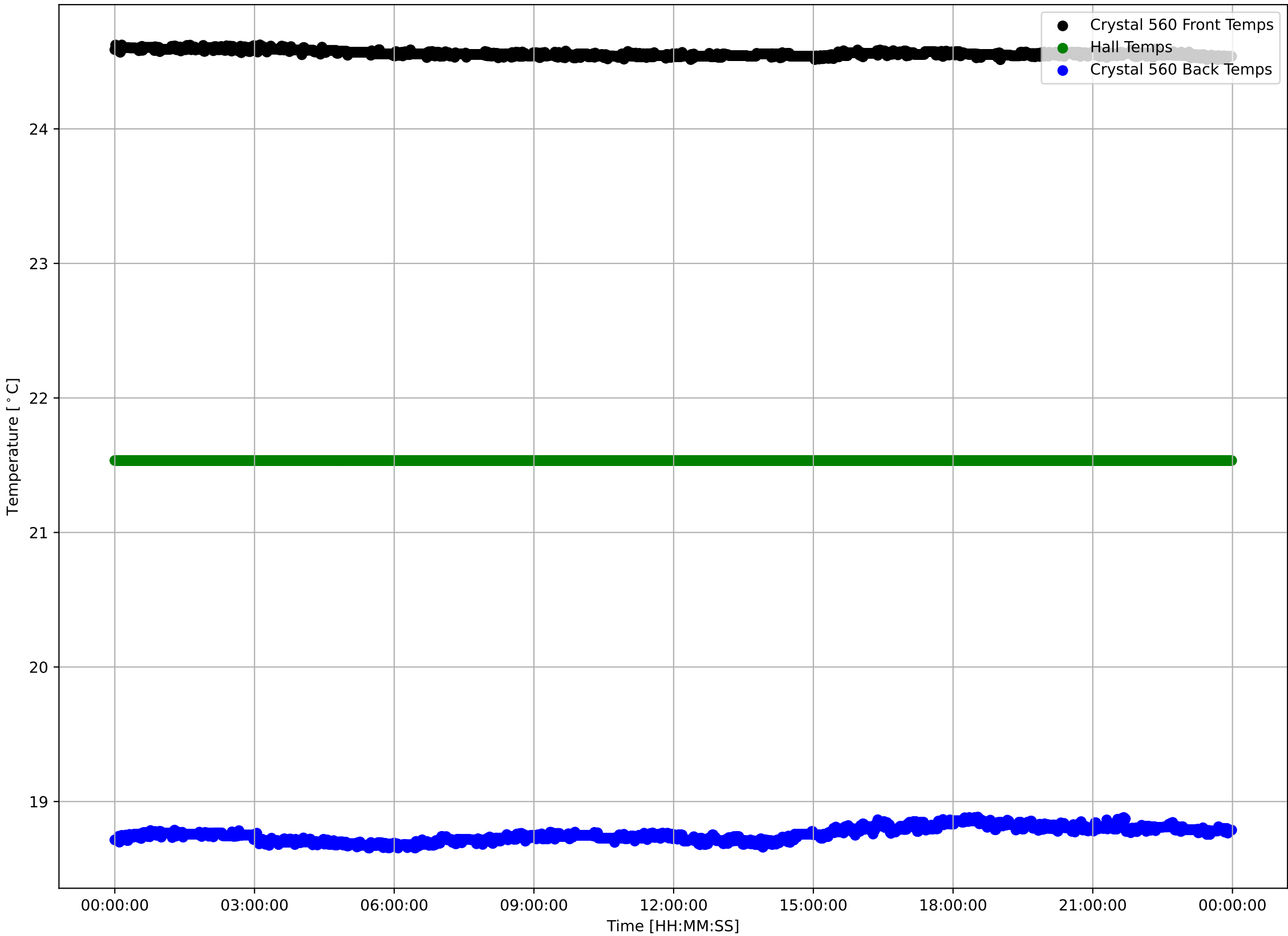
Crystal 560 Front, Back, and Hall Temps v Time - 240404
