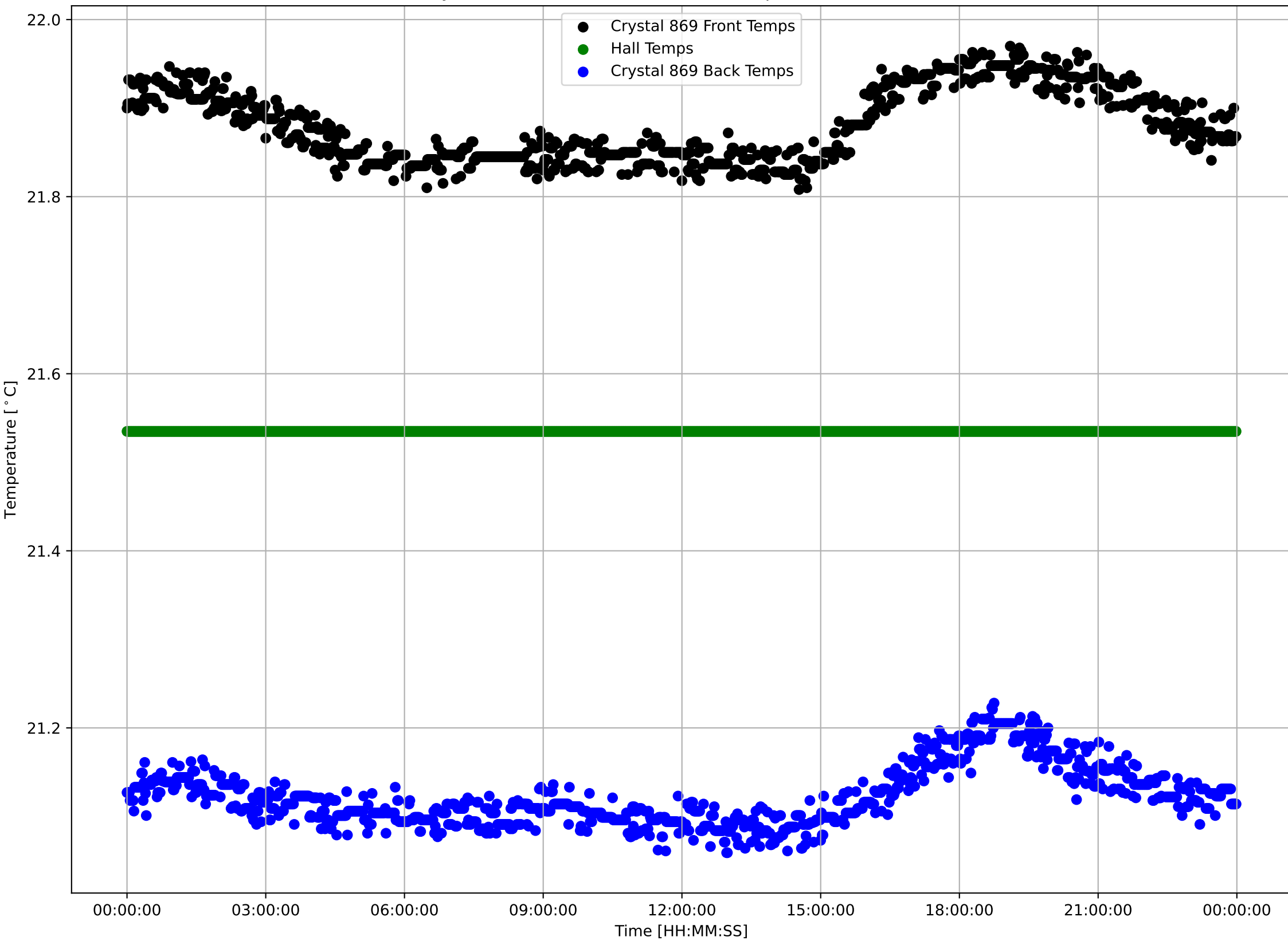
Crystal 869 Front, Back, and Hall Temps v Time - 240404
