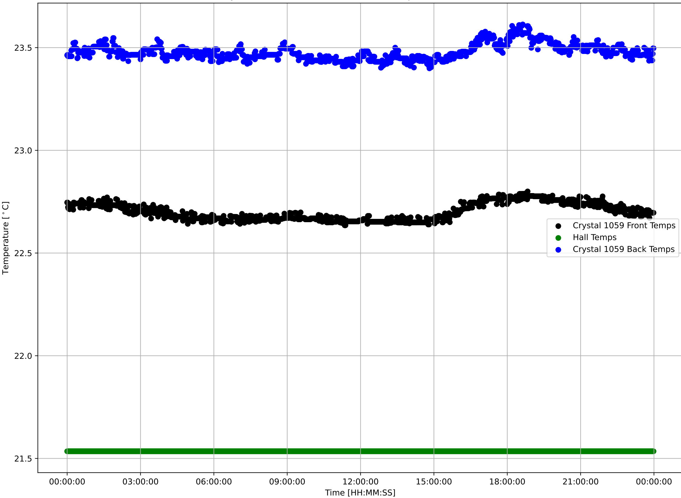
Crystal 1059 Front, Back, and Hall Temps v Time - 240404
