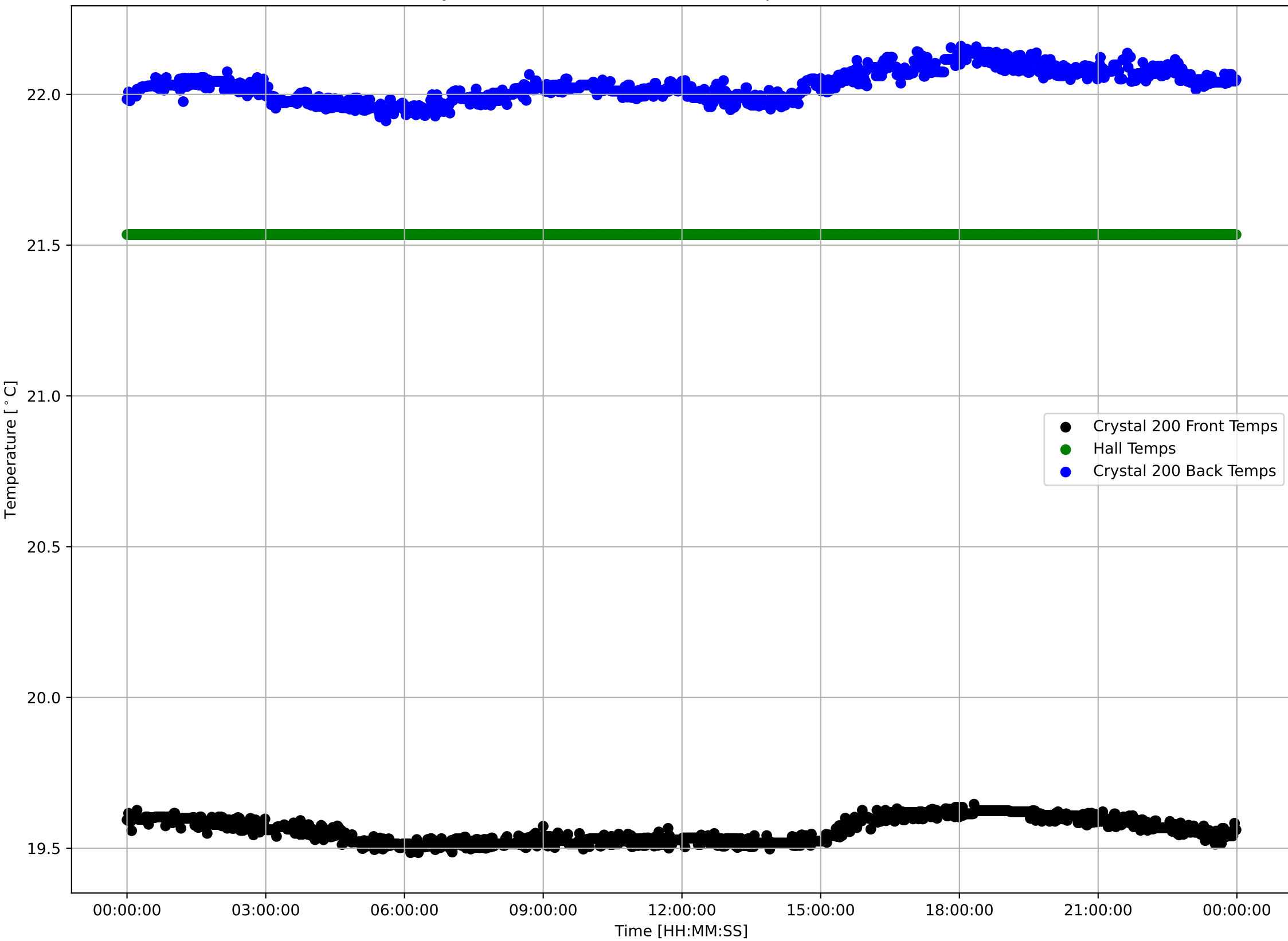
Crystal 200 Front, Back, and Hall Temps v Time - 240404
