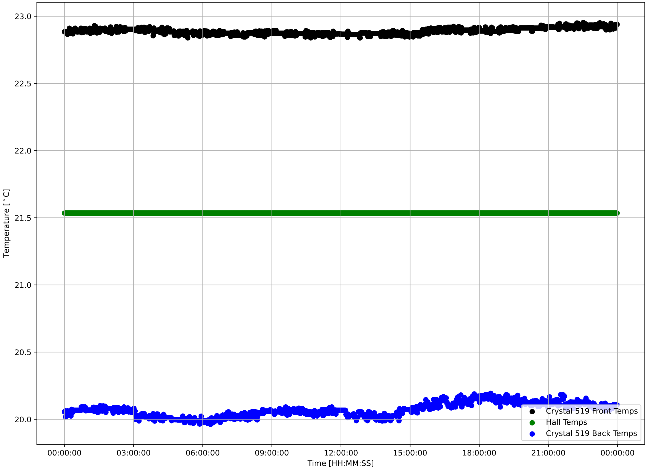
Crystal 519 Front, Back, and Hall Temps v Time - 240404
