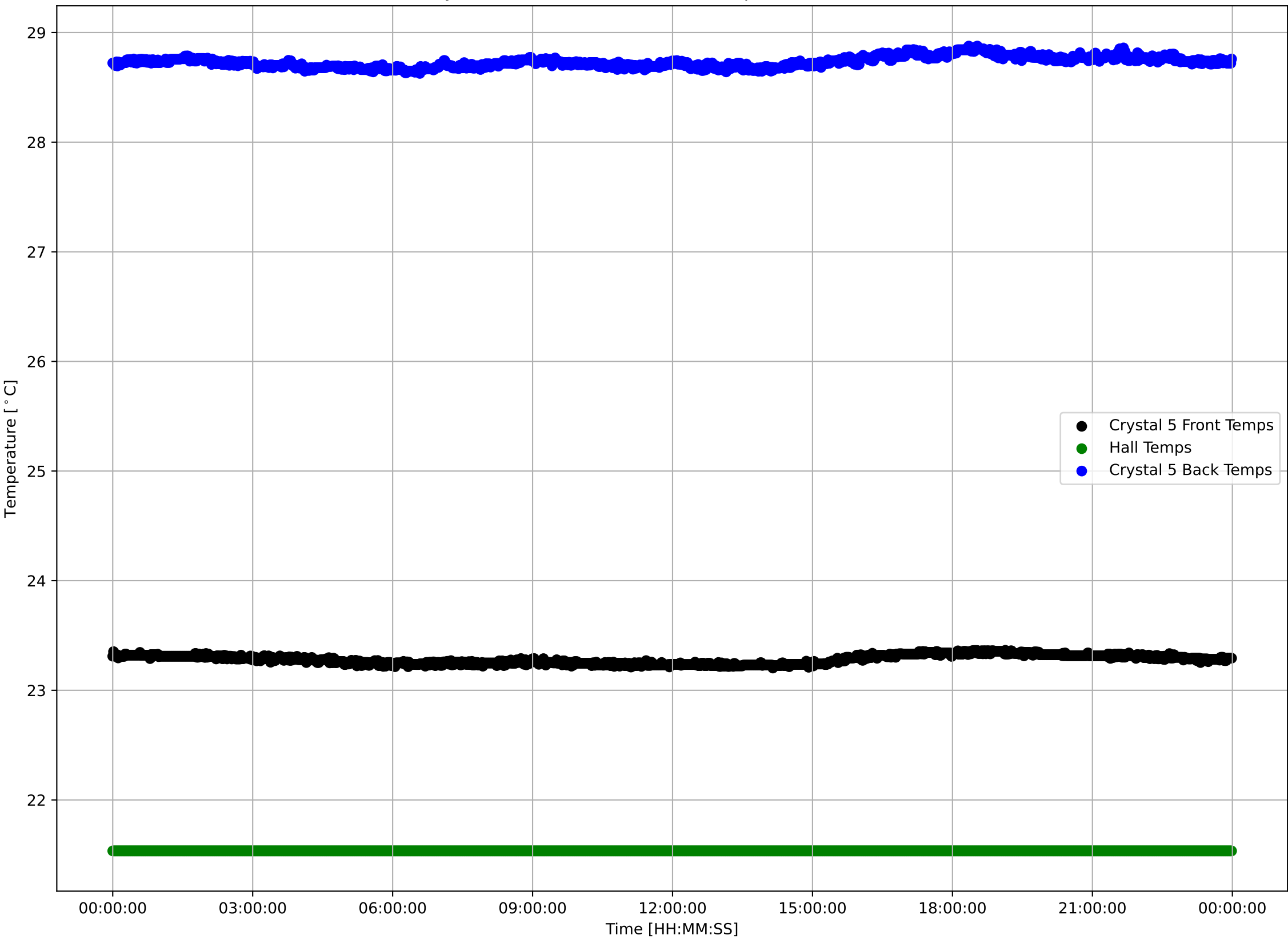
Crystal 5 Front, Back, and Hall Temps v Time - 240404
