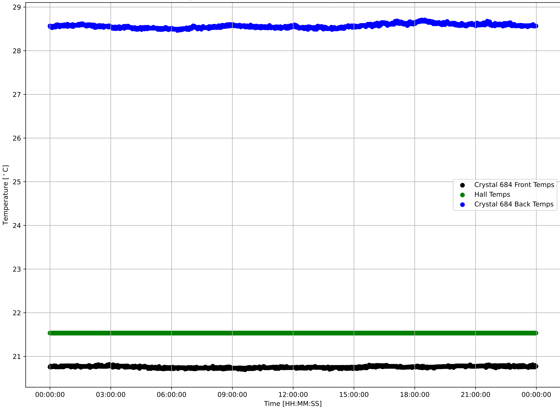
Crystal 684 Front, Back, and Hall Temps v Time - 240404
