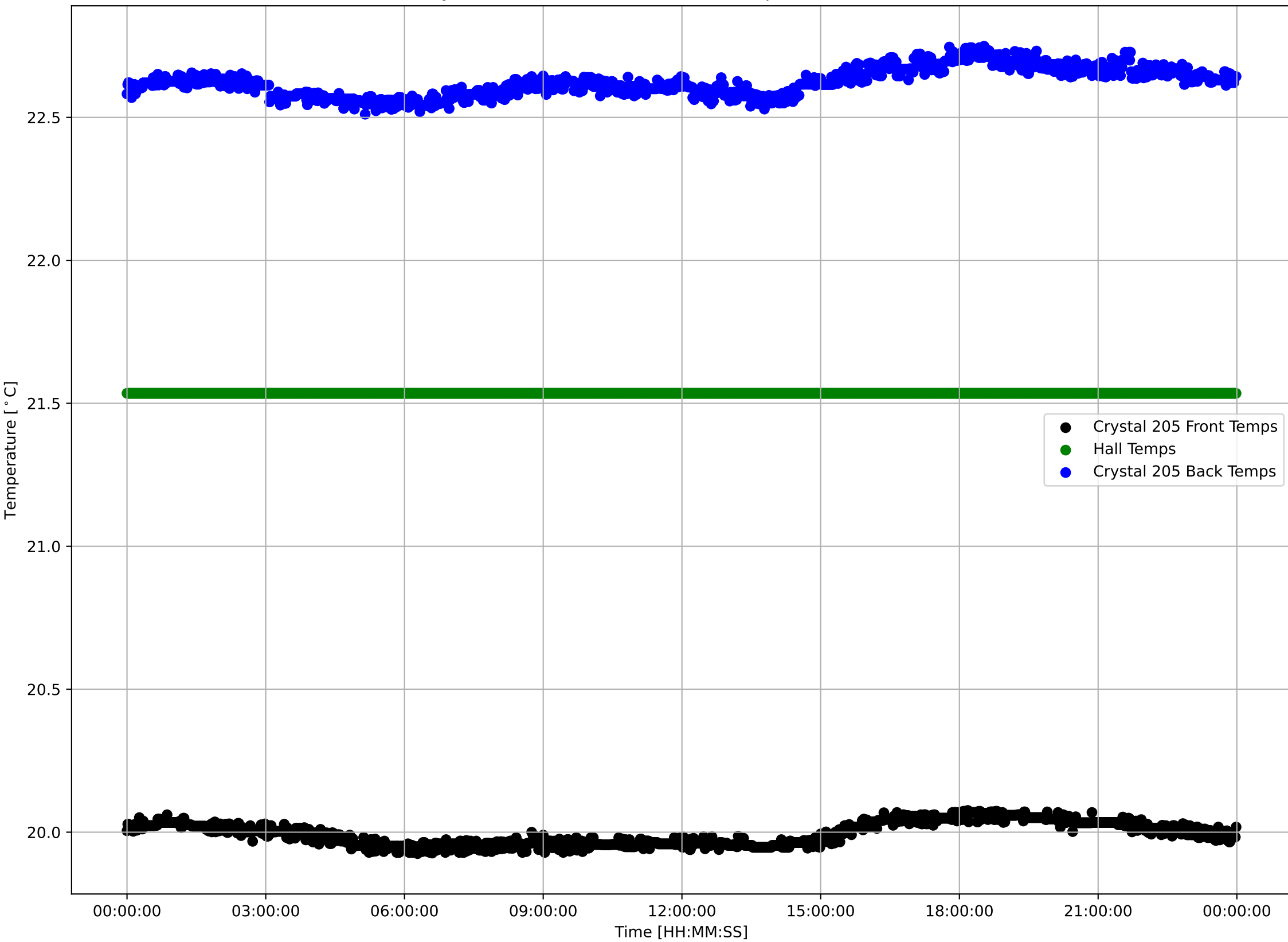
Crystal 205 Front, Back, and Hall Temps v Time - 240404
