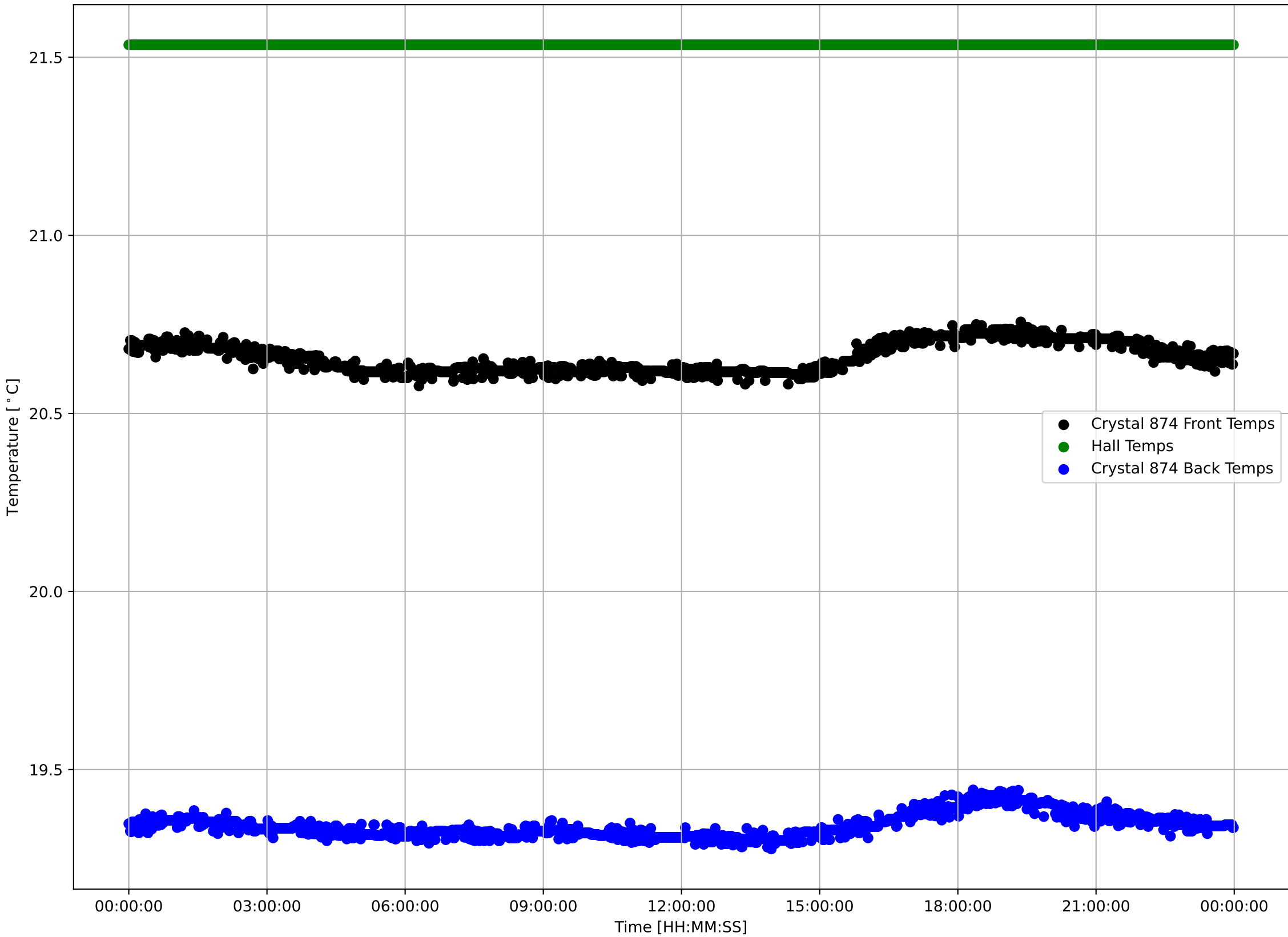
Crystal 874 Front, Back, and Hall Temps v Time - 240404
