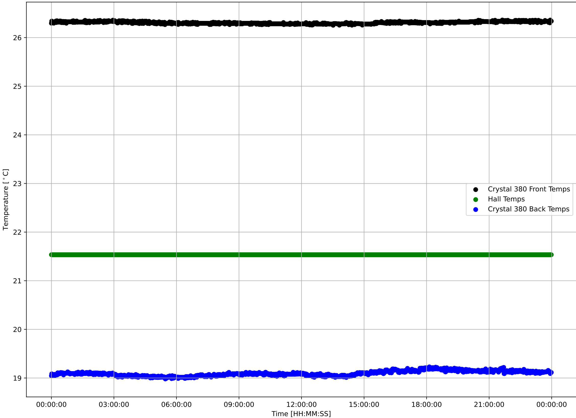
Crystal 380 Front, Back, and Hall Temps v Time - 240404
