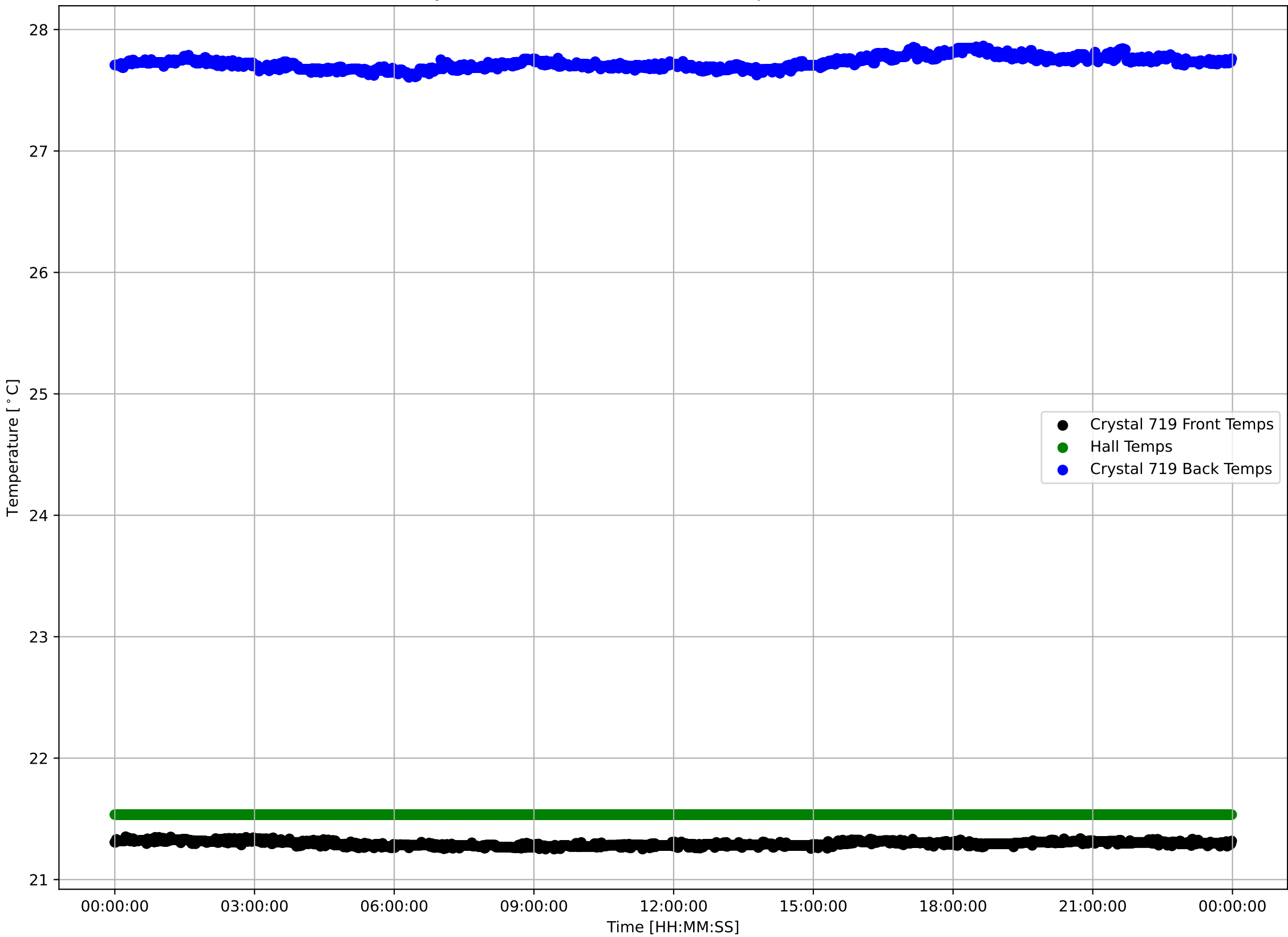
Crystal 719 Front, Back, and Hall Temps v Time - 240404
