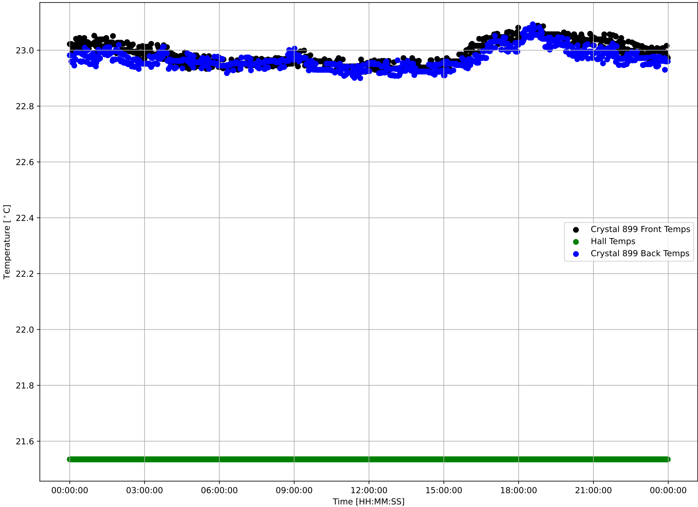
Crystal 899 Front, Back, and Hall Temps v Time - 240404
