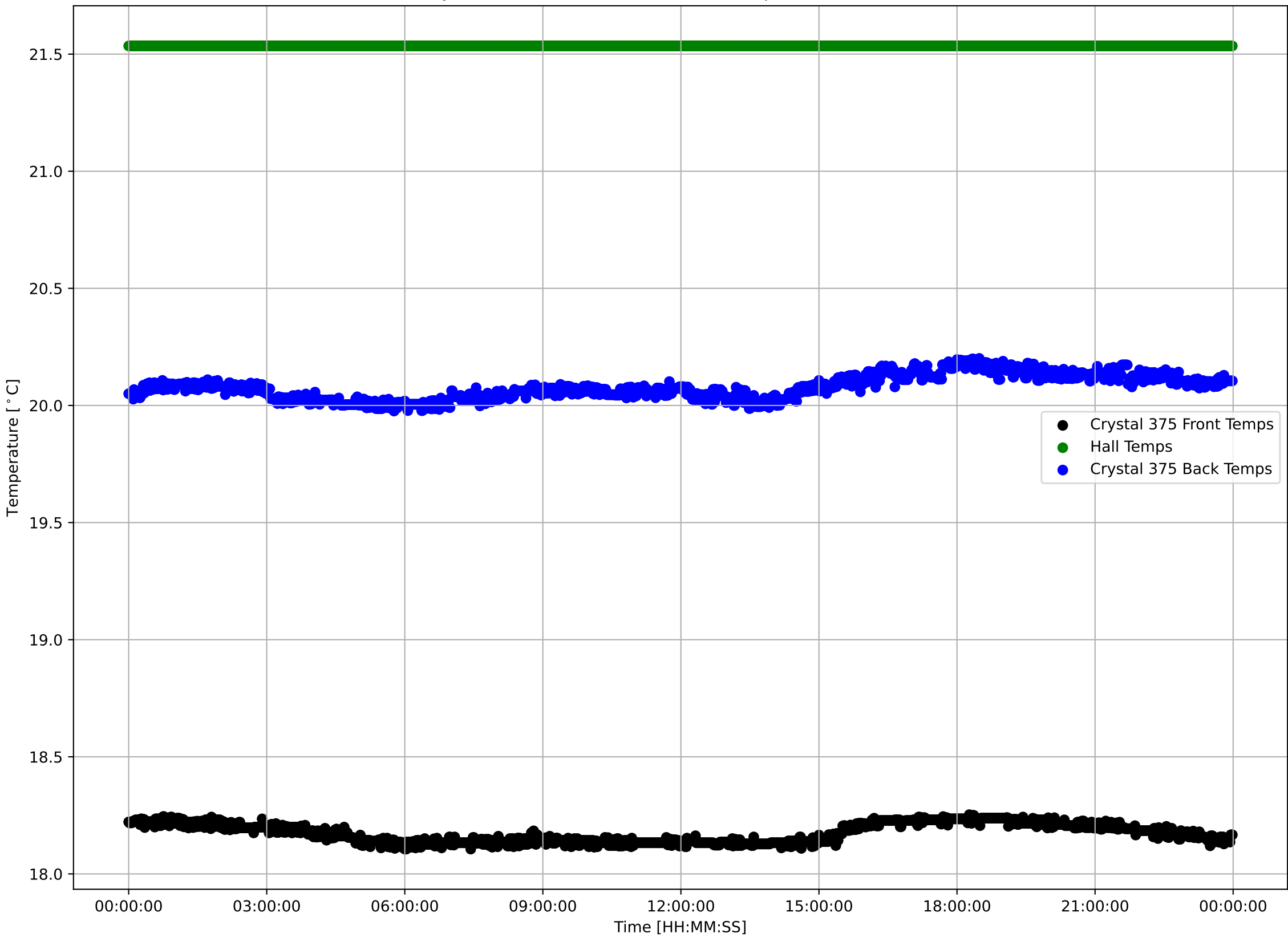
Crystal 375 Front, Back, and Hall Temps v Time - 240404
