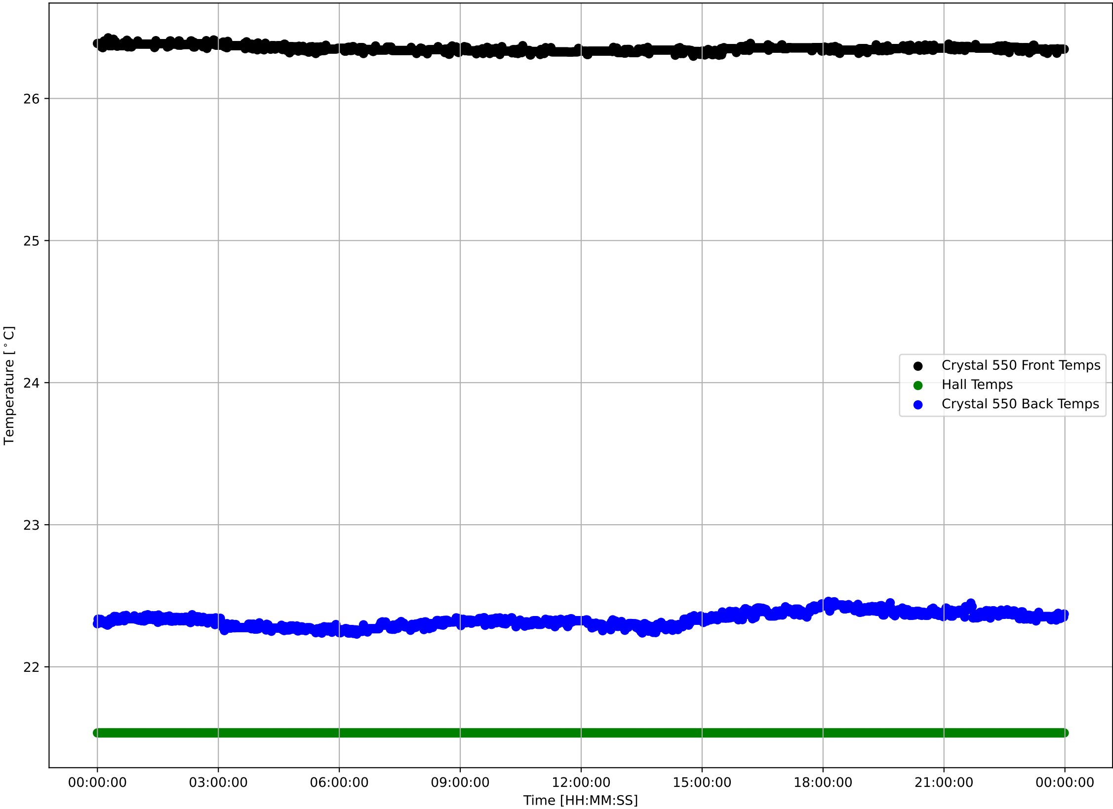
Crystal 550 Front, Back, and Hall Temps v Time - 240404
