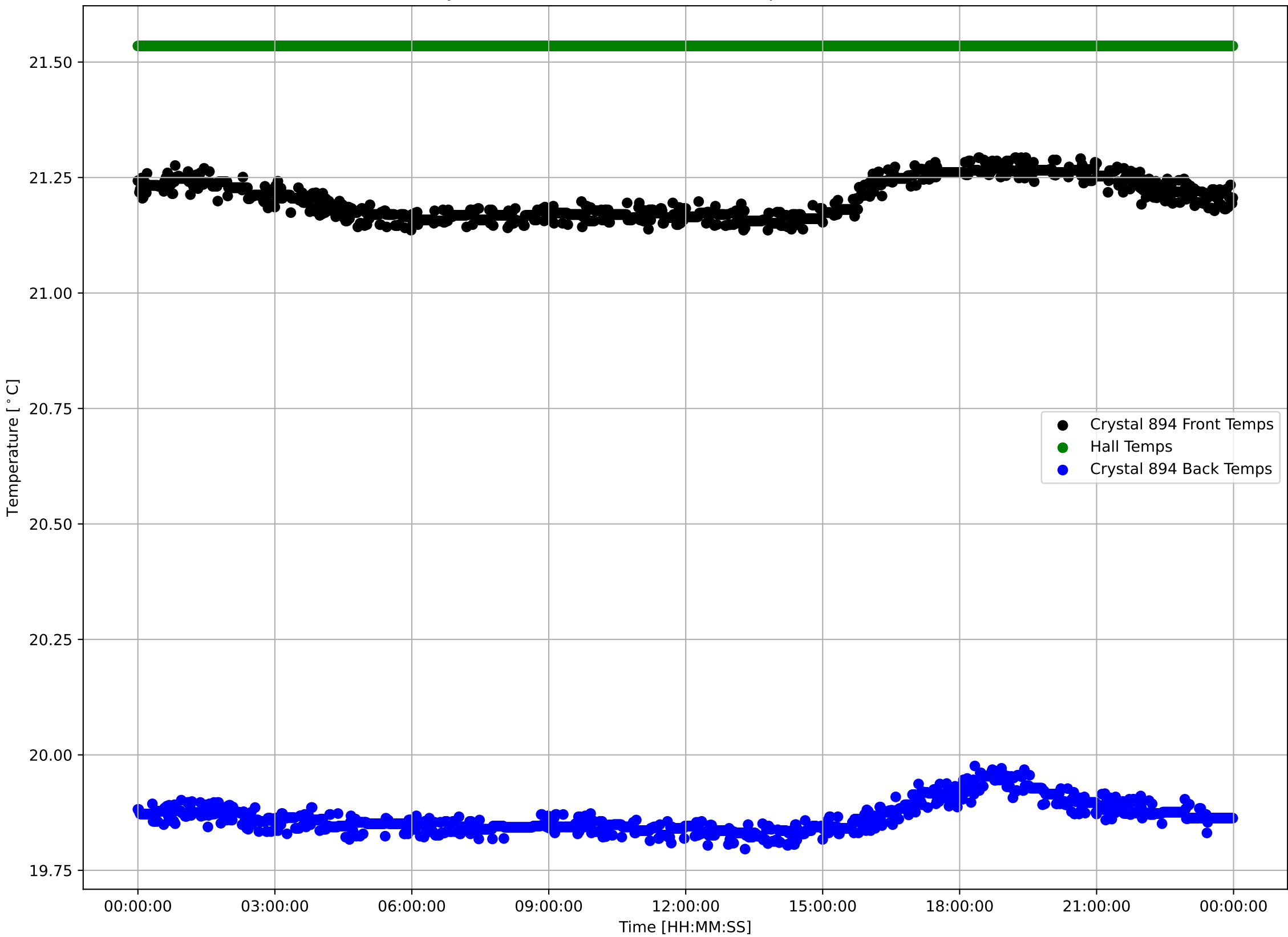
Crystal 894 Front, Back, and Hall Temps v Time - 240404
