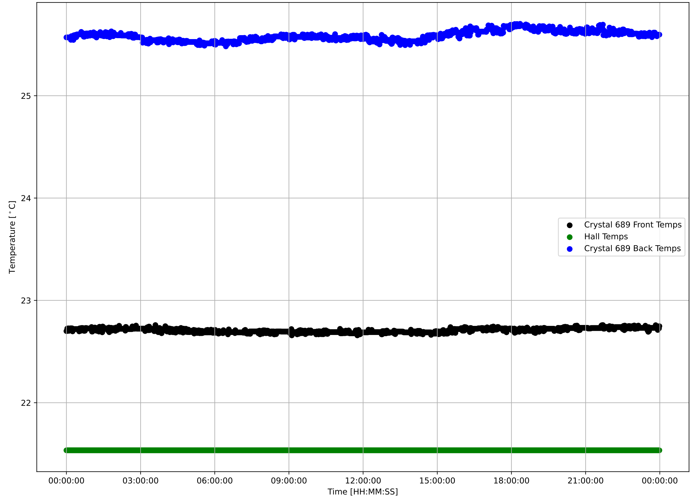
Crystal 689 Front, Back, and Hall Temps v Time - 240404
