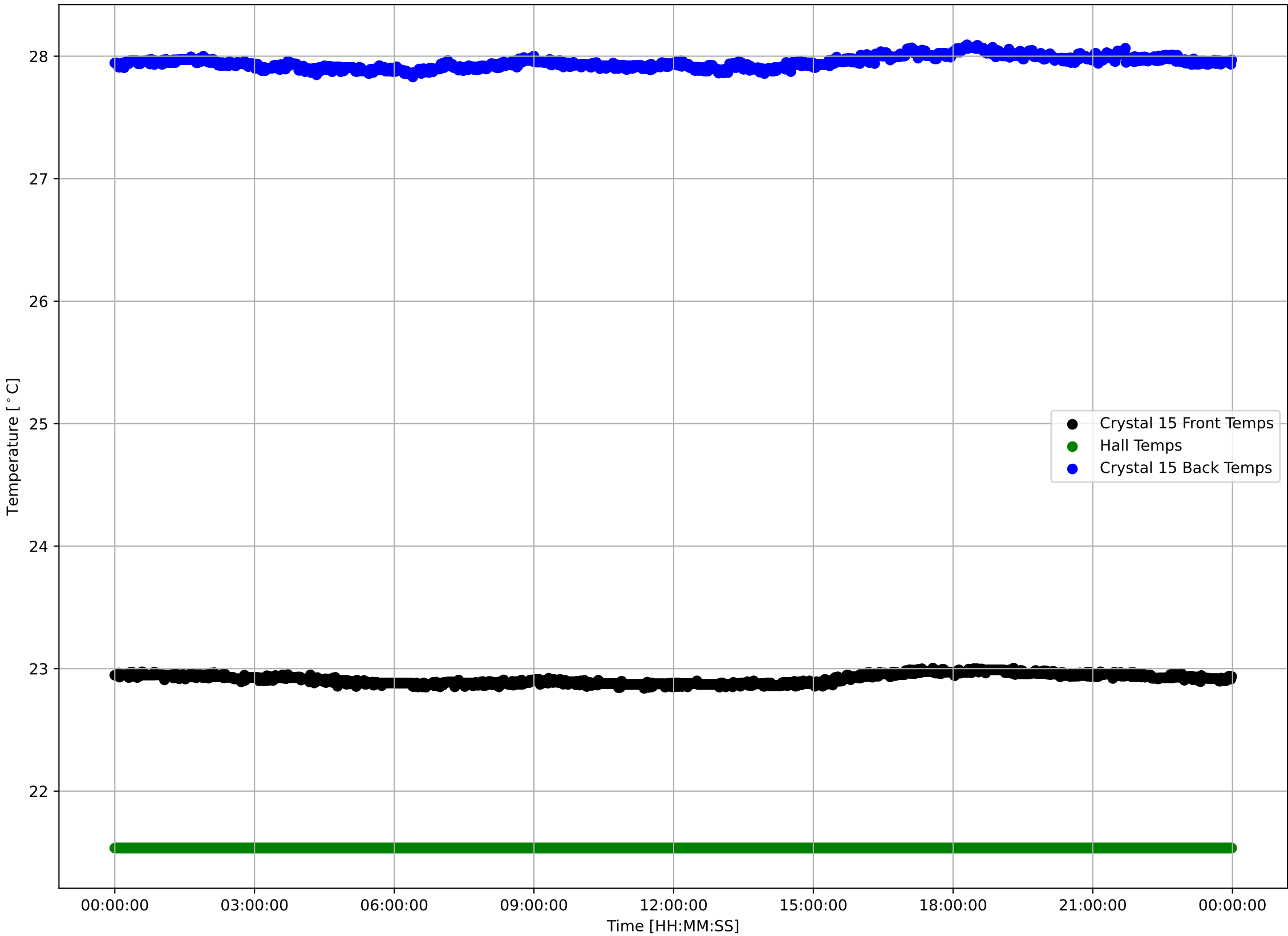
Crystal 15 Front, Back, and Hall Temps v Time - 240404
