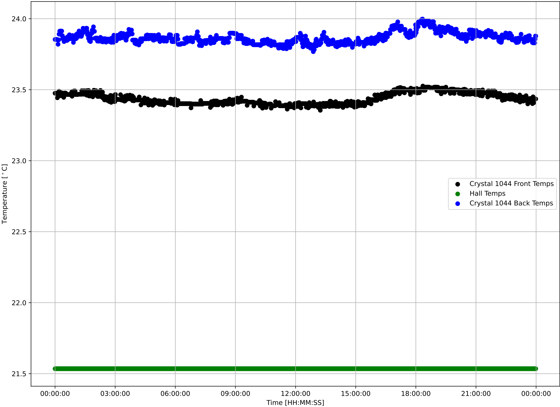
Crystal 1044 Front, Back, and Hall Temps v Time - 240404
