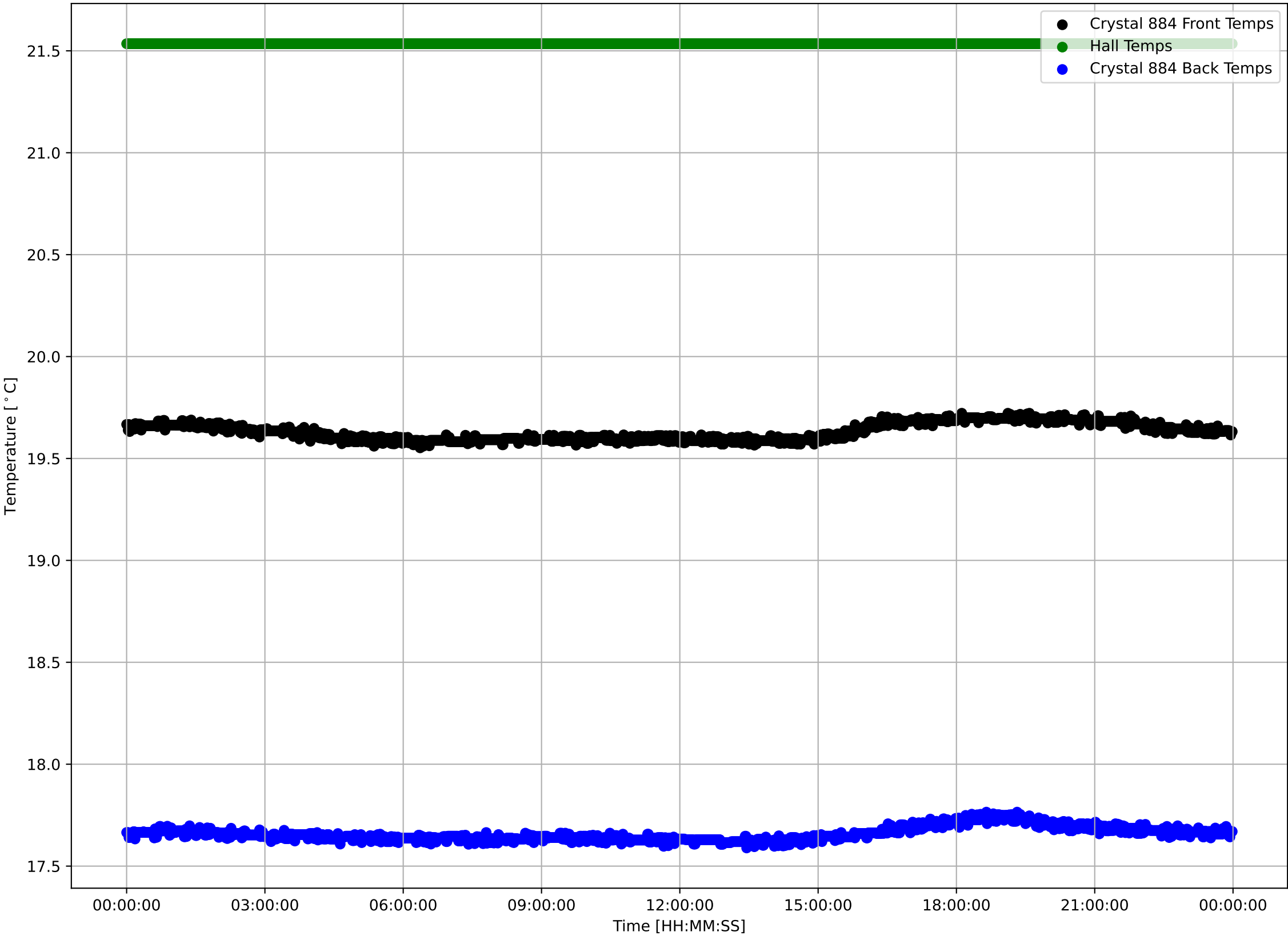
Crystal 884 Front, Back, and Hall Temps v Time - 240404
