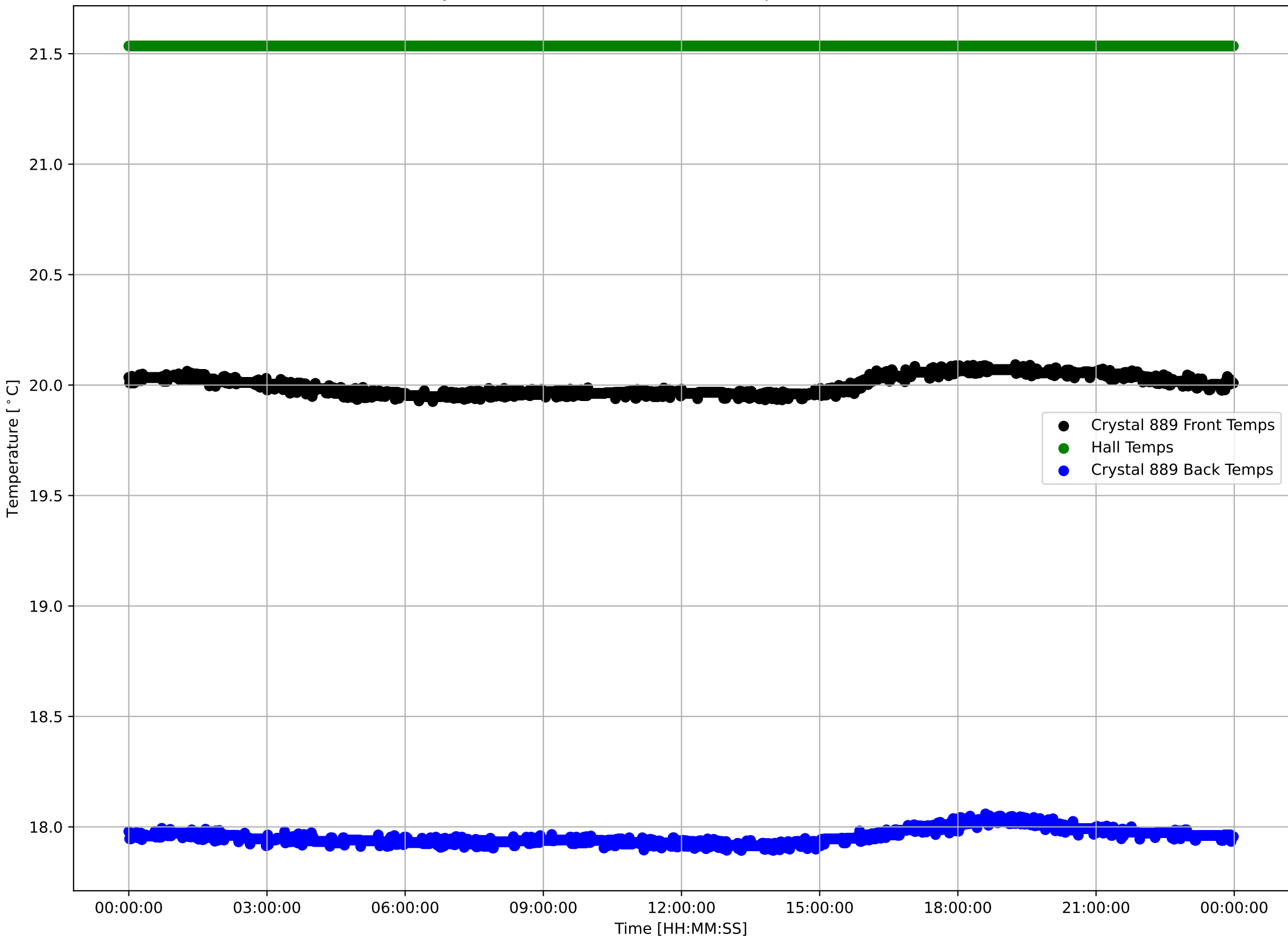
Crystal 889 Front, Back, and Hall Temps v Time - 240404
