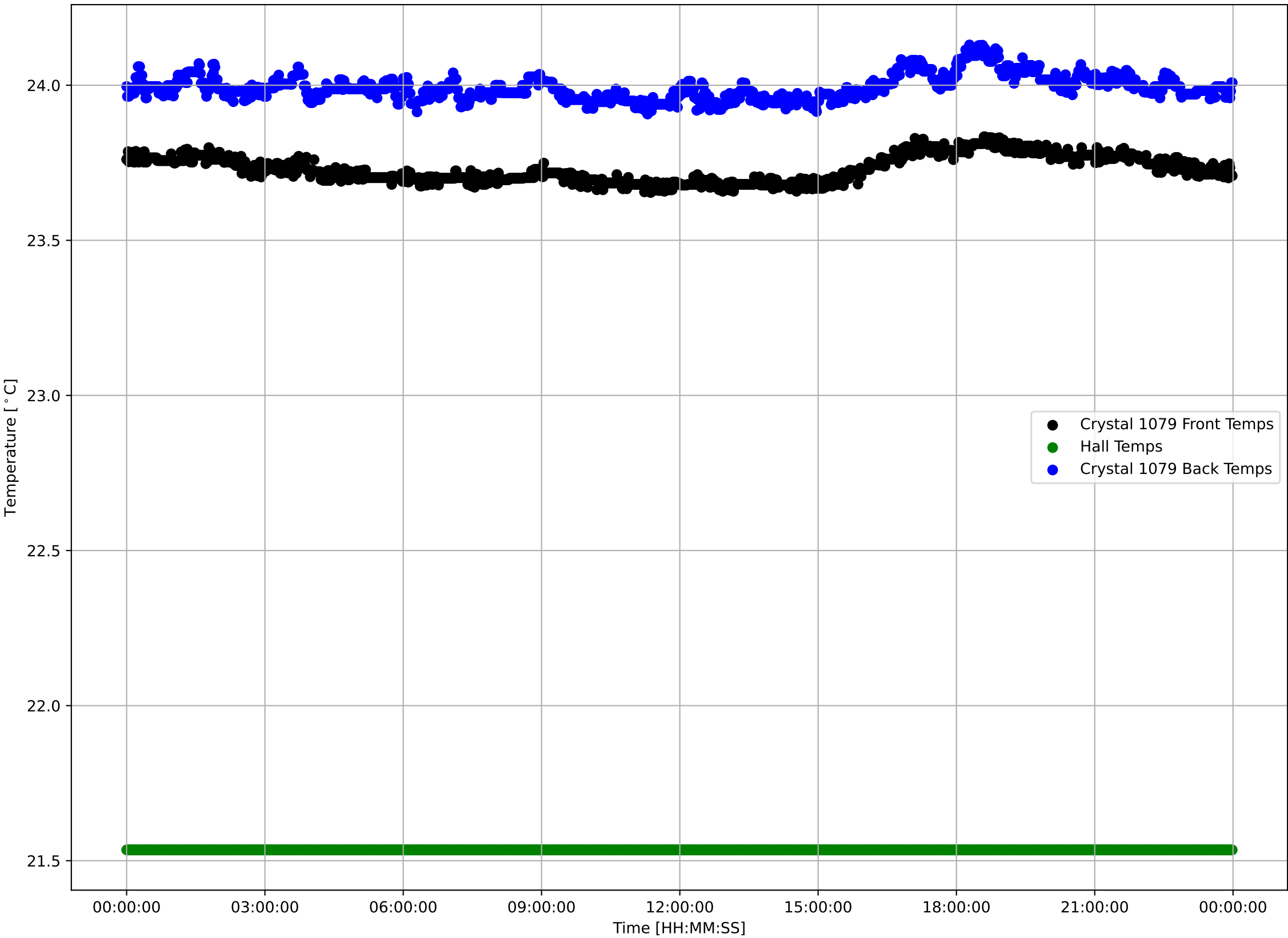
Crystal 1079 Front, Back, and Hall Temps v Time - 240404
