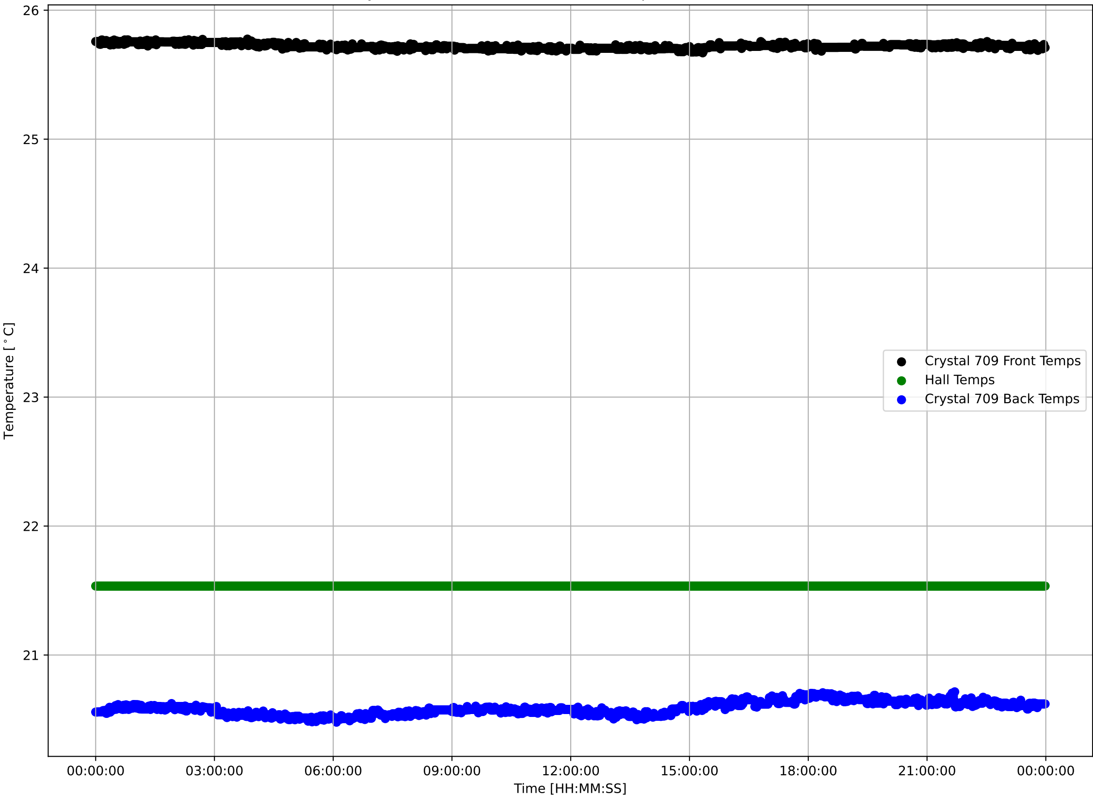
Crystal 709 Front, Back, and Hall Temps v Time - 240404
