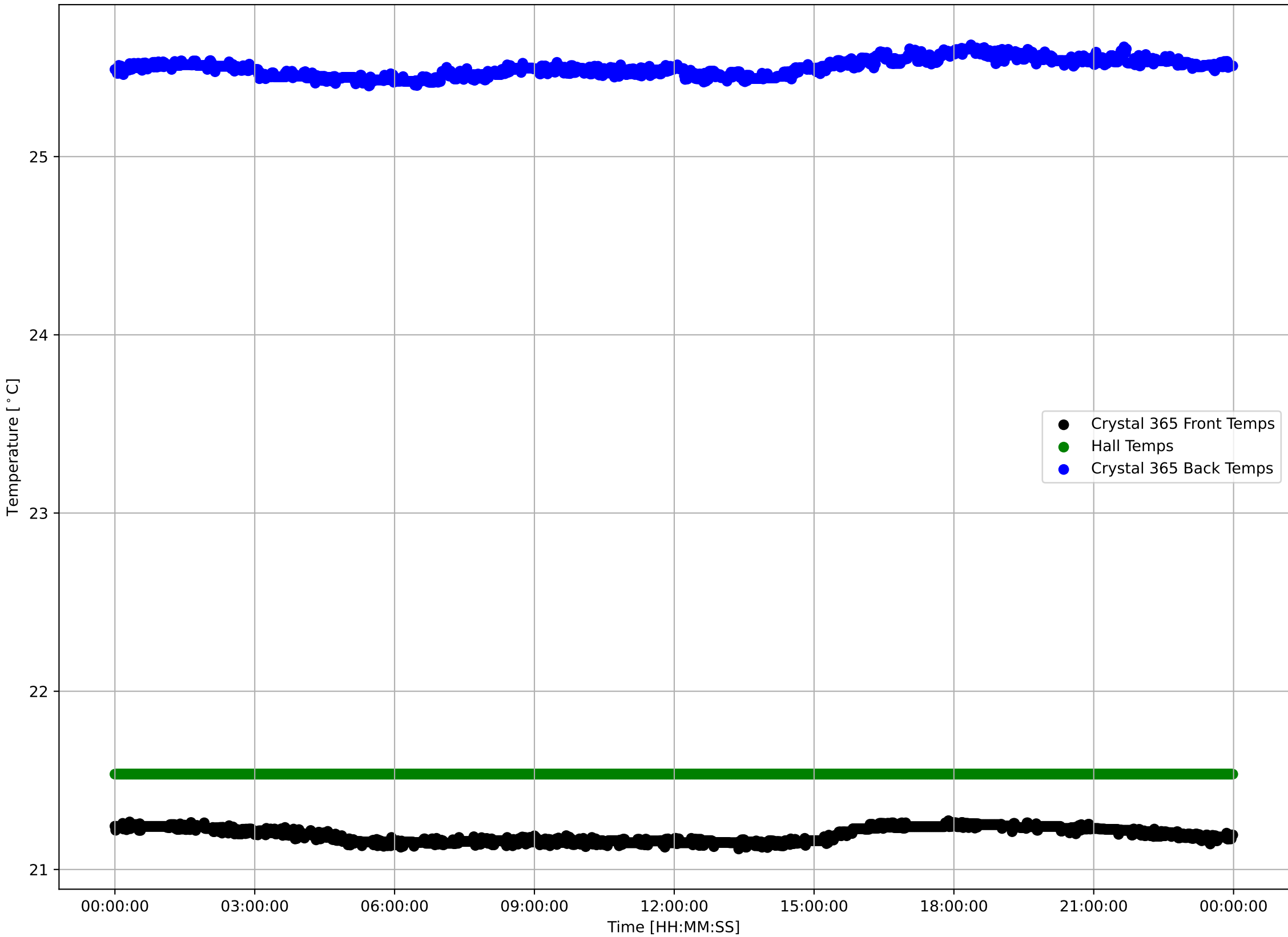
Crystal 365 Front, Back, and Hall Temps v Time - 240404
