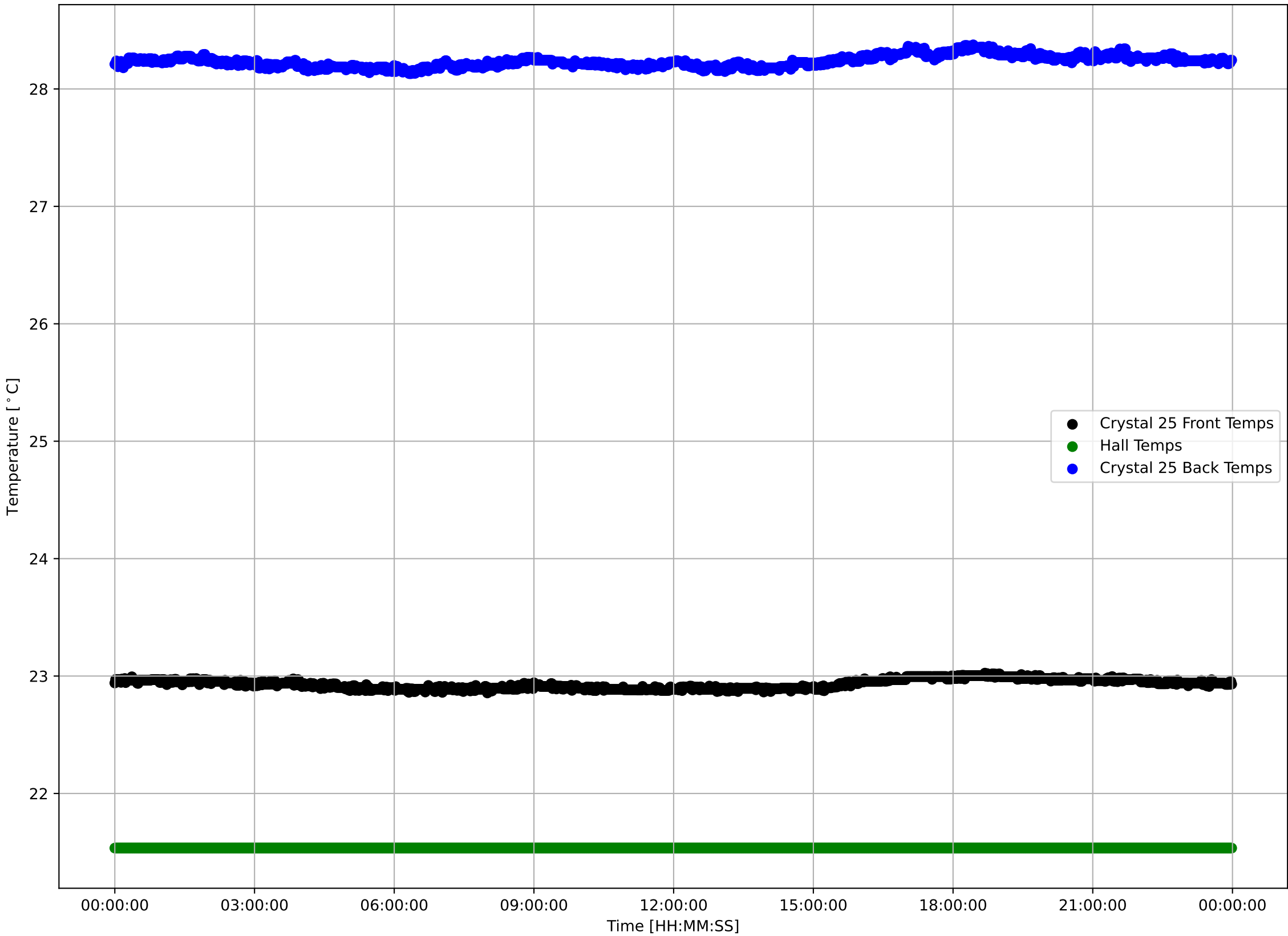
Crystal 25 Front, Back, and Hall Temps v Time - 240404
