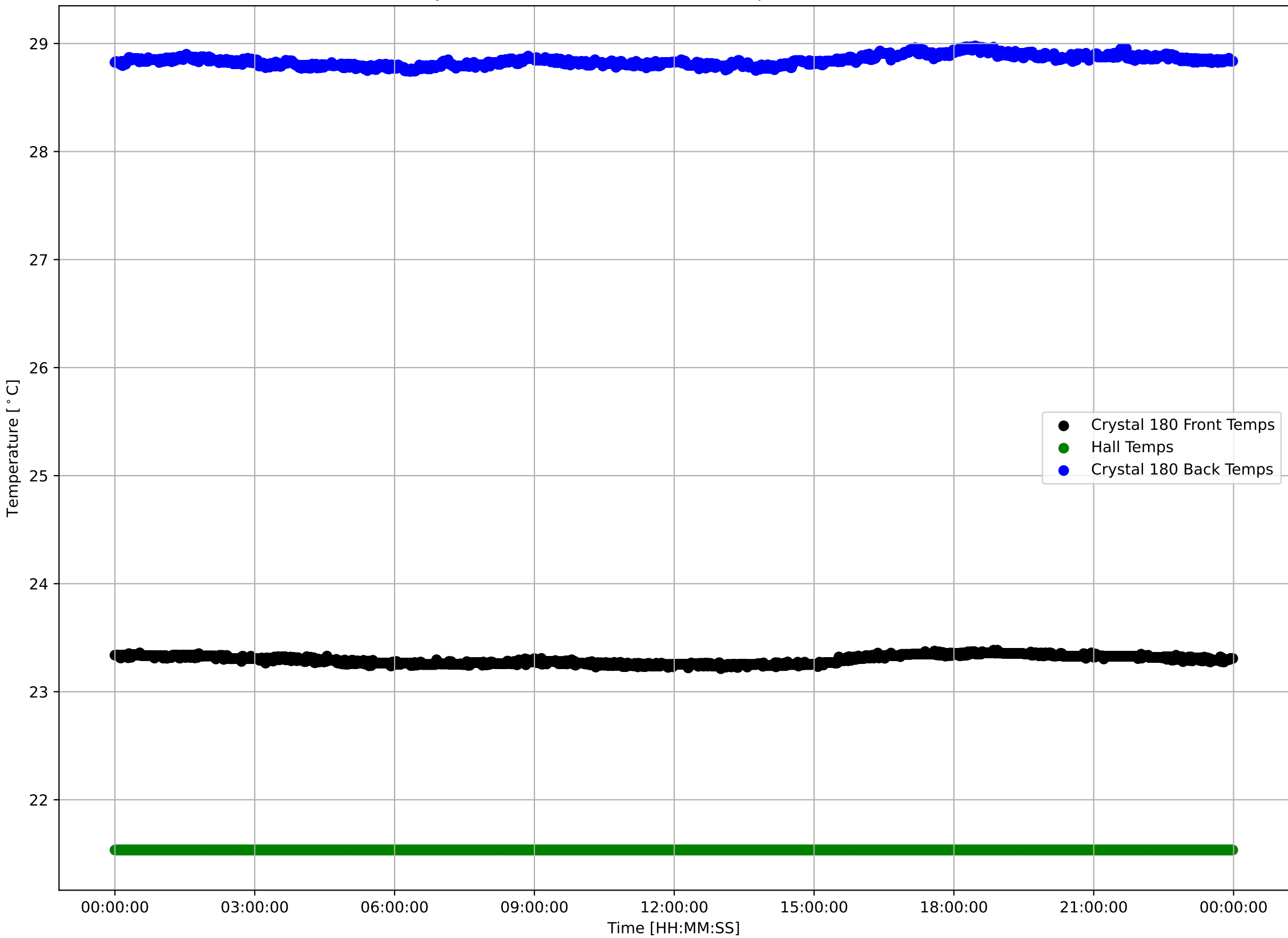
Crystal 180 Front, Back, and Hall Temps v Time - 240404
