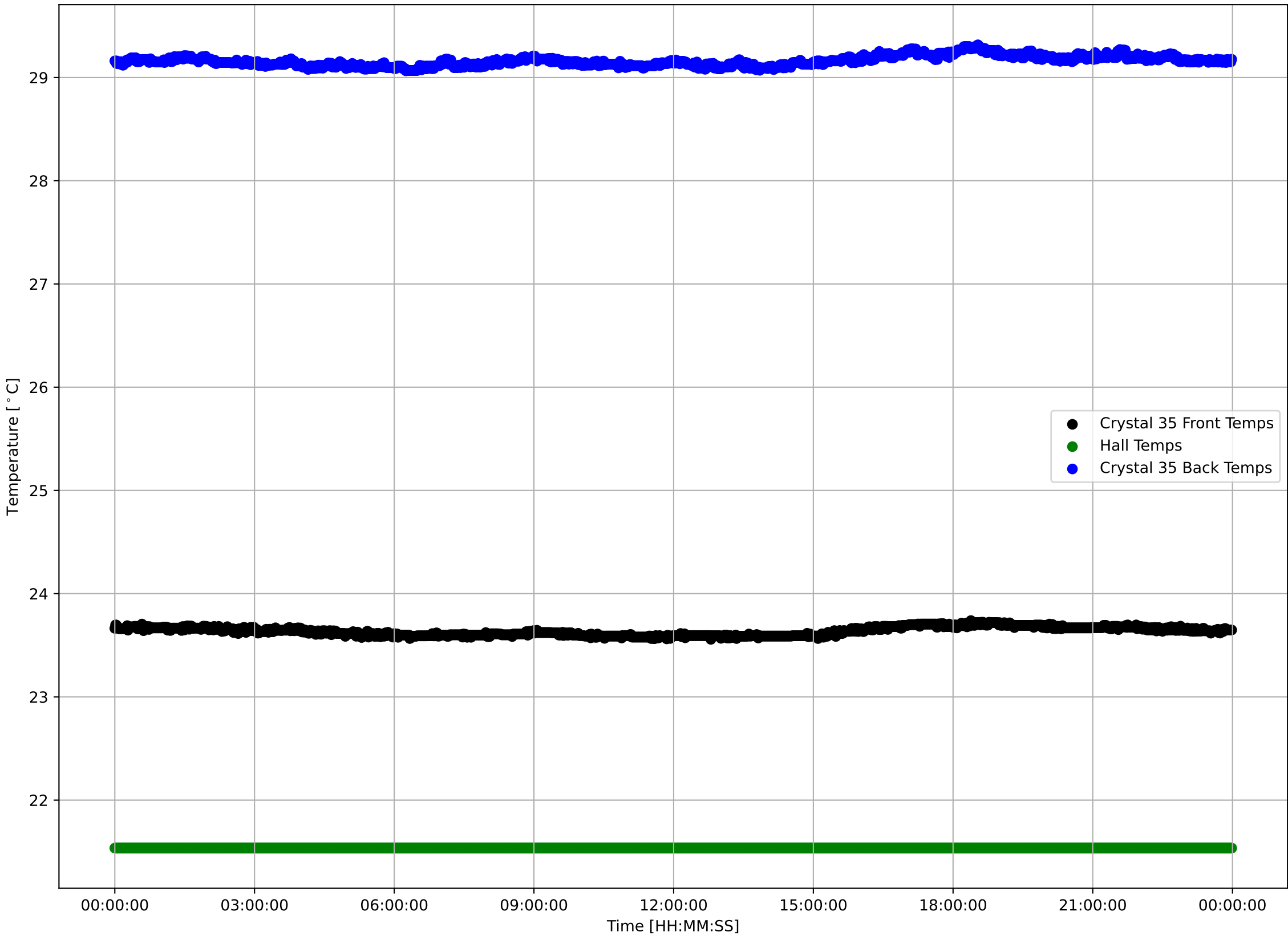
Crystal 35 Front, Back, and Hall Temps v Time - 240404
