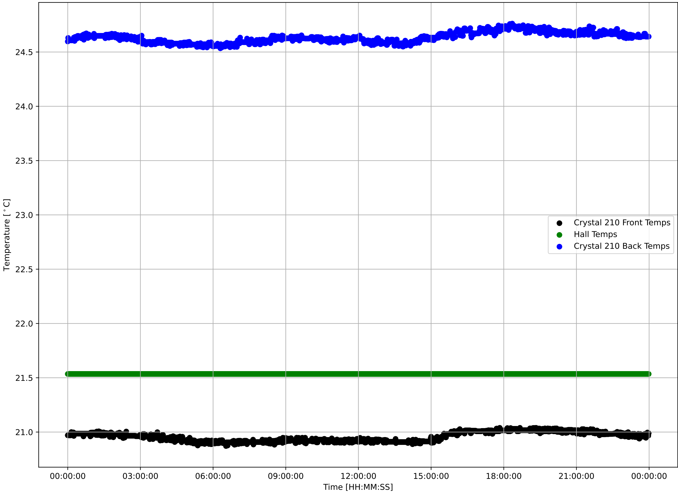
Crystal 210 Front, Back, and Hall Temps v Time - 240404
