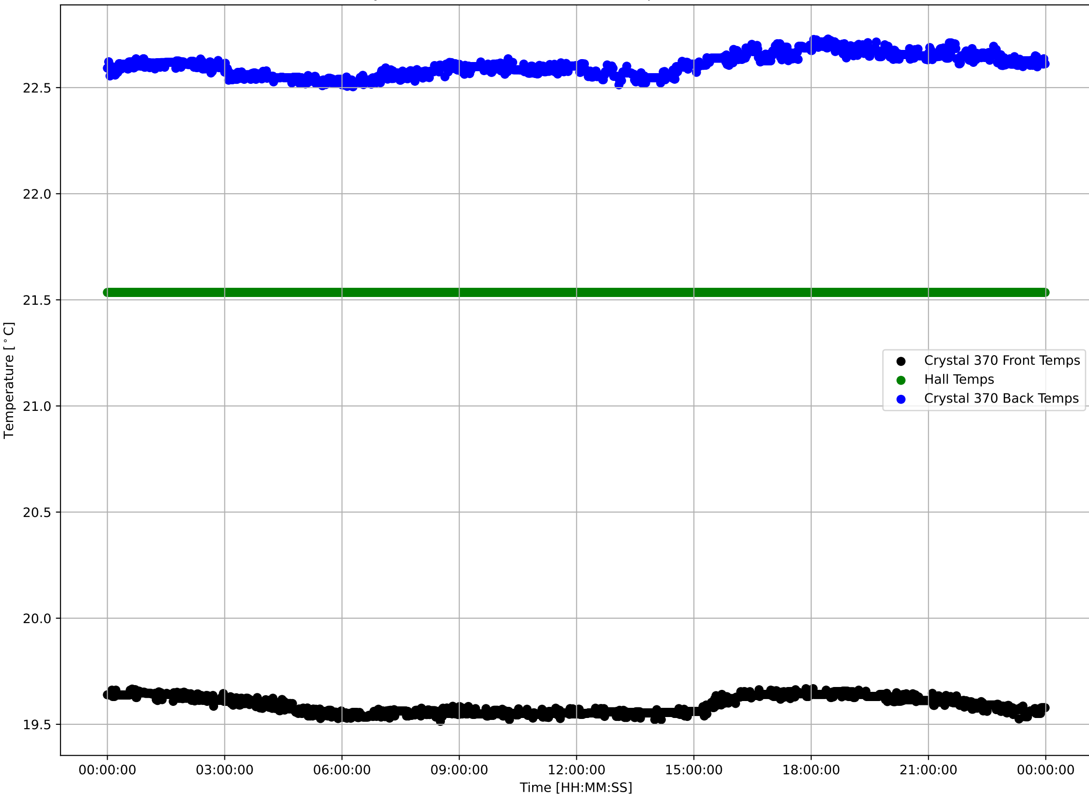
Crystal 370 Front, Back, and Hall Temps v Time - 240404
